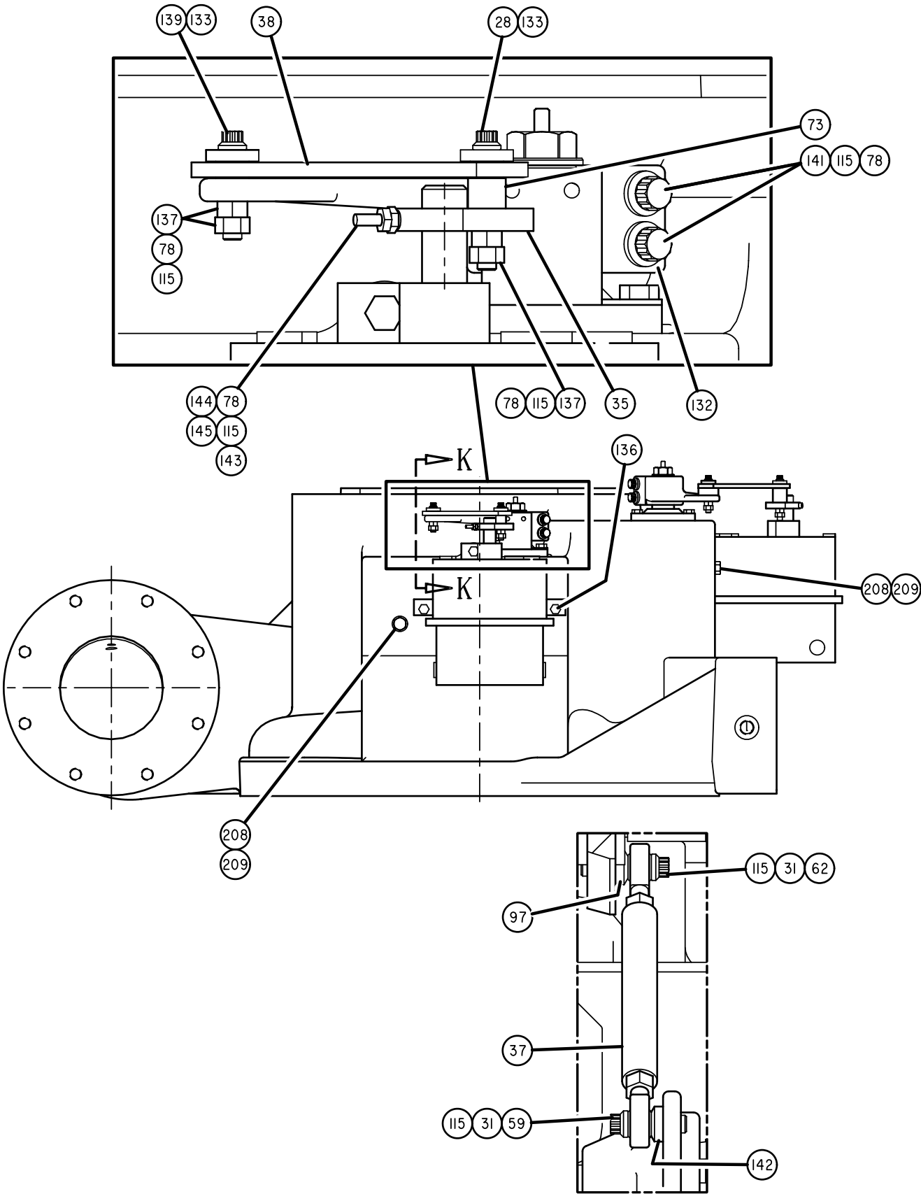
FIG. 23 – HE COMPRESSOR (70)
