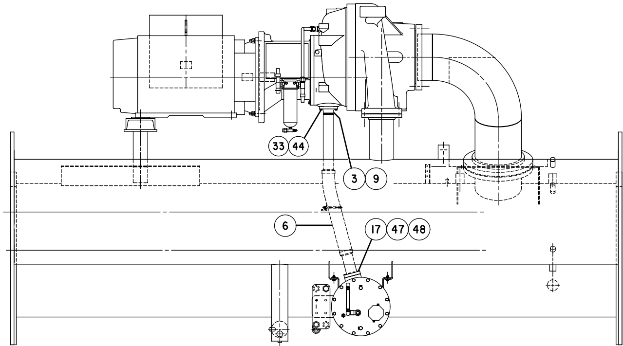
FIG. 57 - OIL RETURN LINE
