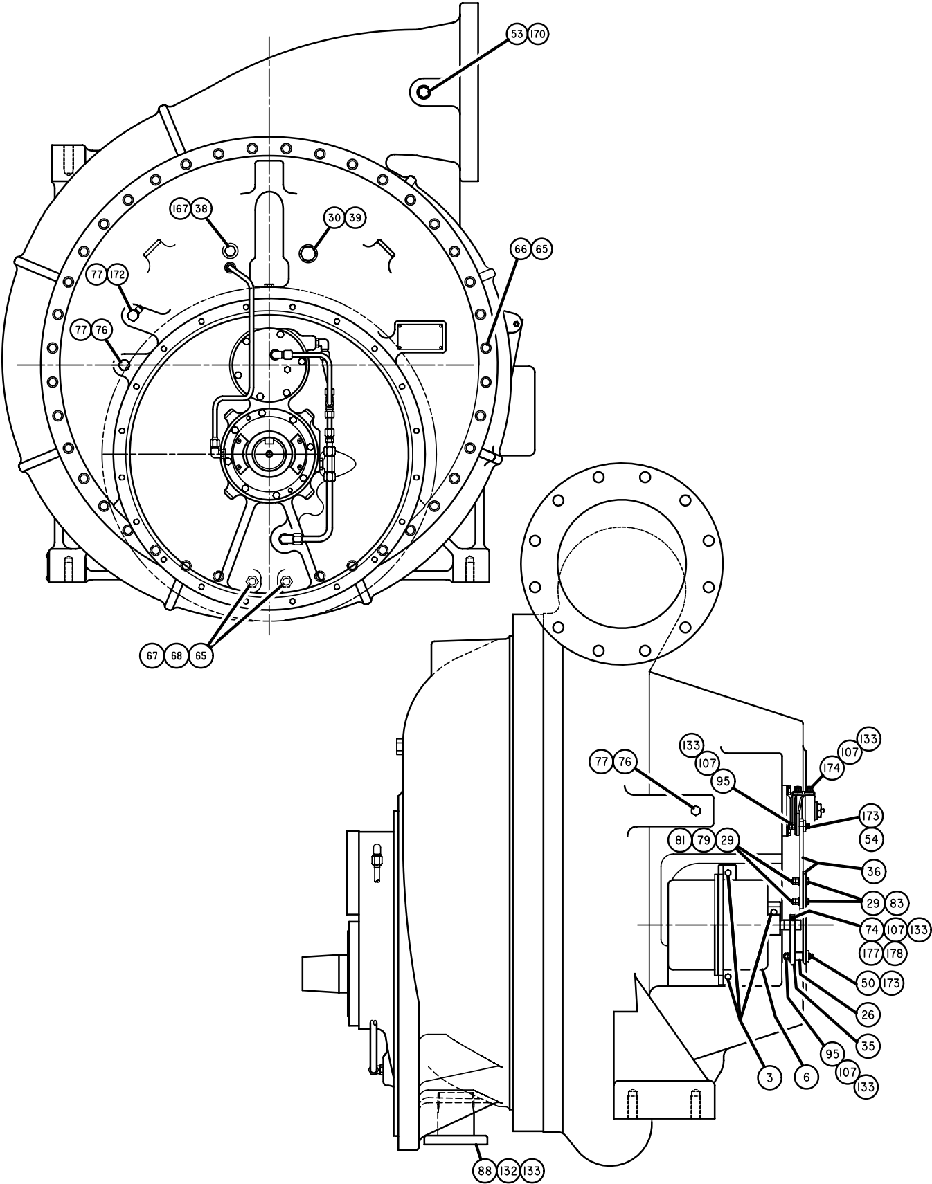
FIG. 39 – HG COMPRESSOR (81, 90)
