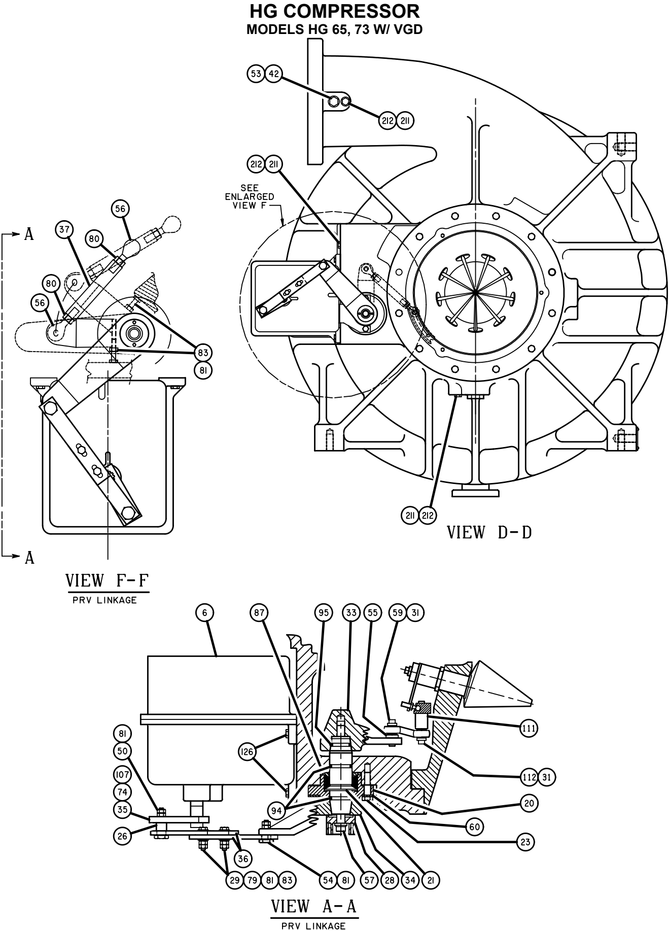
FIG. 33 – HG COMPRESSOR (65, 73)
