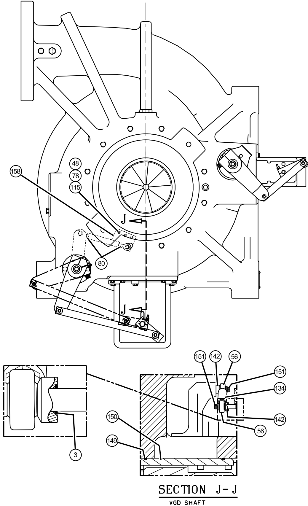
FIG. 34 – HG COMPRESSOR (HG 65, 73)
