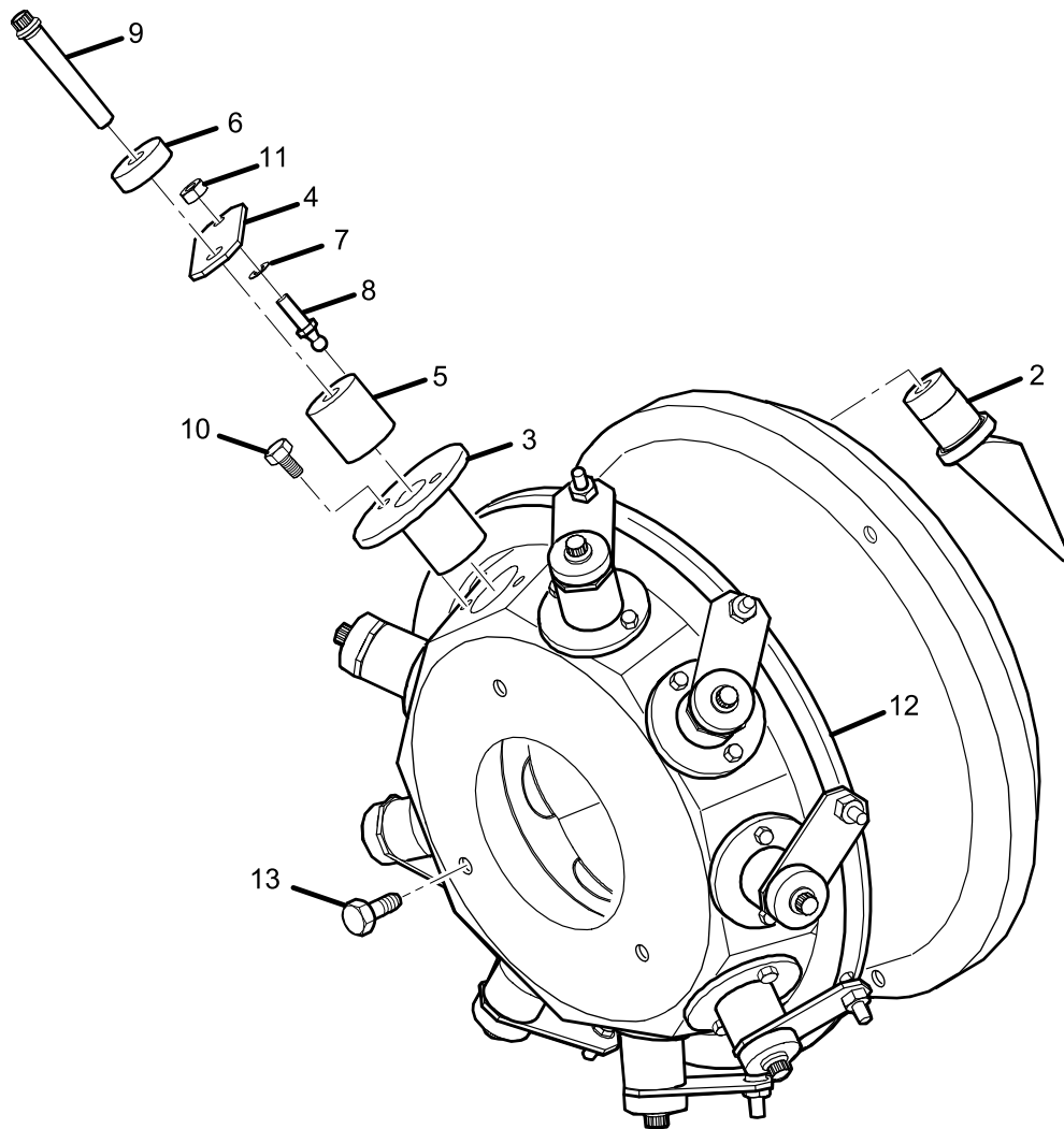
FIG. 4 – DEVICE PRE-ROTATION (HA 41)
