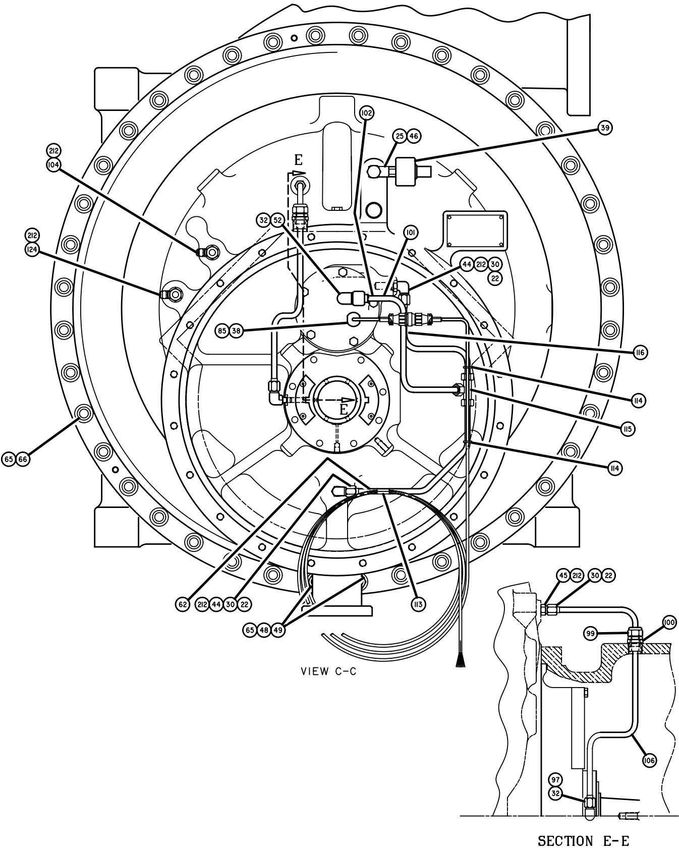
FIG. 32 – HG COMPRESSOR (65, 73)
