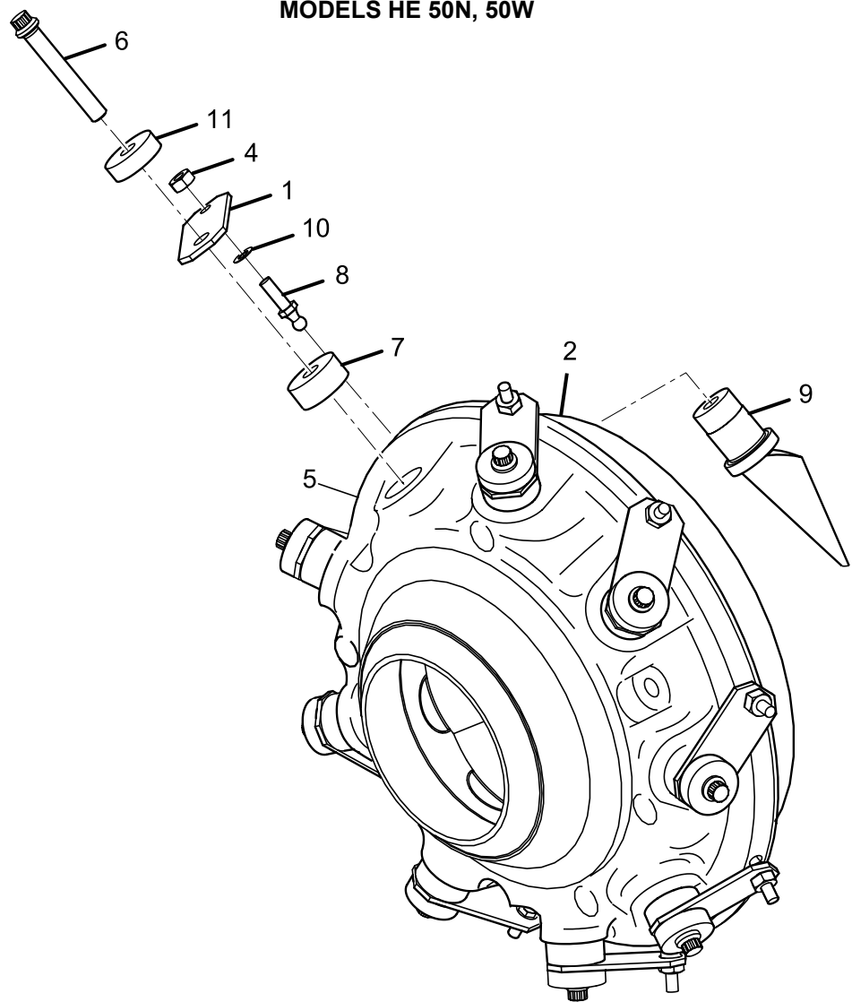
FIG. 13– DEVICE PRE-ROTATION (50N, 50W)
