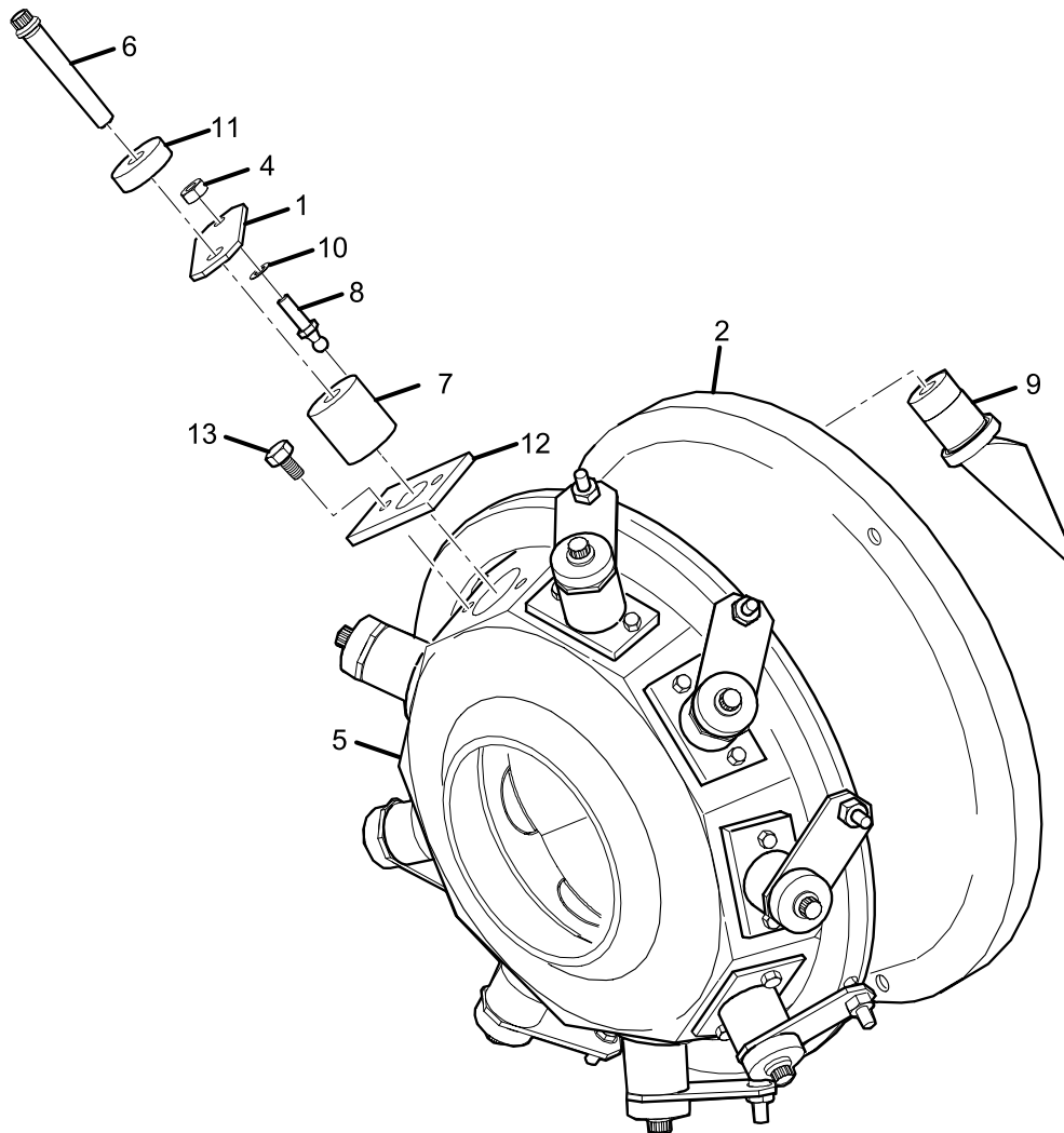
FIG. 8– DEVICE PRE-ROTATION (HB 61)
