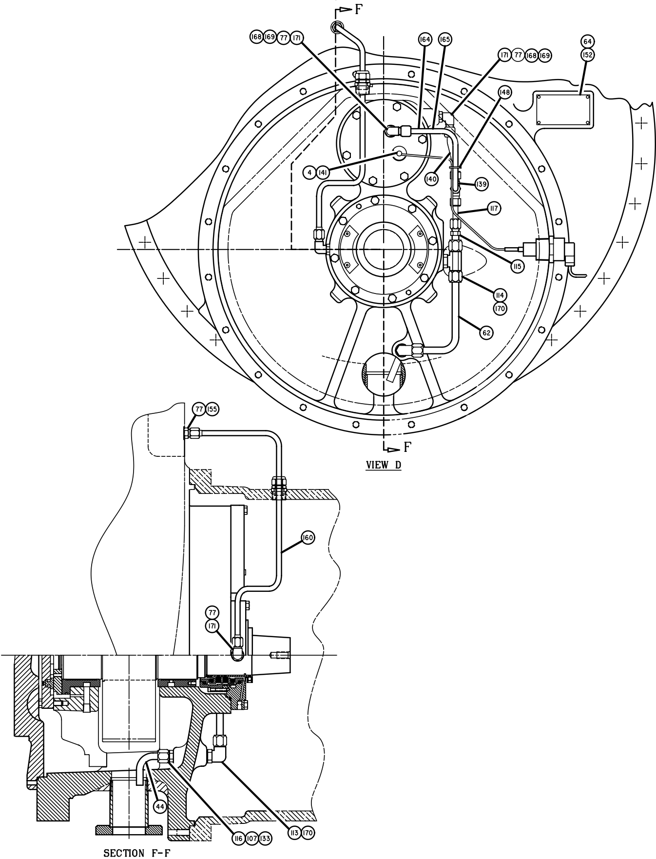
FIG. 41 – HG COMPRESSOR (81, 90)
