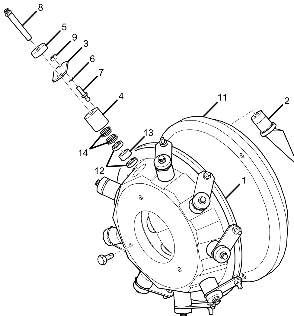
FIG. 55– DEVICE PRE-ROTATION (HA 119)
