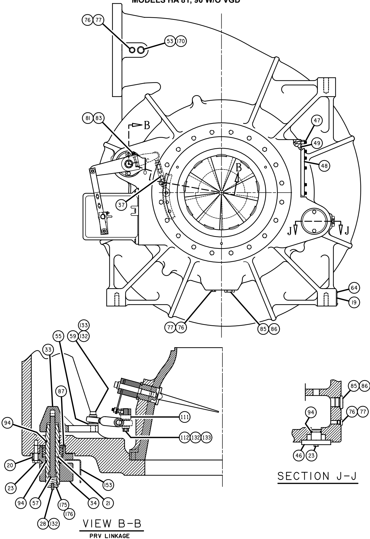
FIG. 40 – HG COMPRESSOR (81, 90)
