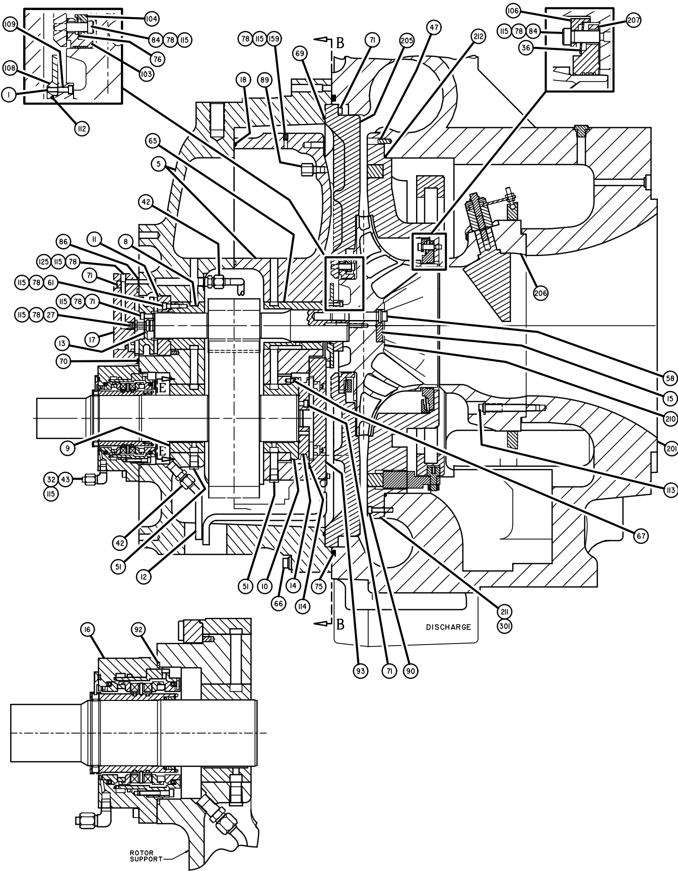
FIG. 19 – HE COMPRESSOR (70)
