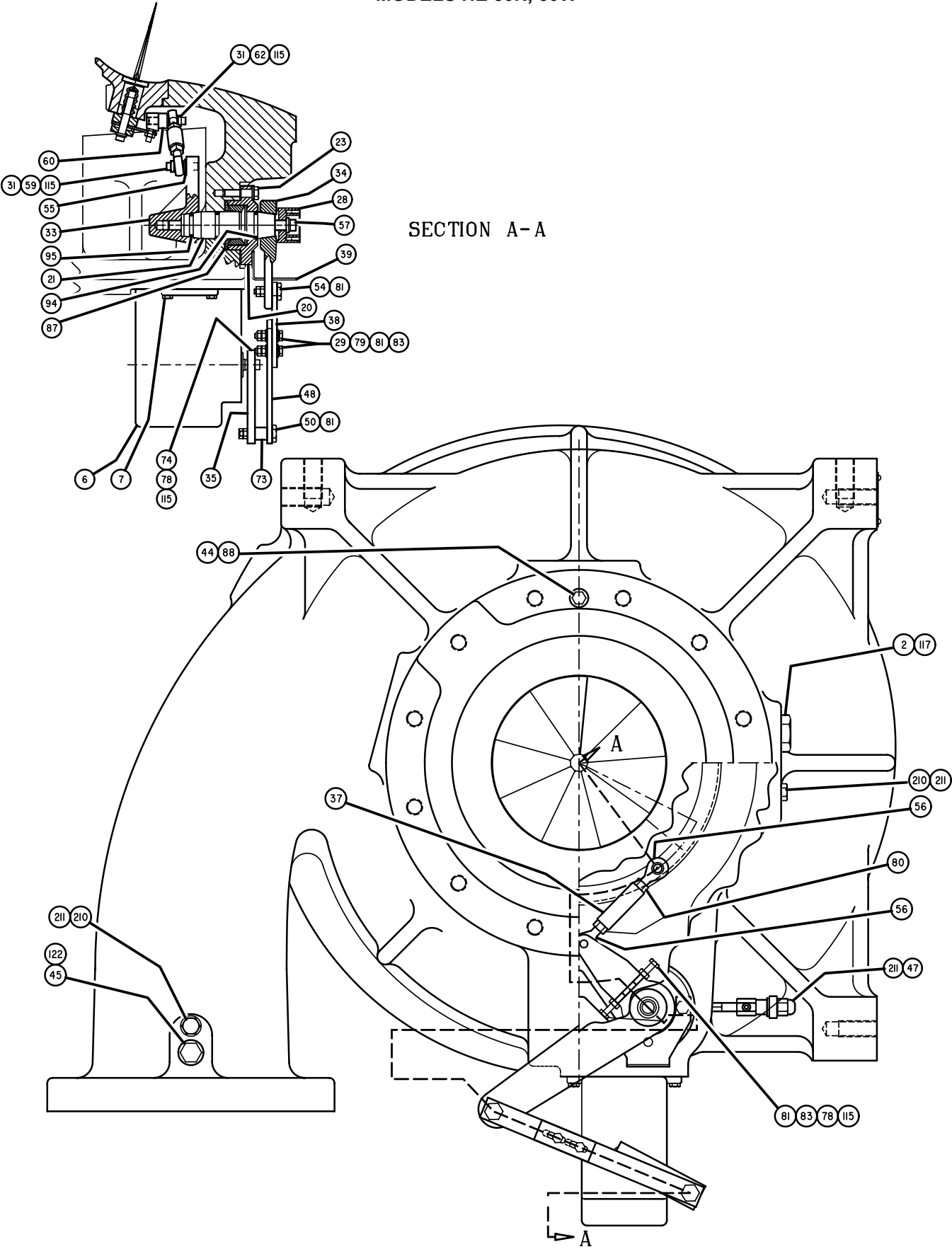
FIG. 12 – HE COMPRESSOR (50N, 50W)
