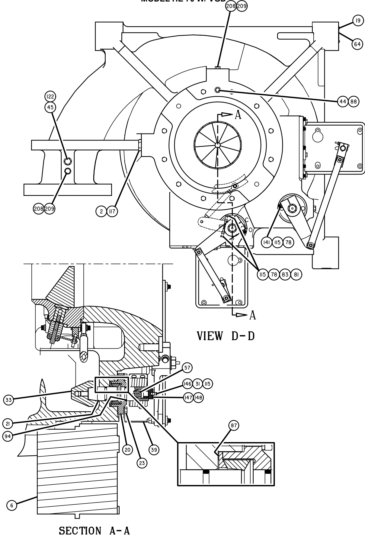
FIG. 22 – HE COMPRESSOR (70)
