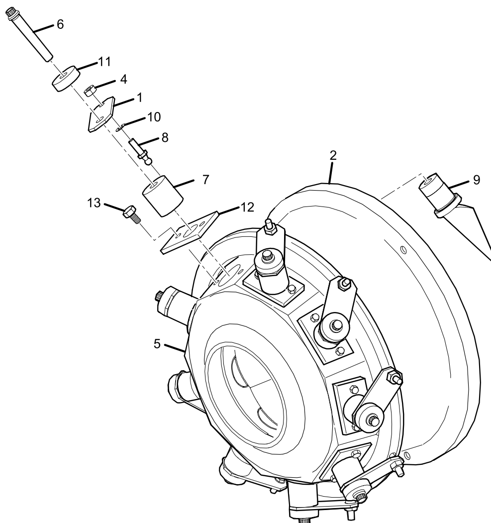
FIG. 42– DEVICE PRE-ROTATION (HA 81, 90)
