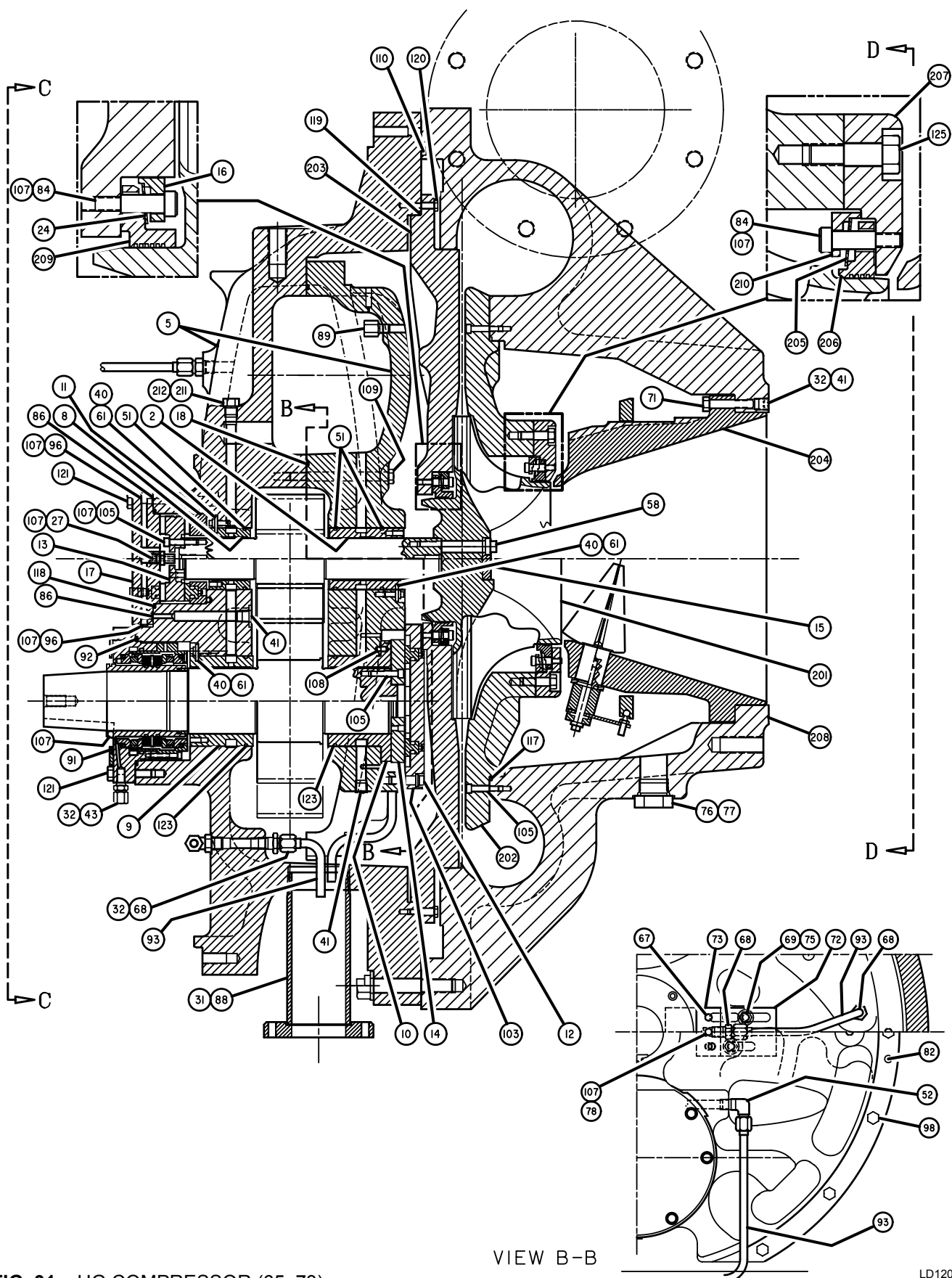
FIG. 31 – HG COMPRESSOR (65, 73)
