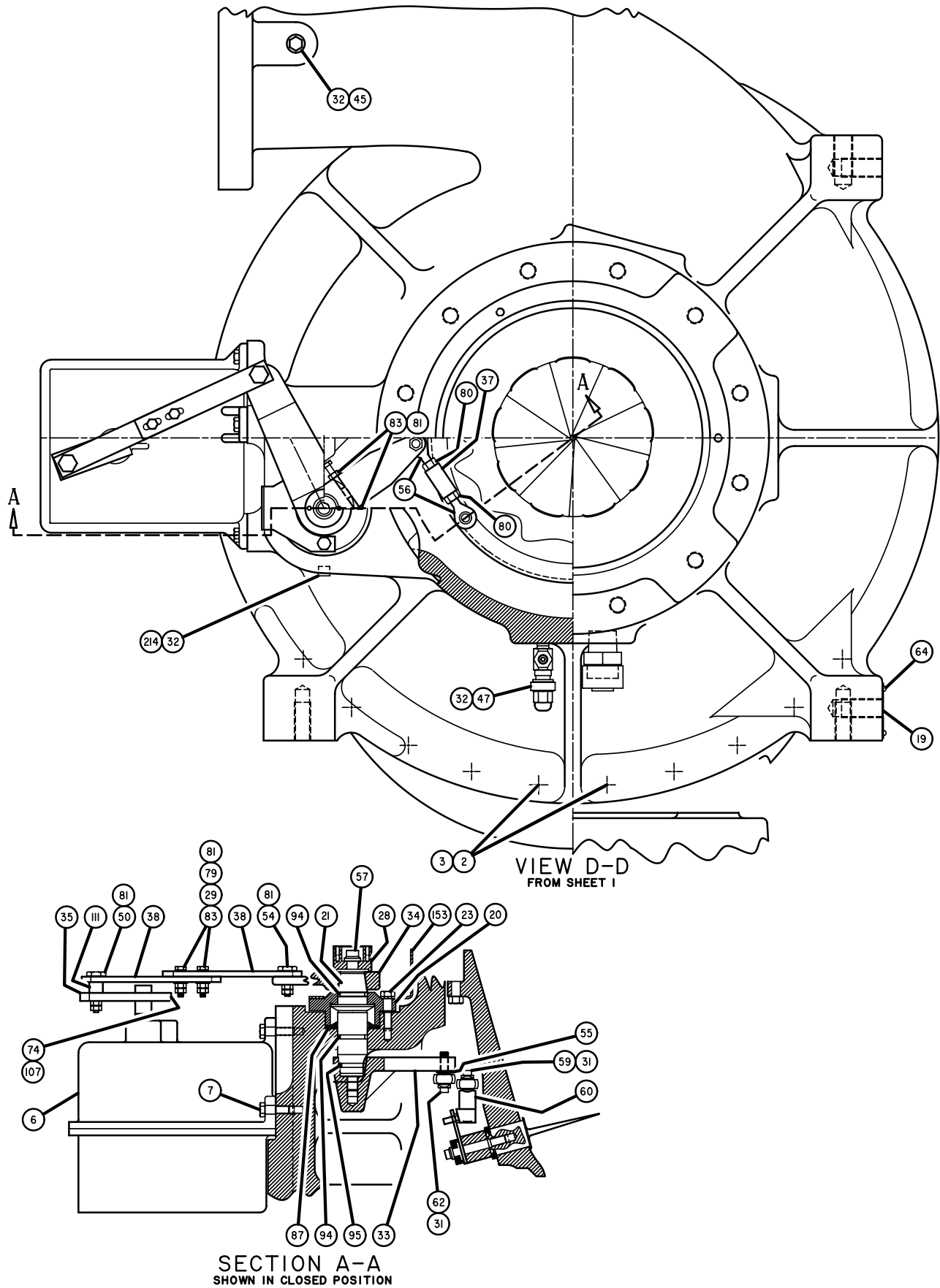
FIG. 7 – HB COMPRESSOR (61)
