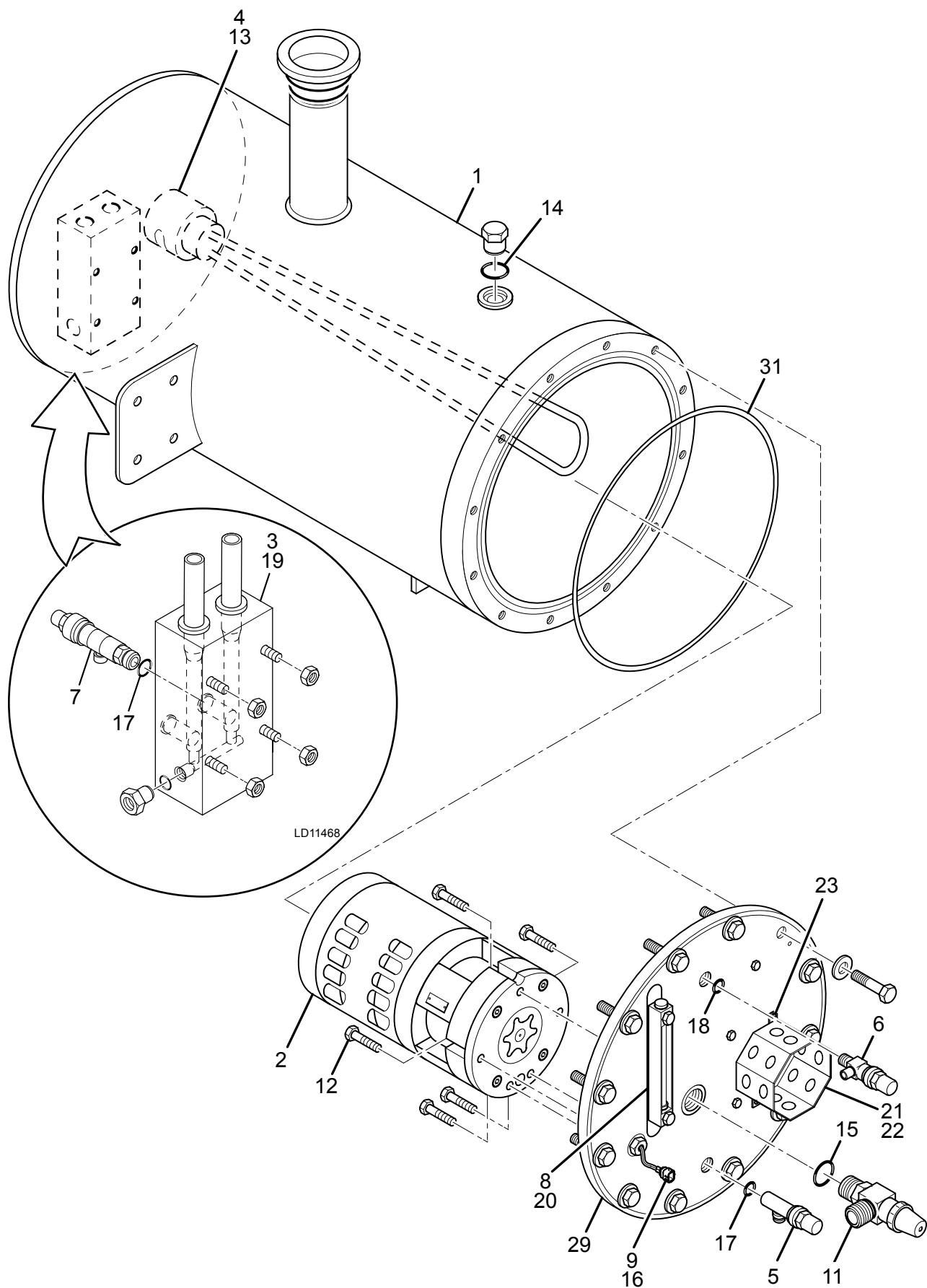
FIG. 56 – OIL PUMP HOUSING ASSEMBLY
