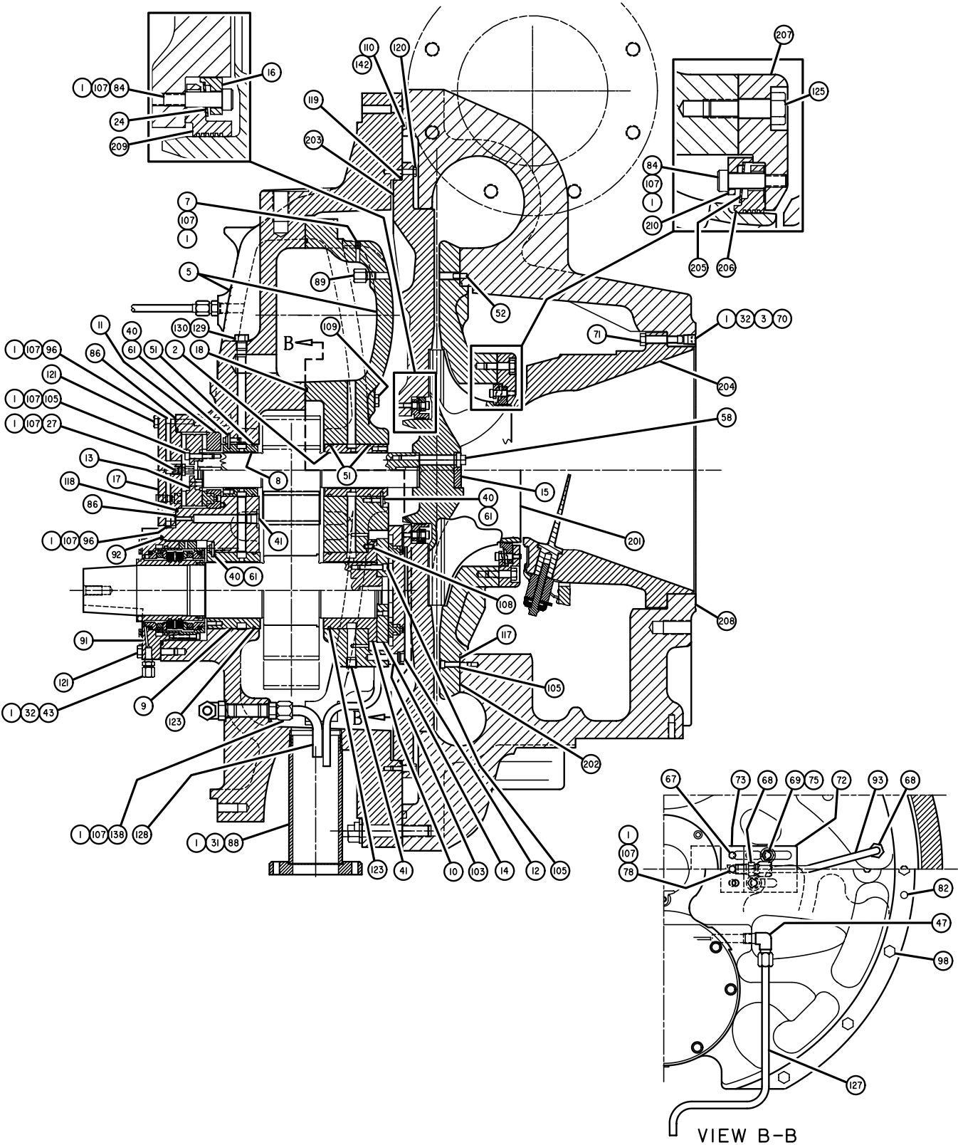
FIG. 28 – HG COMPRESSOR (65, 73)
