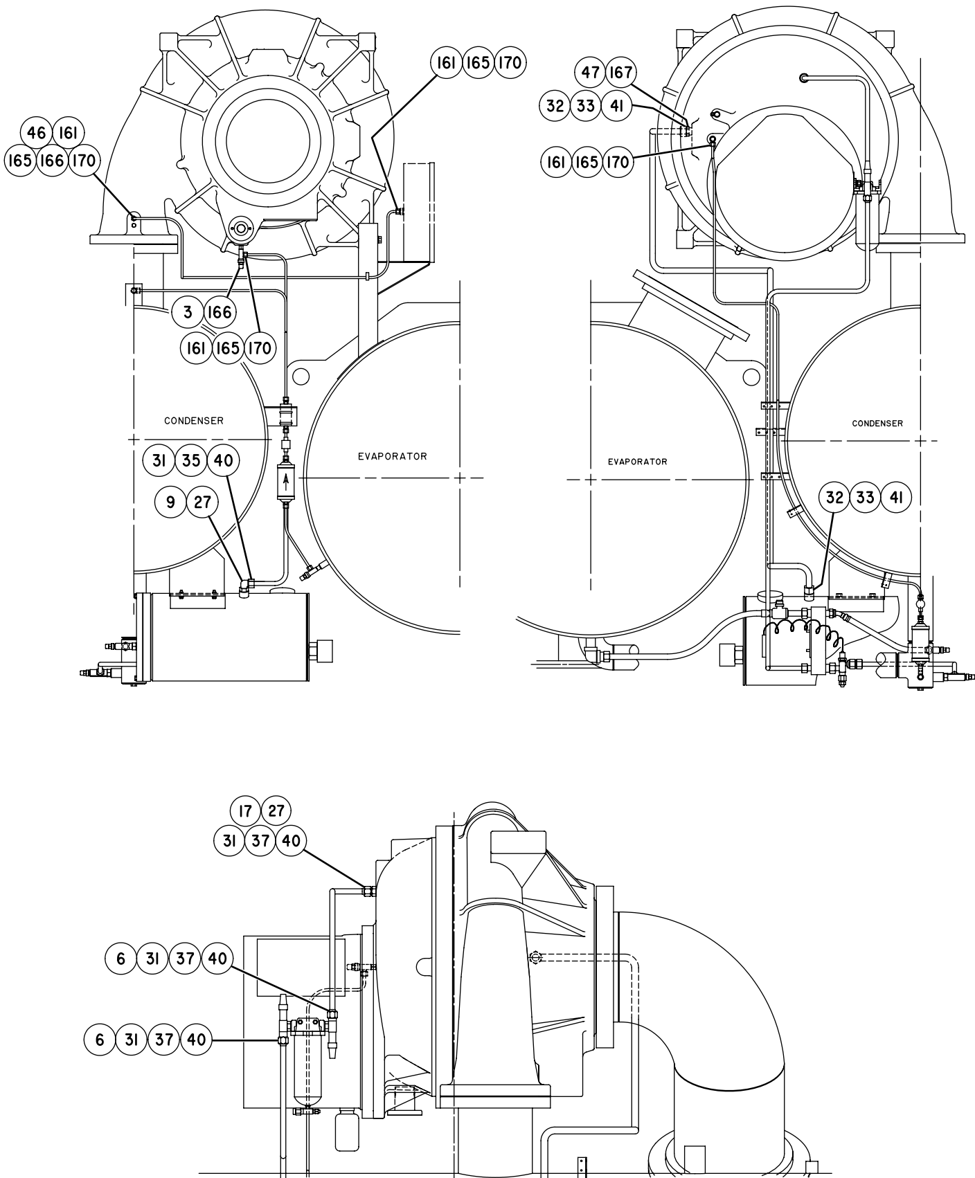
FIG. 58 - COMPRESSOR PIPING
