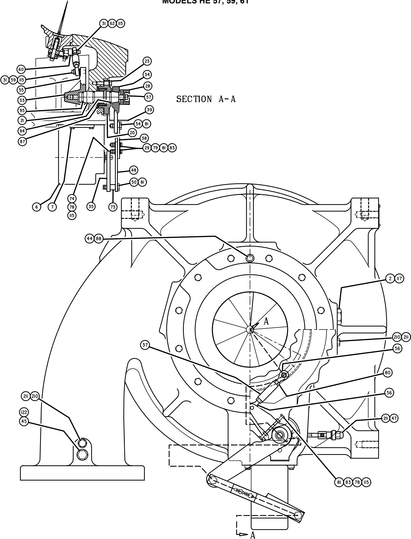
FIG. 17 – HE COMPRESSOR (57, 59, 61)
