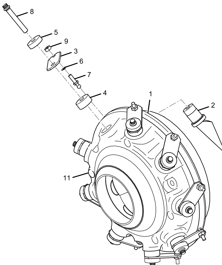
FIG. 27 – DEVICE PRE-ROTATION (HE 70)
