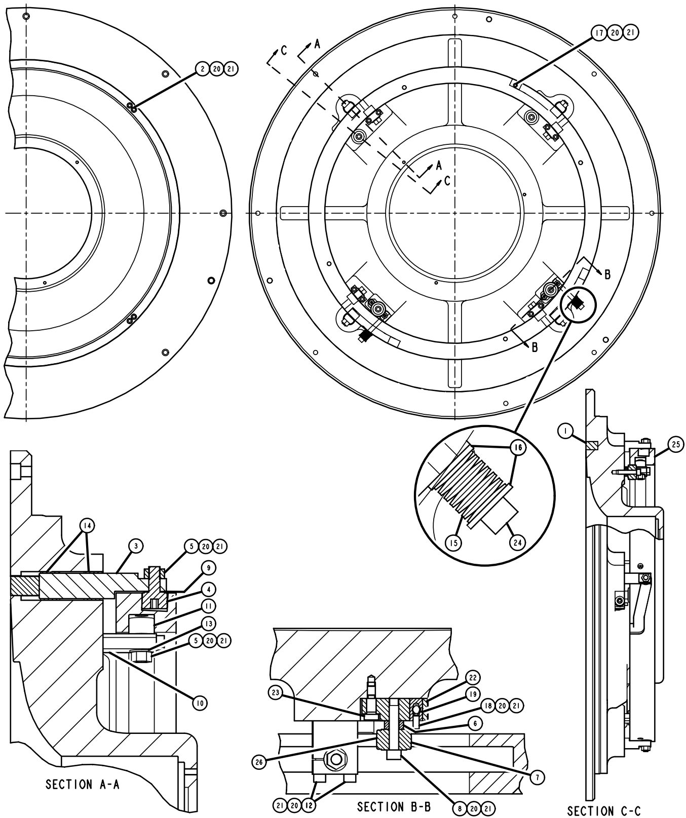
FIG. 50 – VGD DEVICE (HA 119)
