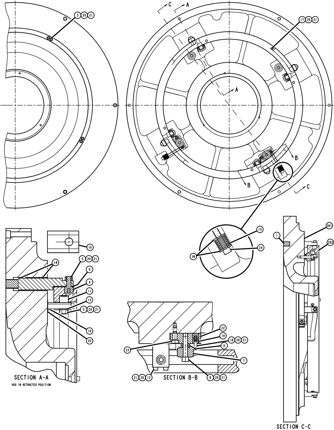
FIG. 50 – VGD DEVICE (HA 81, 90, 104)
