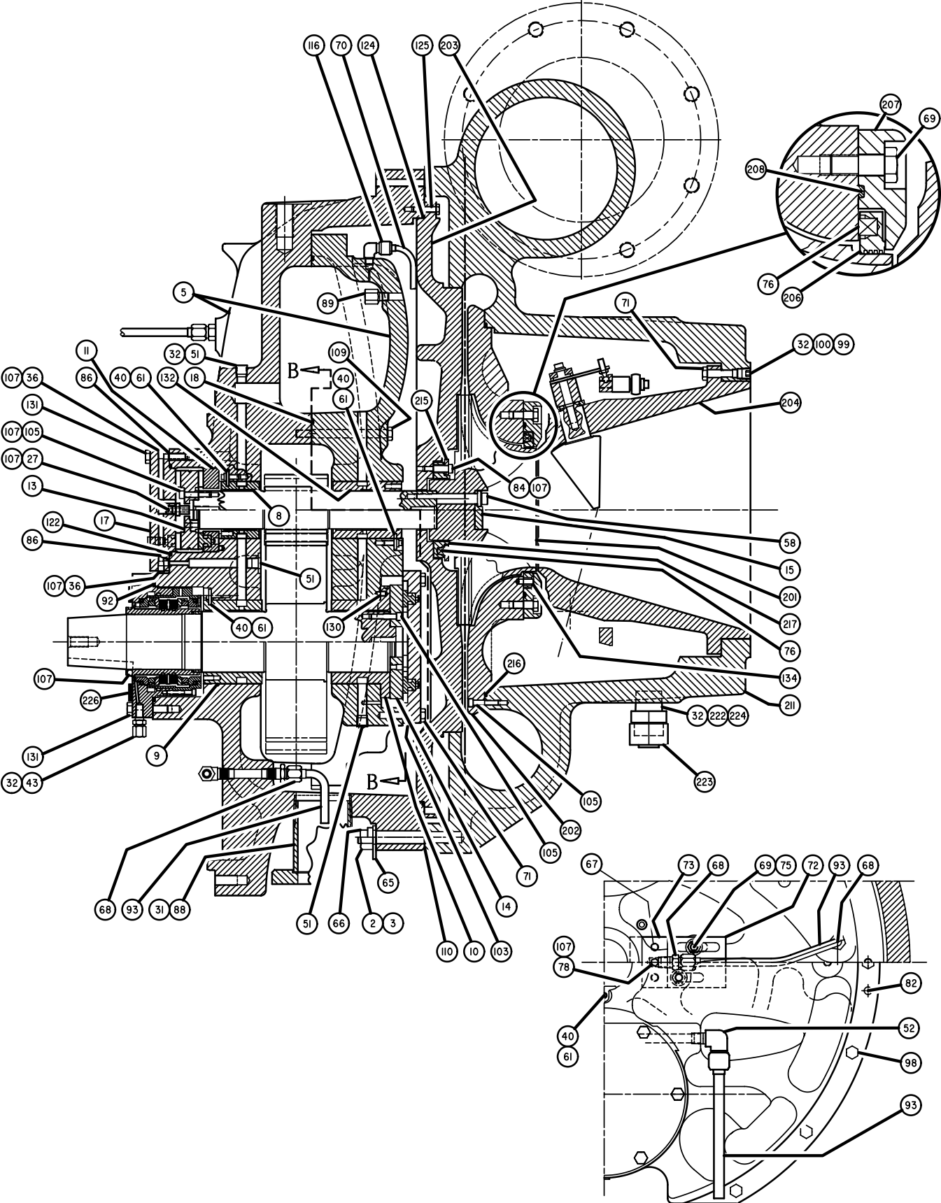
FIG. 5 – HB COMPRESSOR (61)
