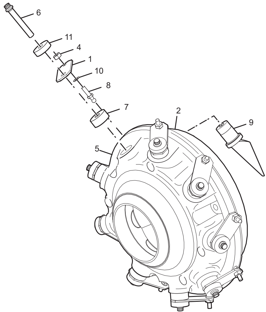
FIG. 25 – DEVICE PRE-ROTATION (MODELS 58 & 62)
