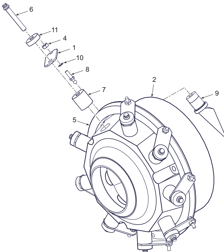
FIG. 20 – DEVICE PRE-ROTATION (MODELS 46 &amp; 52)
