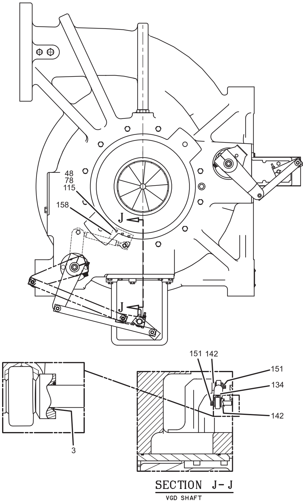
FIG. 26 – VGD DEVICE (MODELS 58 & 62)
