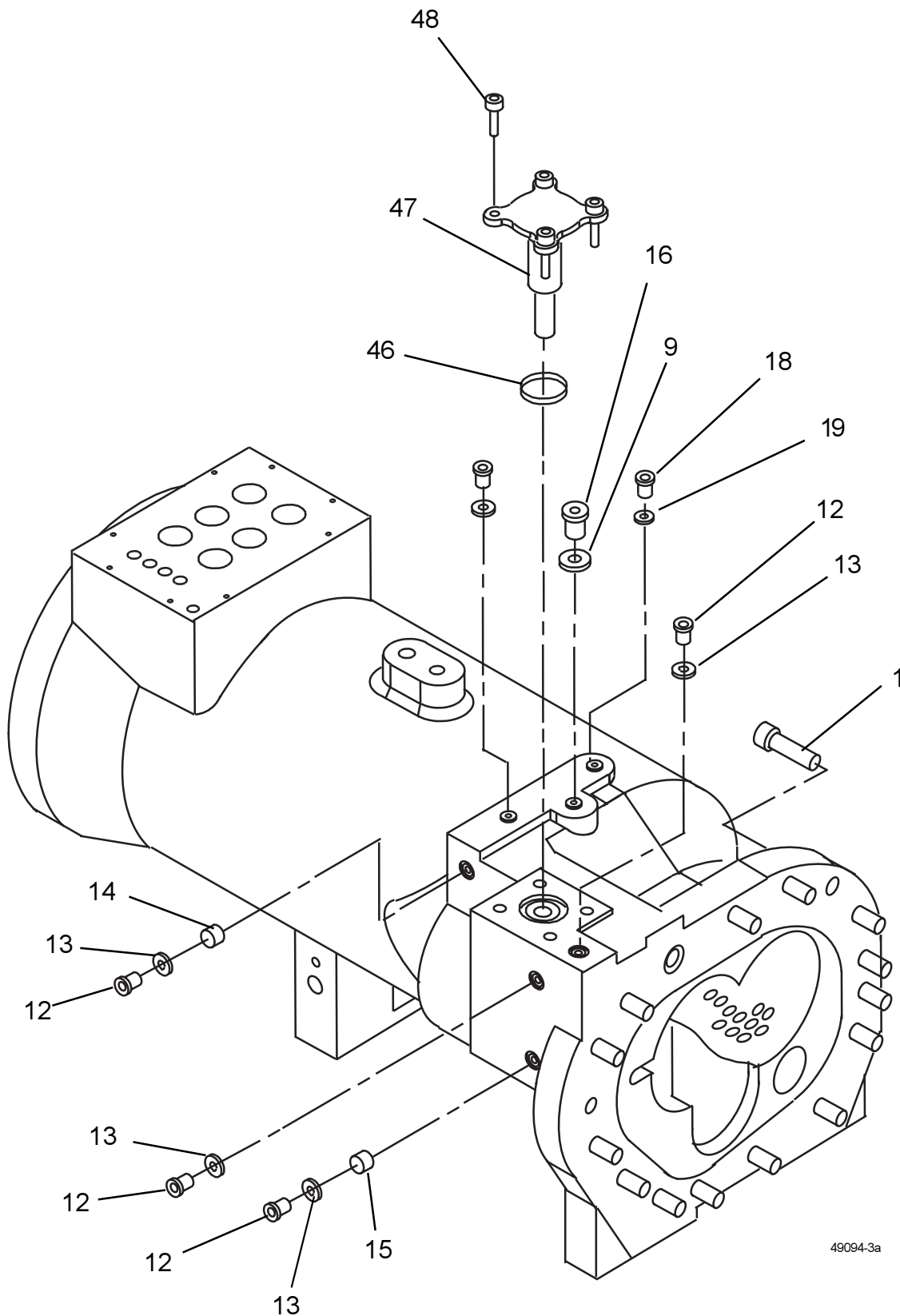
FIG. 9 – 124MM, 136MM & 145MM DXS COMPRESSOR PARTIAL EXPLODED VIEW (REF. TABLE 5, PAGES 21 AND 22)
