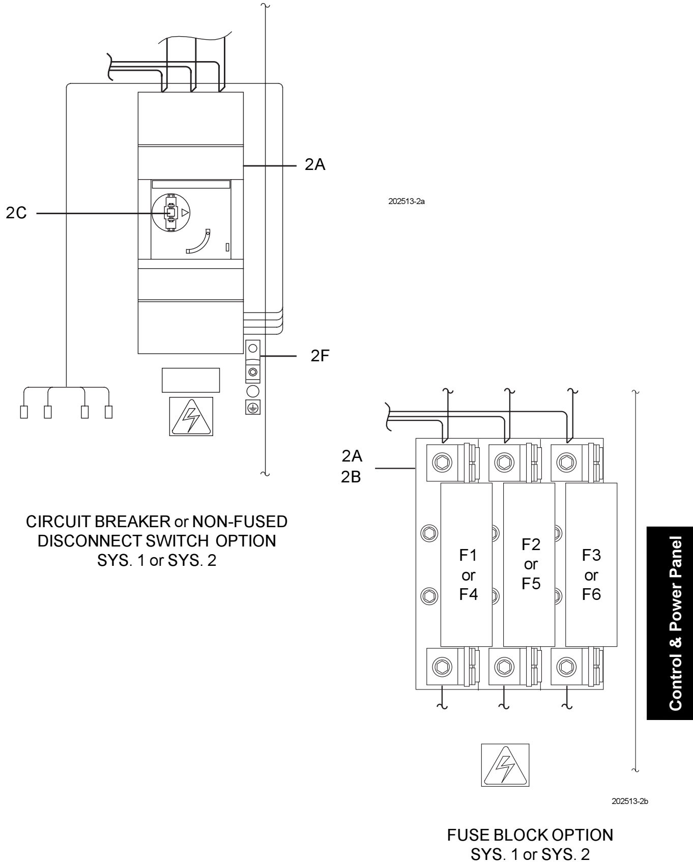
FIG. 15B – POWER PANEL COMPONENTS (REF. TABLES 9, PAGE 34)
