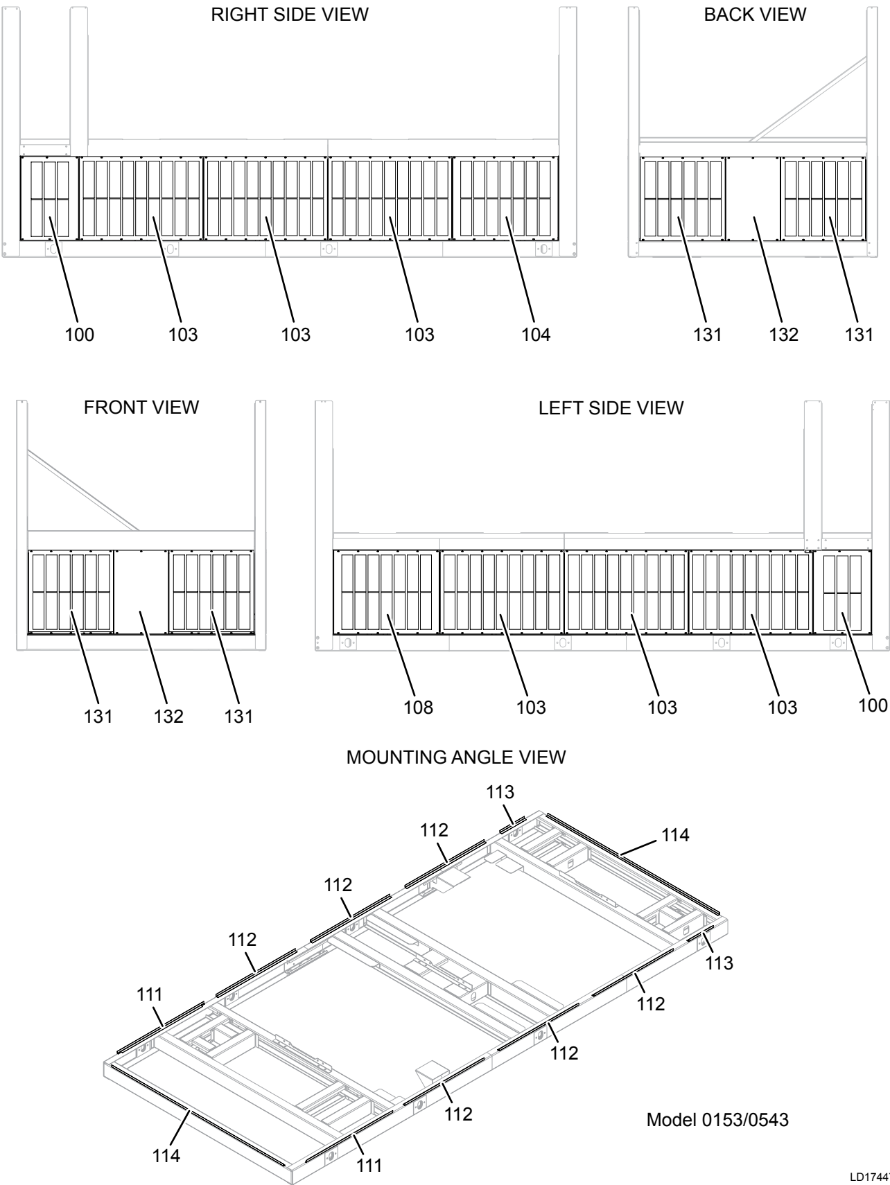
FIGURE 59 - BOTTOM SECTION: LOUVERED ENCLOSURE KIT COMPONENTS - MODEL 0153/0543
