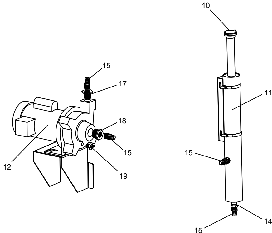
FIGURE 50 - GLYCOL LOOP COMPONENTS
