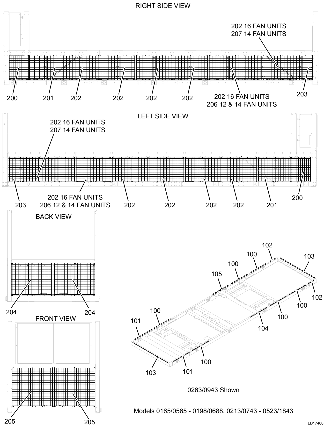
FIGURE 81 - WIRE ENCLOSURE KIT COMPONENTS - MODELS 0165/0565 - 0198/0688, 0213/0743 - 0523/1843
