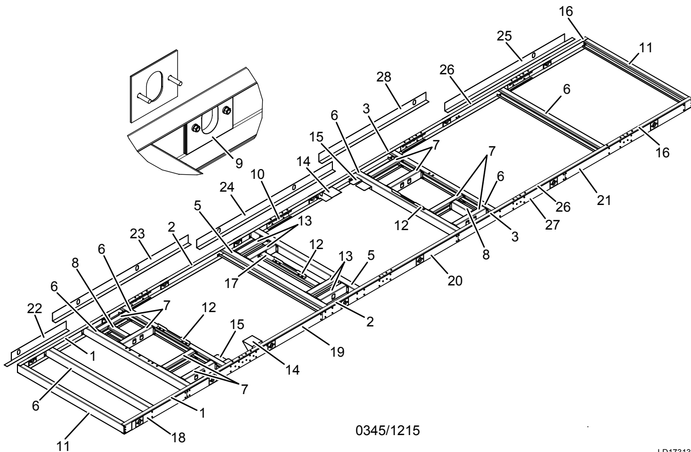
FIGURE 12 - BASE ASSEMBLY (0333/1173, 0343/1193, 0345/1215)
