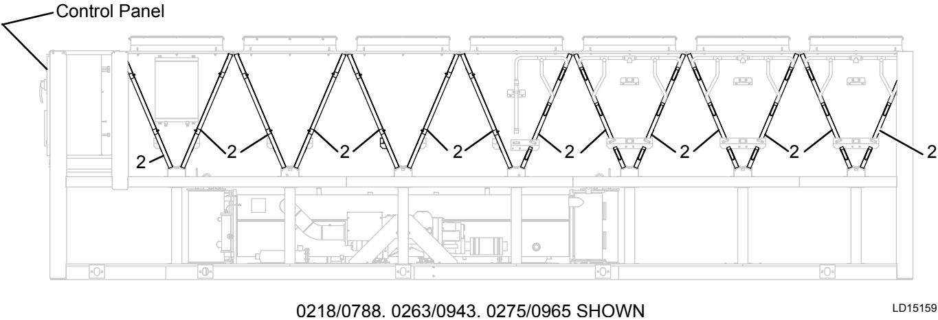
FIGURE 14 - CONDENSER COILS, TYPICAL CONFIGURATION
