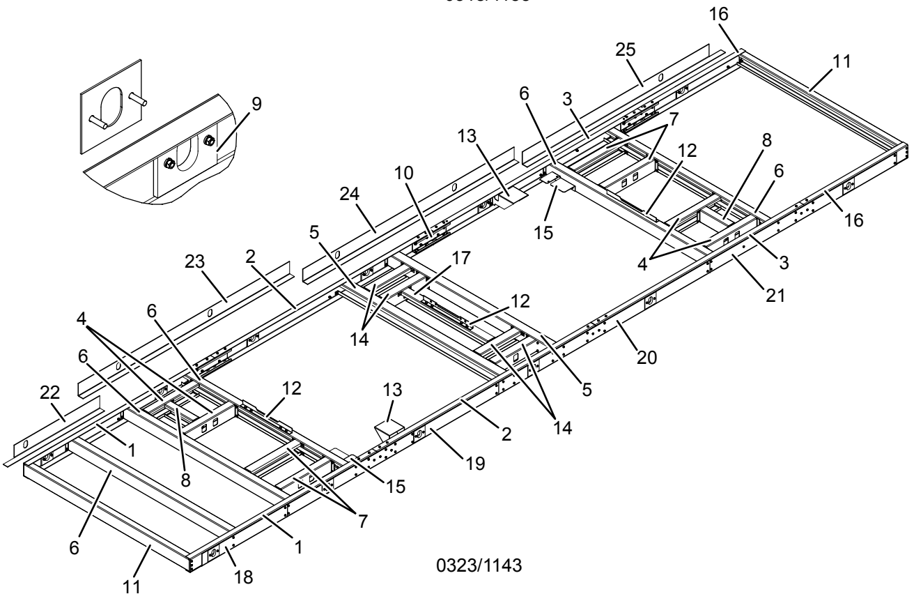
FIGURE 11 - BASE ASSEMBLY (0318/1188, 0323/1143)
