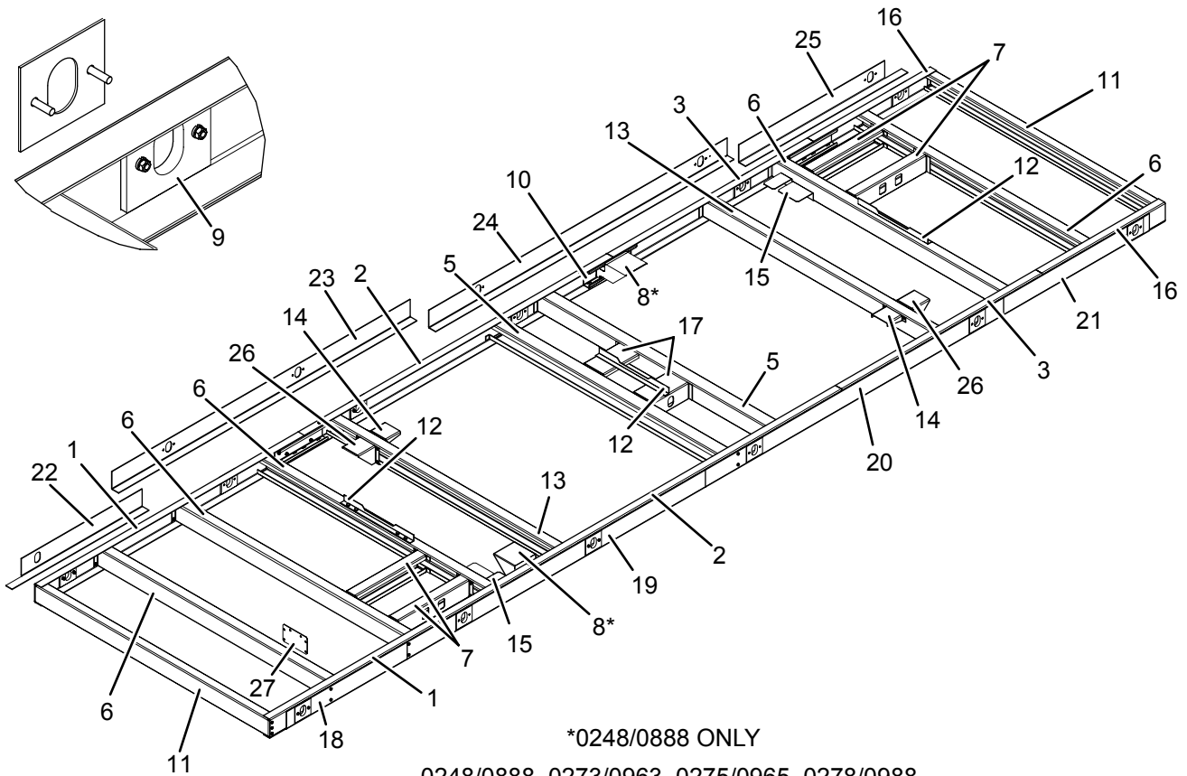
FIGURE 8 - BASE ASSEMBLY (0233/0843, 0248/0888, 0273/0963, 0275/0965, 0278/0988)
