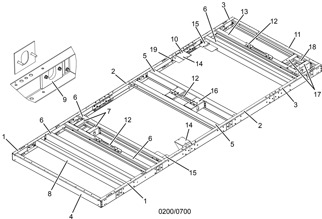
FIGURE 7 - BASE ASSEMBLY (0198/0688, 0200/0700)
