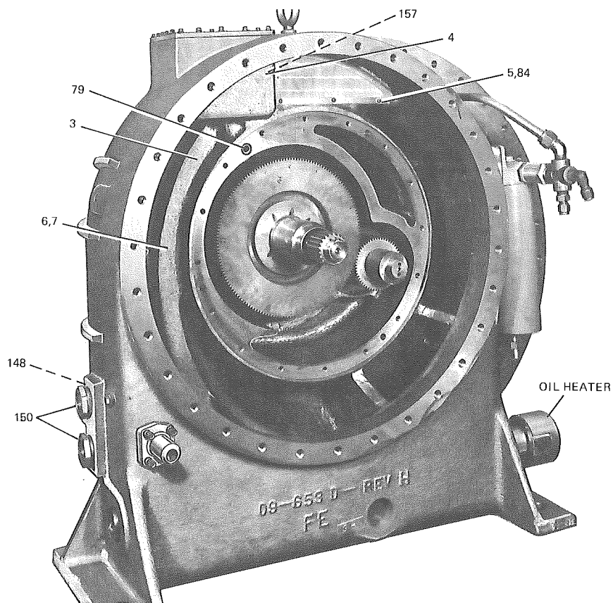
FIG. 6— COMPRESSOR INTERNAL VIEW, PARTS LOCATION
