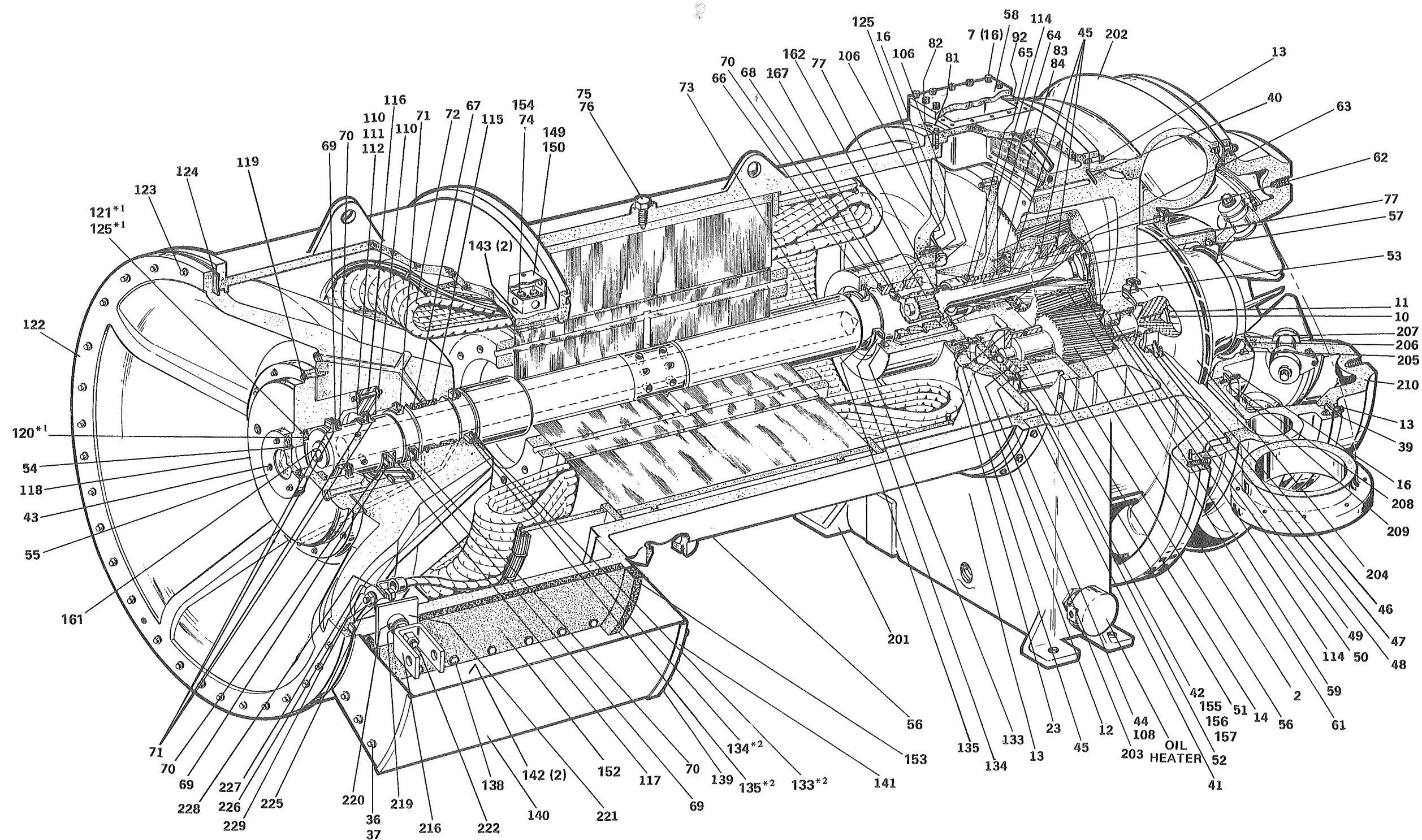
FIG. 2— MODEL MKB65 & MKB73 COMPRESSORS, PARTS LOCATION
