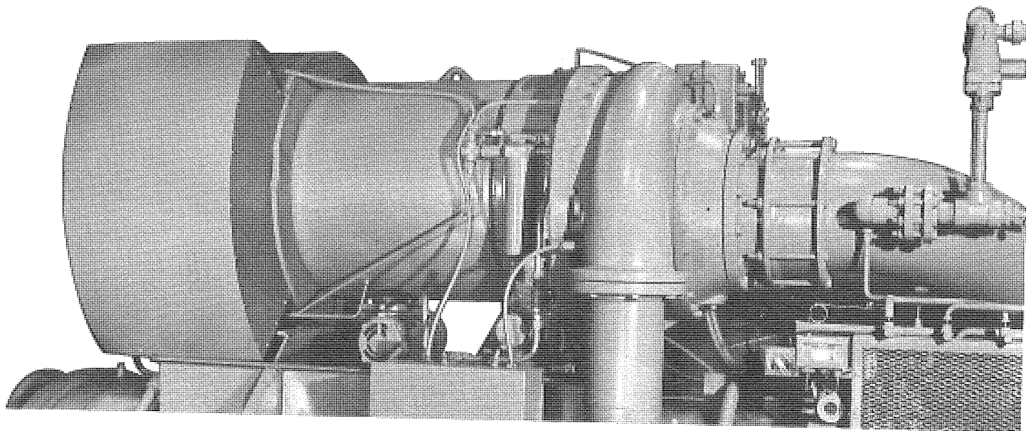
FIG. 1— HERMETIC—MOTOR COMPRESSOR, MODEL MKB
