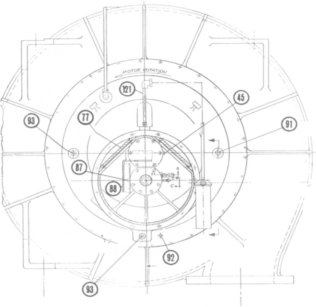
SECTION F-F
