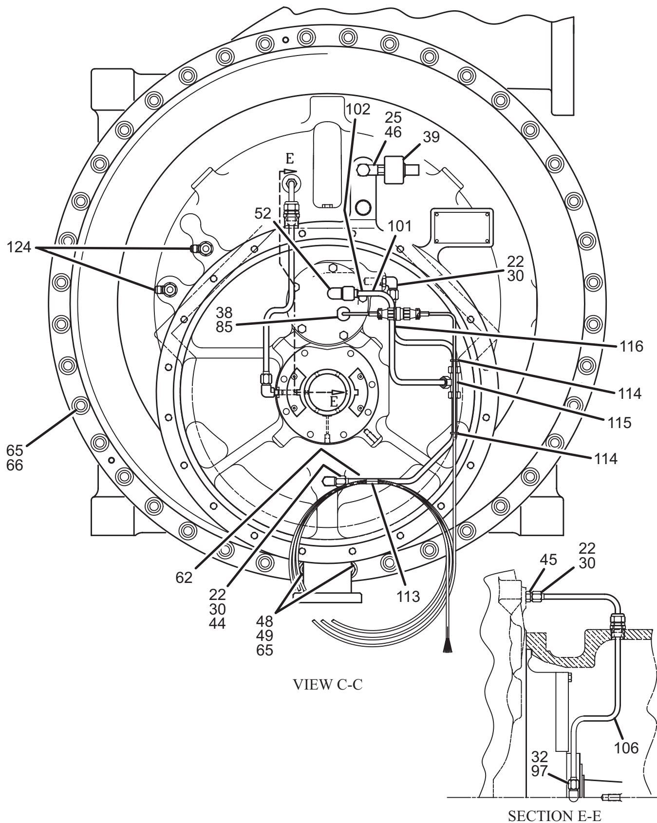
FIGURE 17 - YD COMPRESSOR COMPONENTS (J1/J2)
