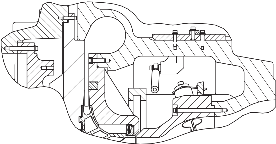
SECTION J-J
