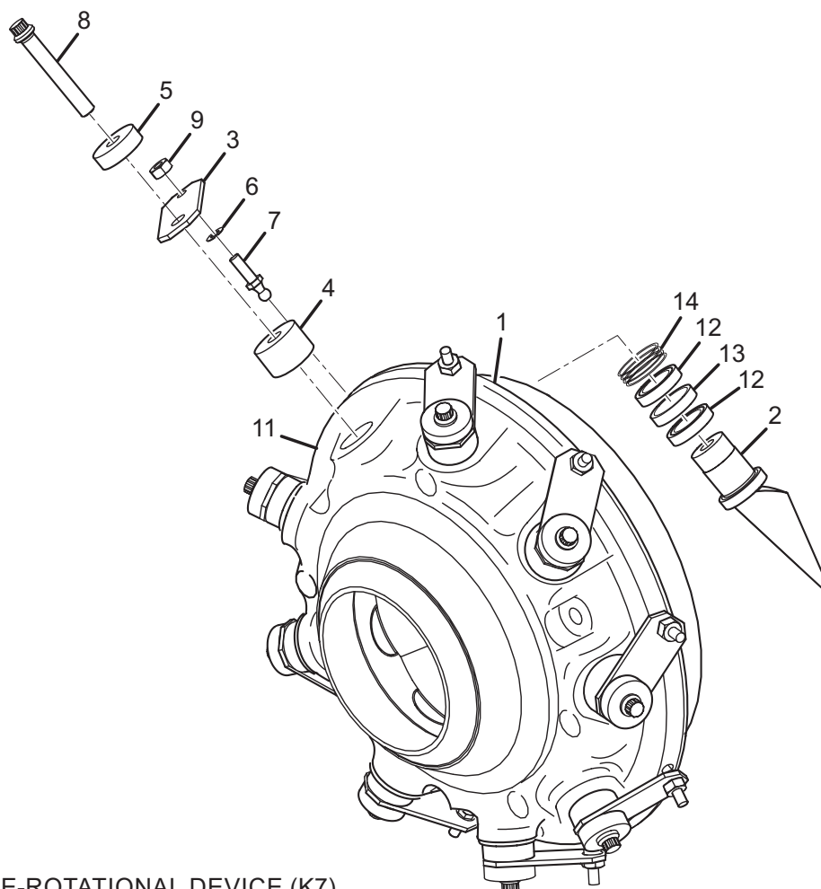
FIGURE 53 - PRE-ROTATIONAL DEVICE (K7)
