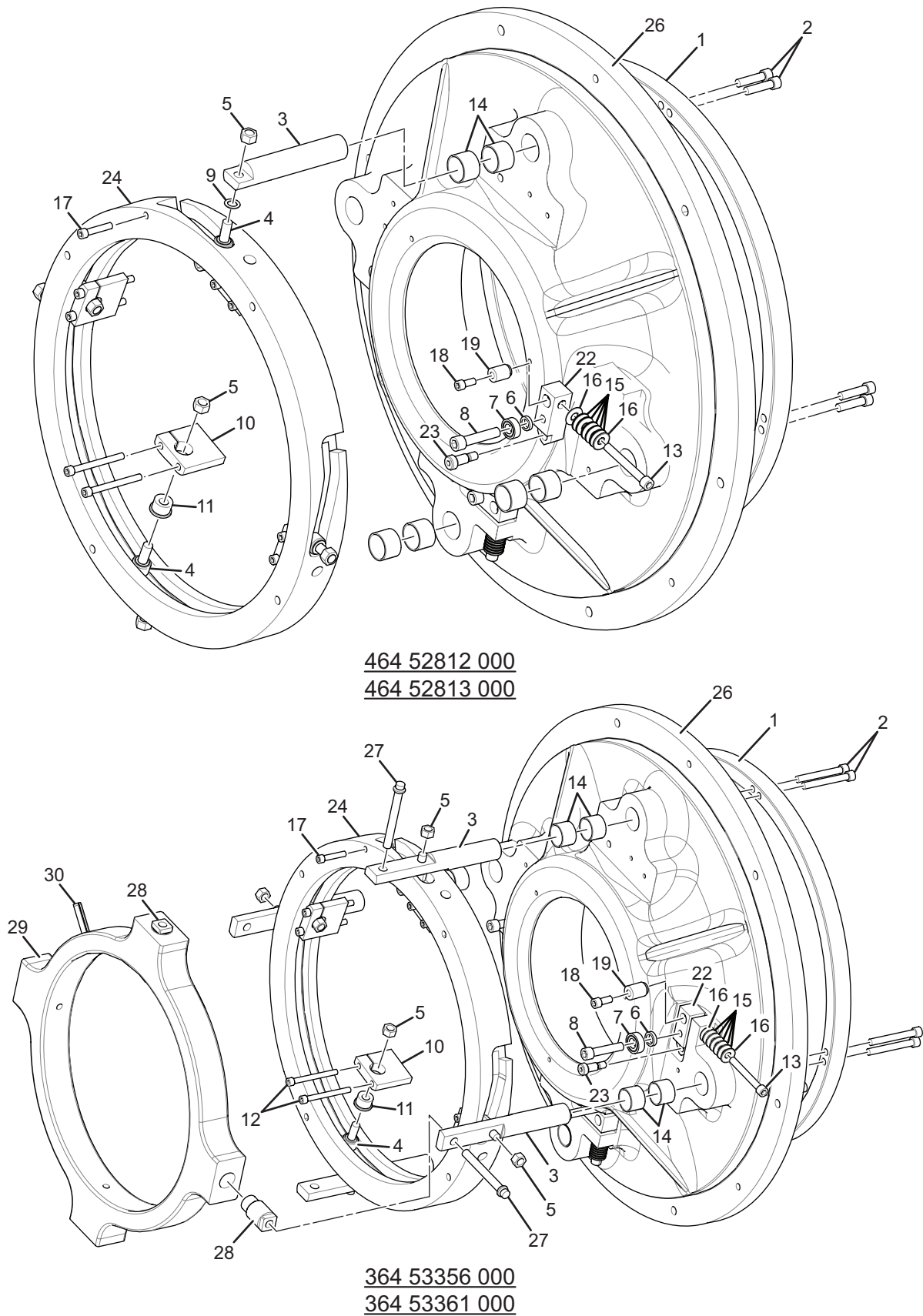
FIGURE 42 - VARIABLE GEOMETRY DIFFUSER (K1/K2)
