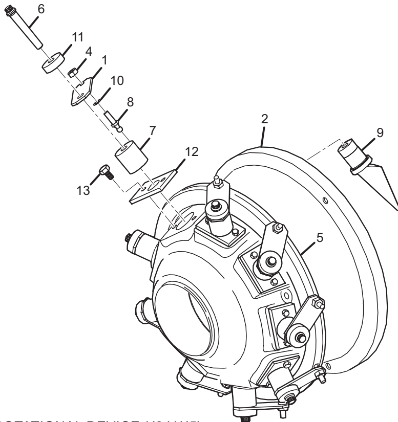
FIGURE 29 - PRE-ROTATIONAL DEVICE (J3J4/J5)
