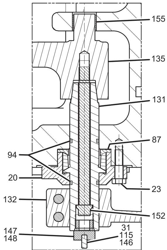
SECTION I-I
