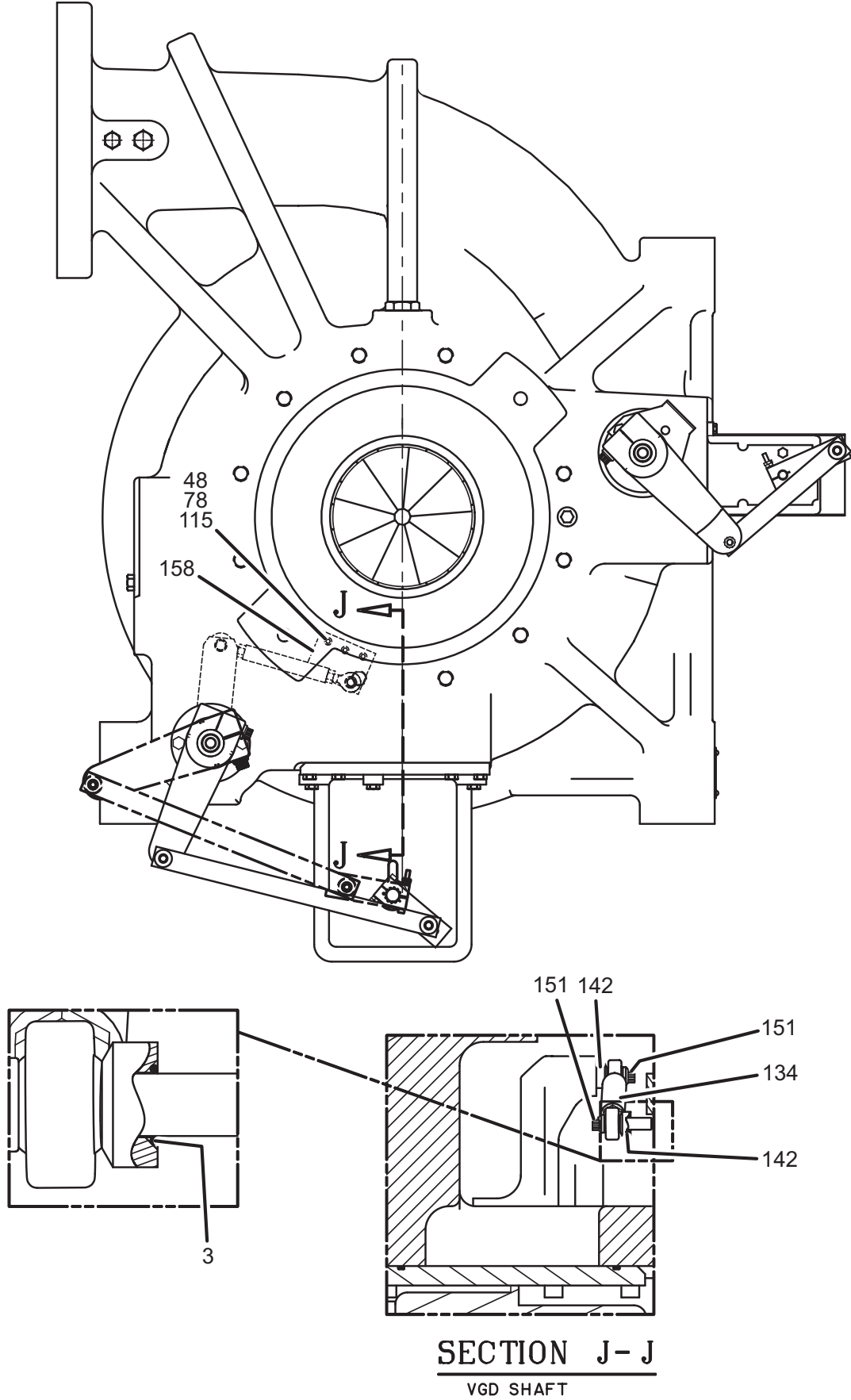
FIGURE 19 - YD COMPRESSOR COMPONENTS (J1/J2)
