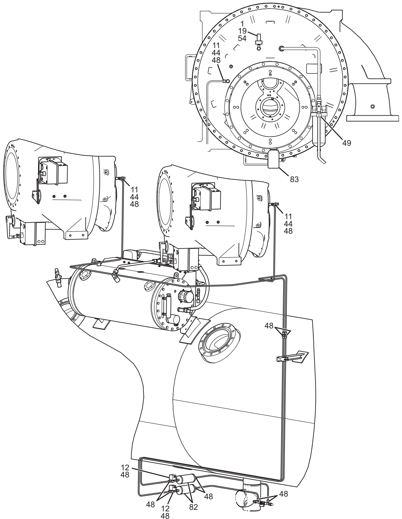
FIGURE 7 - YD UNIT PIPING (MOD B-C)
