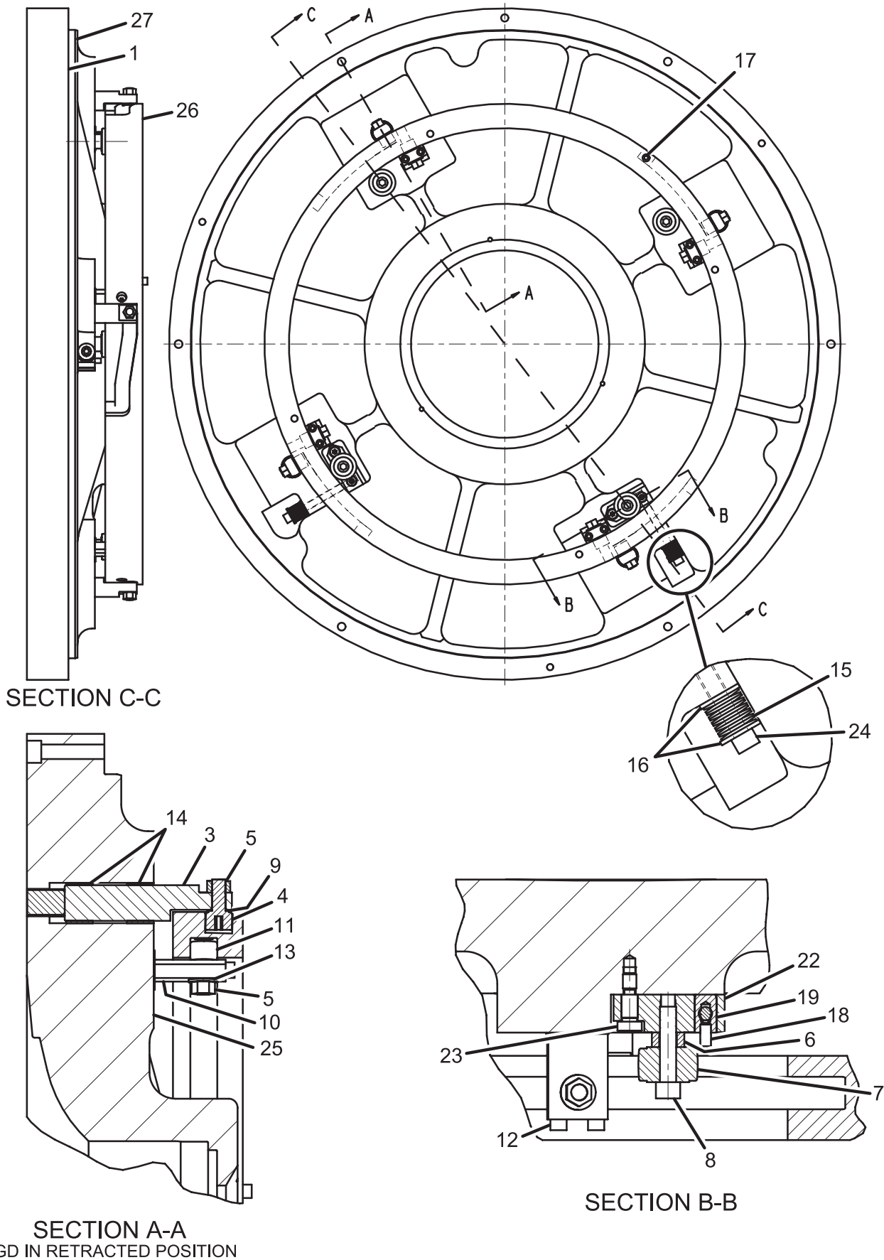
FIGURE 30 - VARIABLE GEOMETRY DIFFUSER (J3J4/J5)
