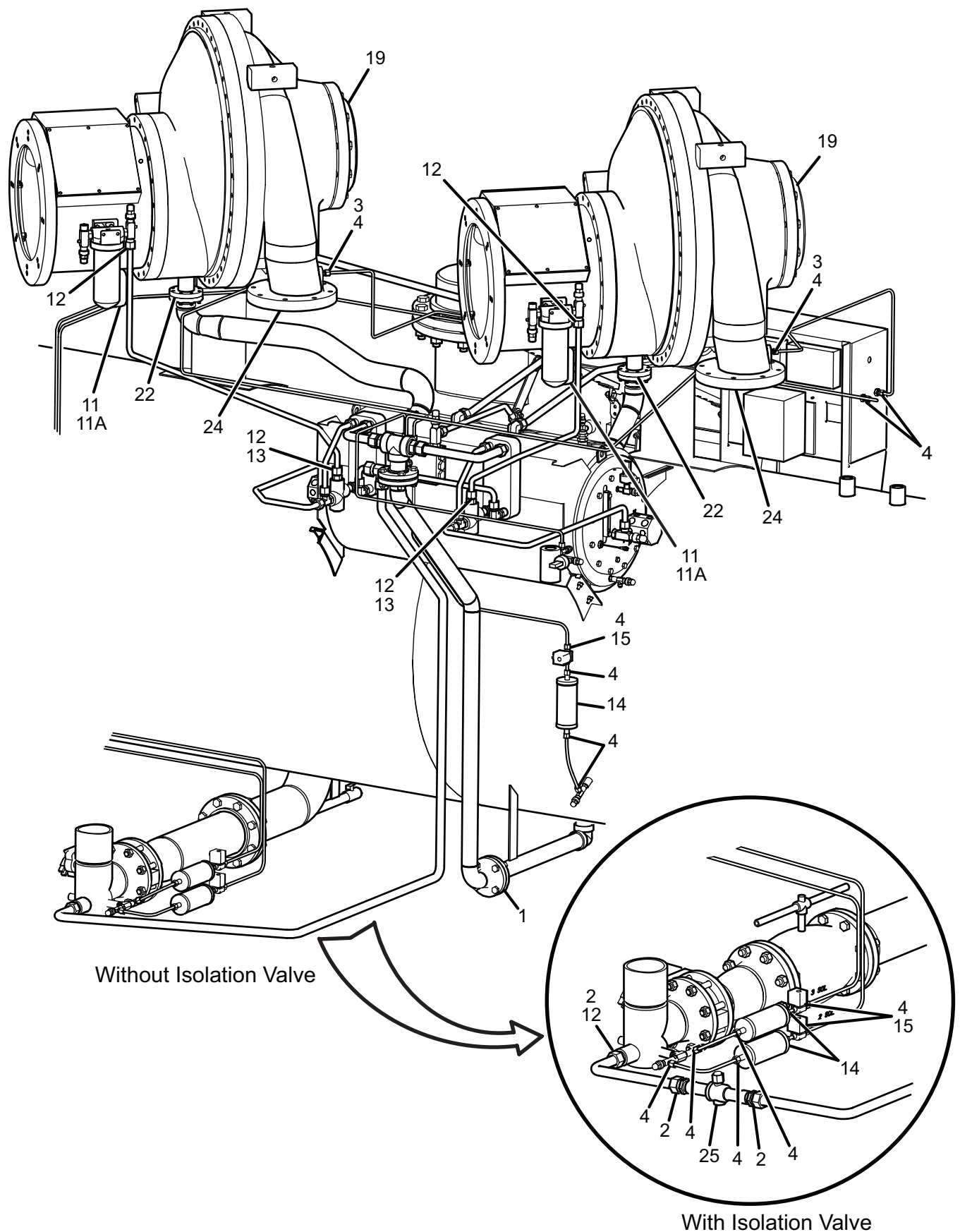
FIGURE 2 - YD UNIT PIPING (MOD A)
