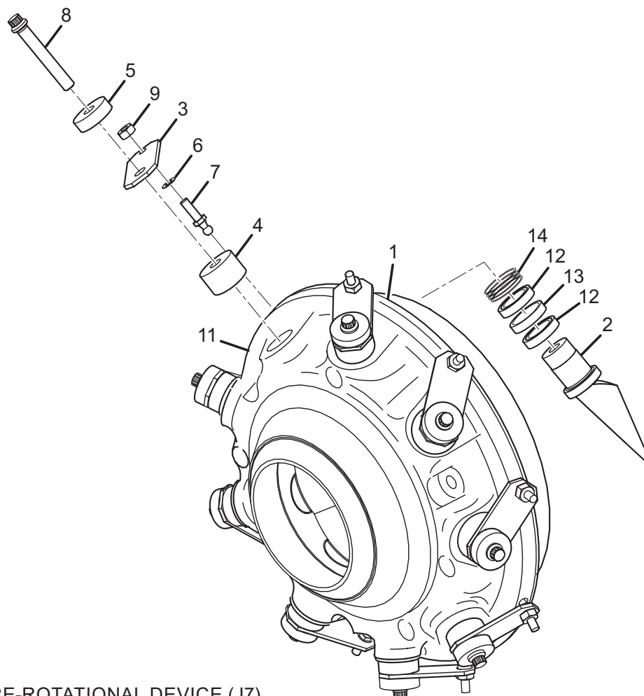
FIGURE 35 - PRE-ROTATIONAL DEVICE (J7)
