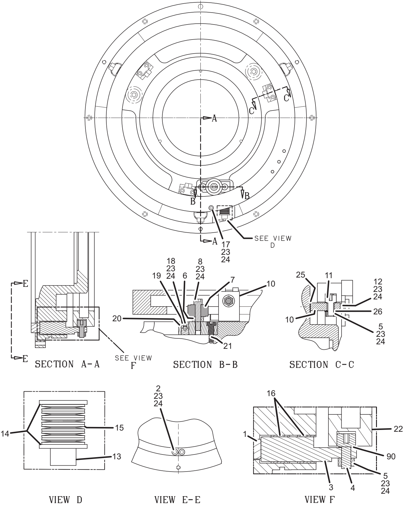
FIGURE 22 - VARIABLE GEOMETRY DIFFUSER (J1/J2)
