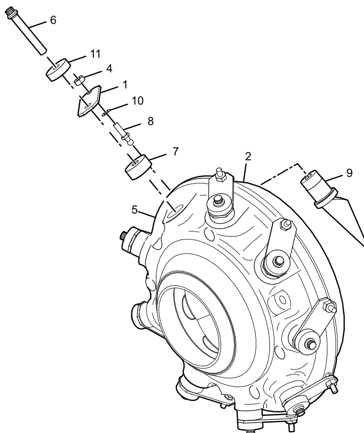
FIGURE 21 - PRE-ROTATIONAL DEVICE (J1/J2)
