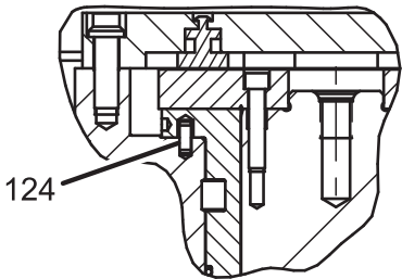
SECTION G-G
