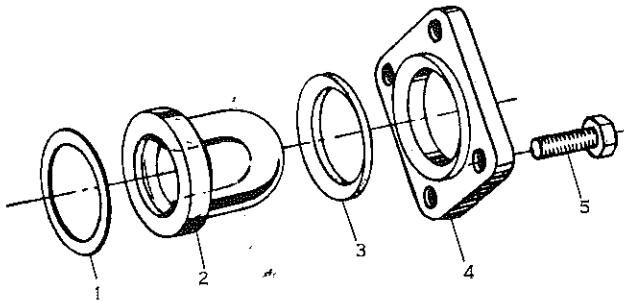
FIG. 8— Oil Sight Glass - Bulb Type
