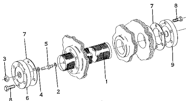
FIG. 5— Suction Strainer Assembly
