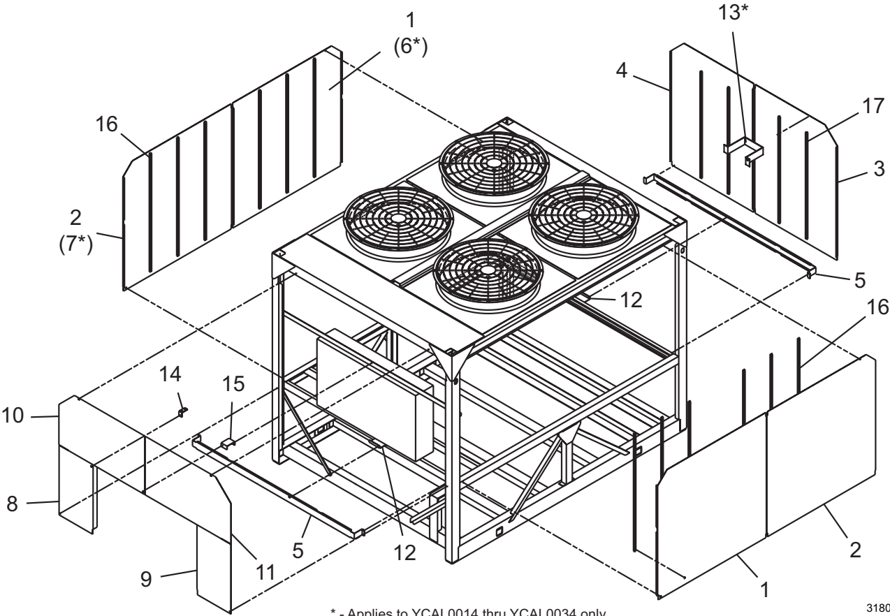
FIG. 16 – LOUVERED ENCLOSURE (TOP SECTIONS) - 475-31806-000 SHOWN (REF. TABLE 13)
