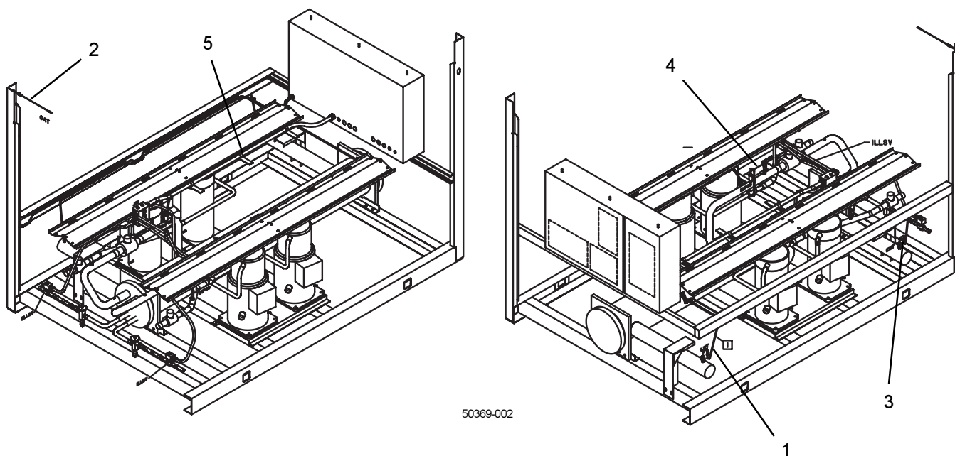
FIG. 12B – SENSOR HARNESS - YCAL0040-YCAL0060 (REF. TABLE 8B)
