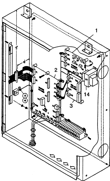
ELECTRONIC PANEL
