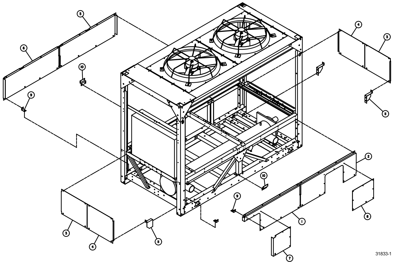
FIG. 17 – LOUVERED ENCLOSURE (BOTTOM SECTIONS) - YCAL0073, 0087 &amp; YCAL0107
