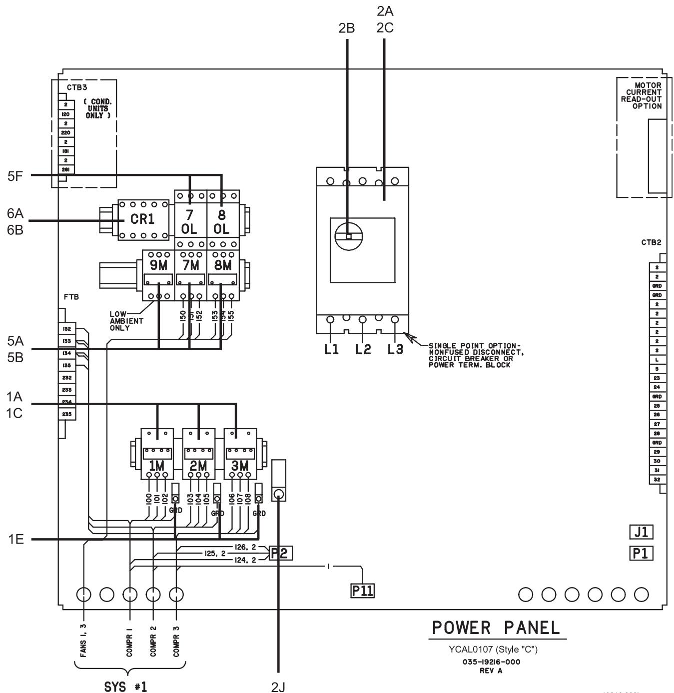
FIG. 8 – POWER PANEL COMPONENTS - YCAL0107 (REF. TABLE 7, PAGES 27-38)
