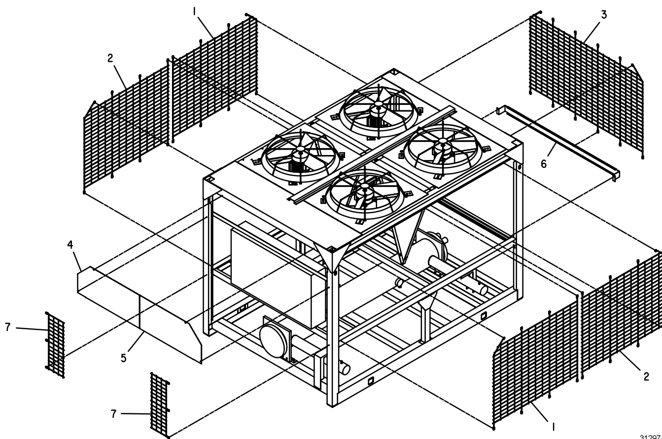
FIG. 18 – WIRE ENCLOSURE (TOP SECTIONS) - YCAL0117, 0133, 0147, 0157 &amp; YCAL0173 SHOWN
