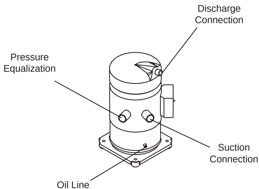
FIG. 5A – COMPRESSOR (REF. TABLE 6, PAGES 17 AND 18)
