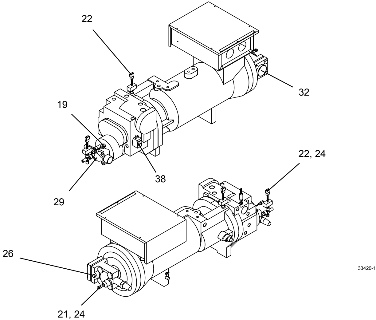
FIG. 16 – TRANSDUCERS, PRESSURE CUTOUTS AND TEMP SENSORS (REF. TABLE 11)
