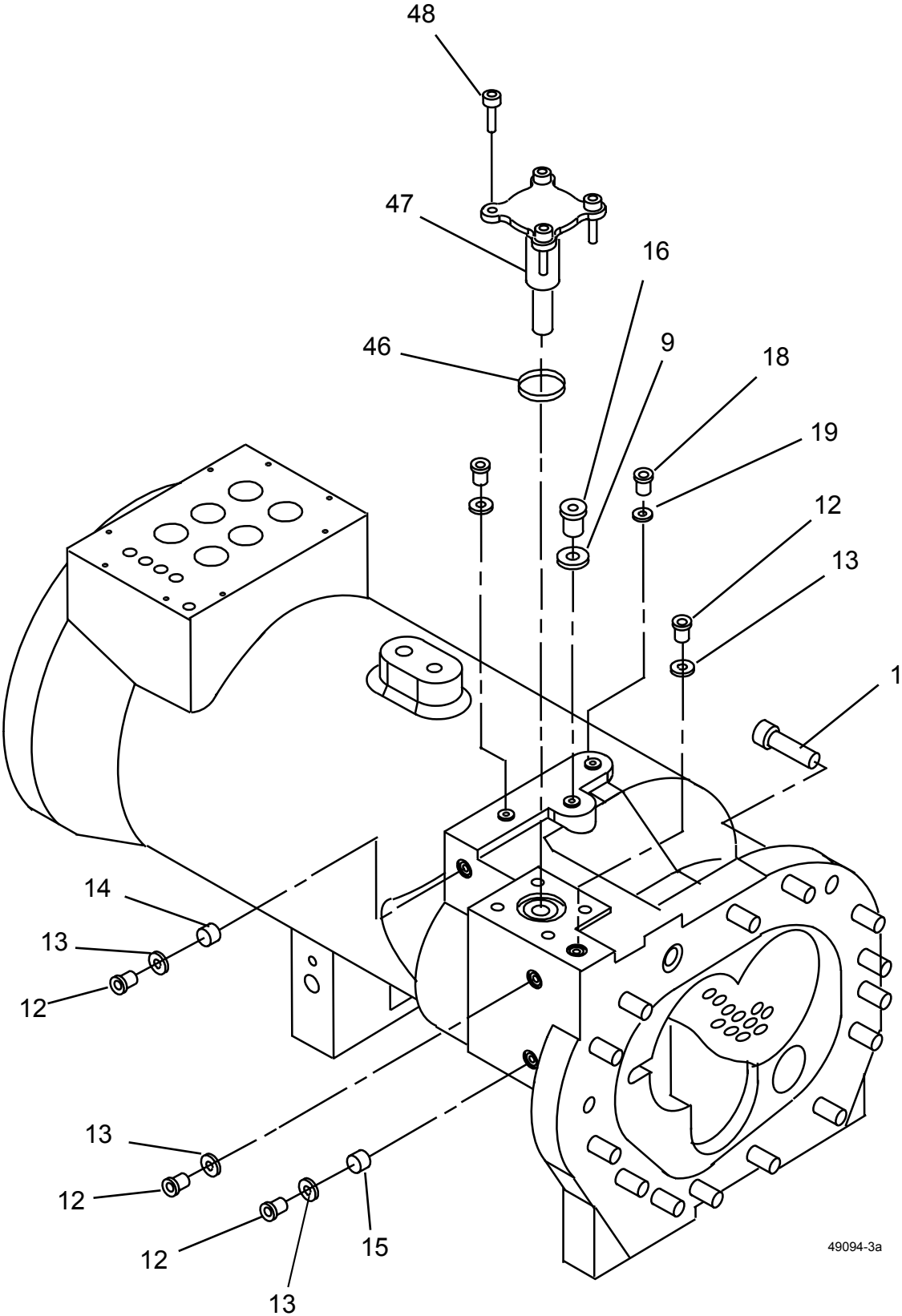
FIG. 9 – 124MM, 136MM & 145MM DXS COMPRESSOR PARTIAL EXPLODED VIEW (REF. TABLE 6, PAGES 21 AND 22)
