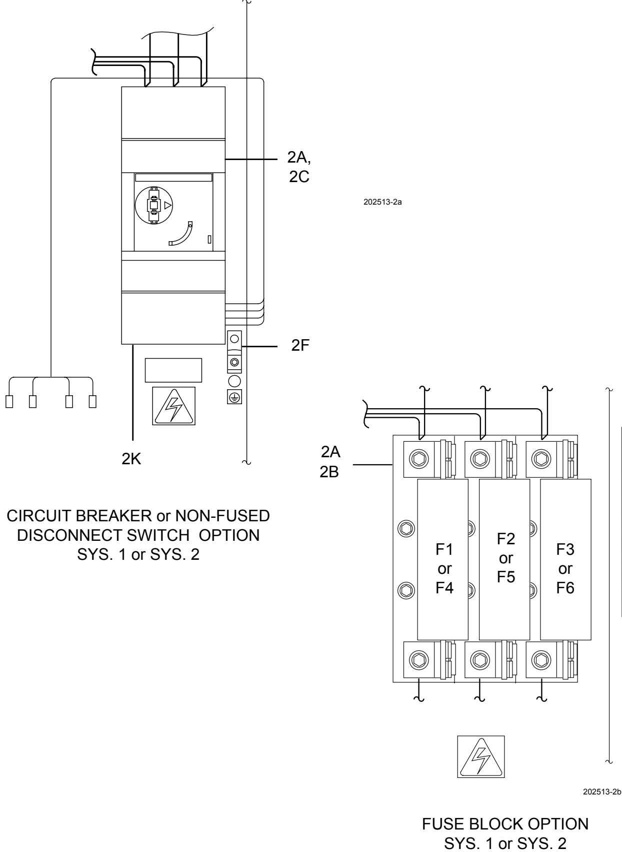
FIG. 15B – POWER PANEL COMPONENTS (REF. TABLES 9 AND 10, PAGES 34-41)
