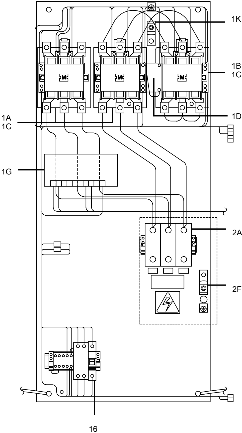
FIG. 15A – POWER PANEL COMPONENTS (REF. TABLES 9 AND 10, PAGES 34-41)
