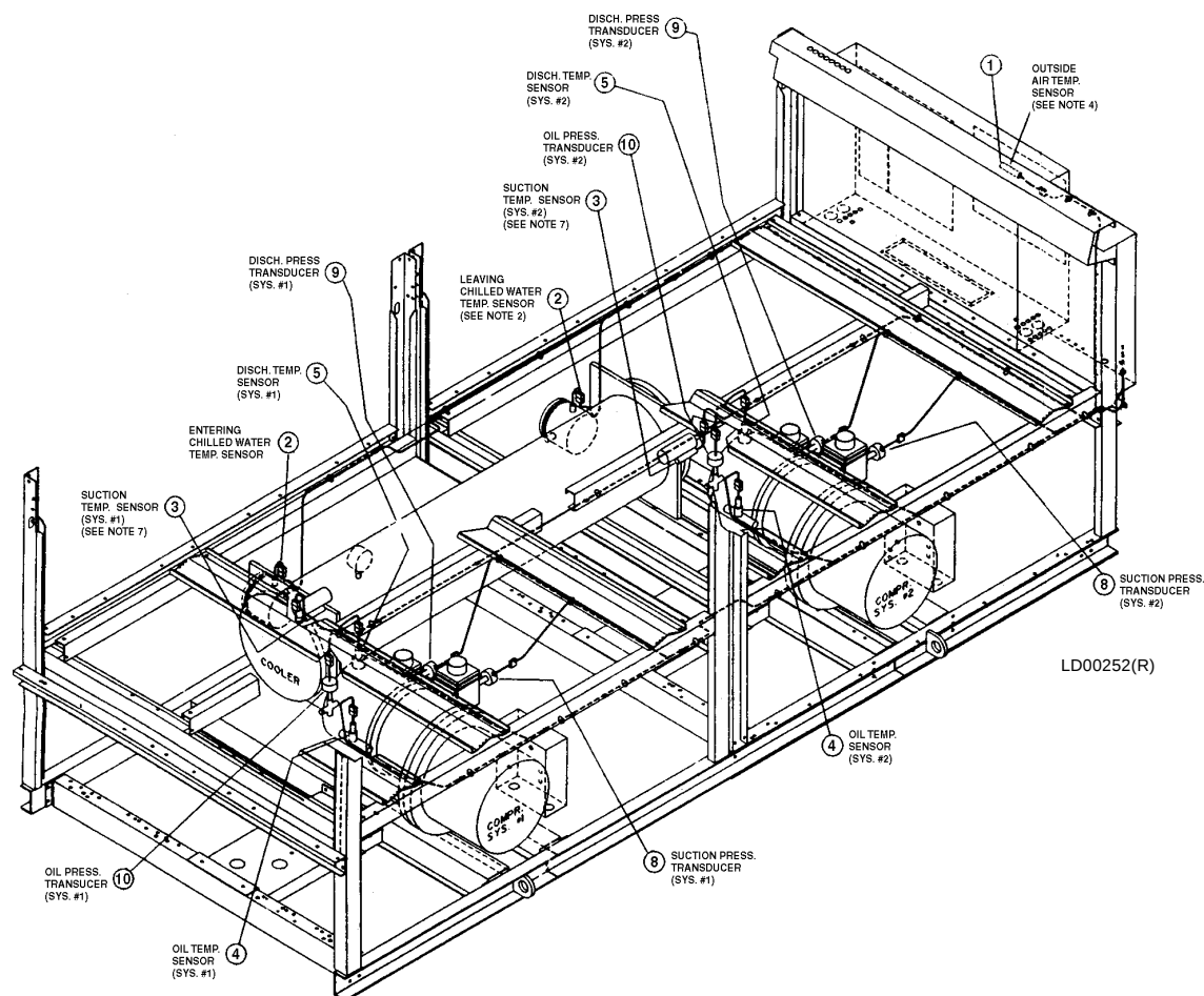
FIG. 5 – SYSTEM CONTROLS
