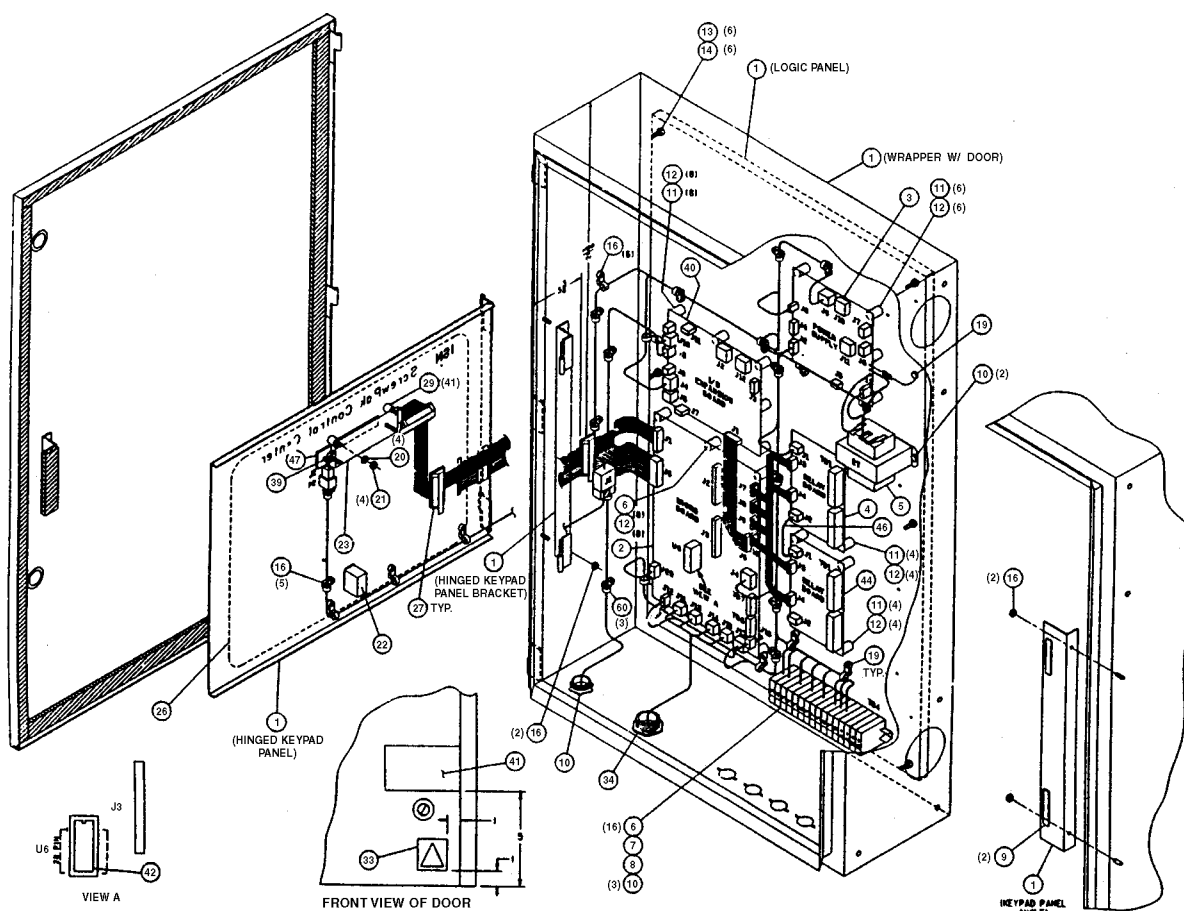
FIG. 1 – CONTROL PANEL, BOX
