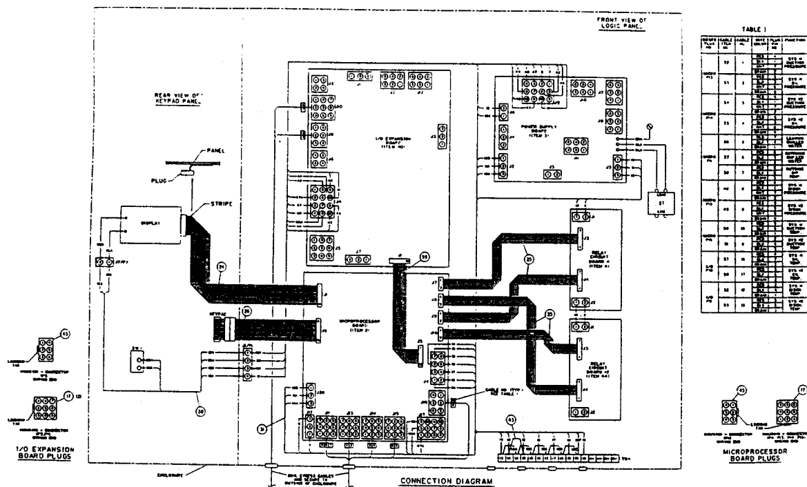
FIG. 2 – CONTROL PANEL, CONNECTION DIAGRAM
