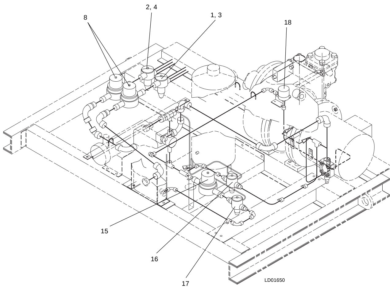
FIG. 7 – SYSTEM PIPING
