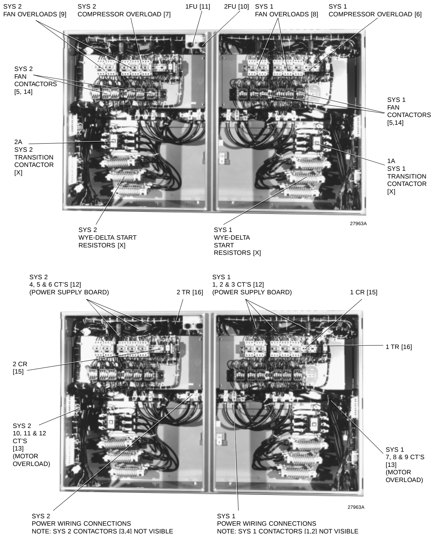
FIG. 3 – WYE-DELTA START POWER PANEL
