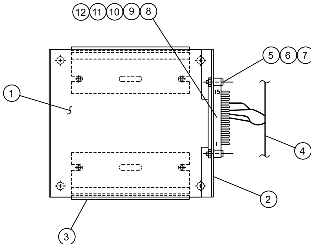
FIG. 15 – REMOTE TEMPERATURE RESET KIT COMPONENTS
