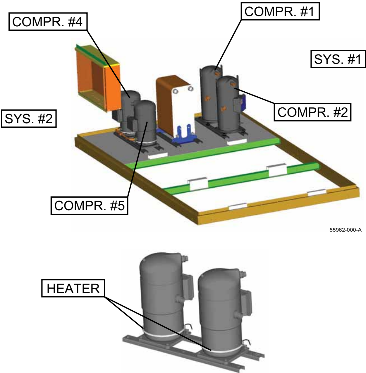
FIG. 5 – COMPRESSOR - TYPICAL LAYOUT (REF. TABLES 6A AND 6B, PAGE 19)
