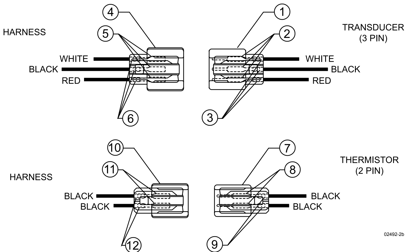
FIG. 10 – TRANSDUCER AND THERMISTOR WIRE HARNESS CONNECTORS - FIELD REPLACEMENT PART NUMBERS (REF. TABLE 12)
