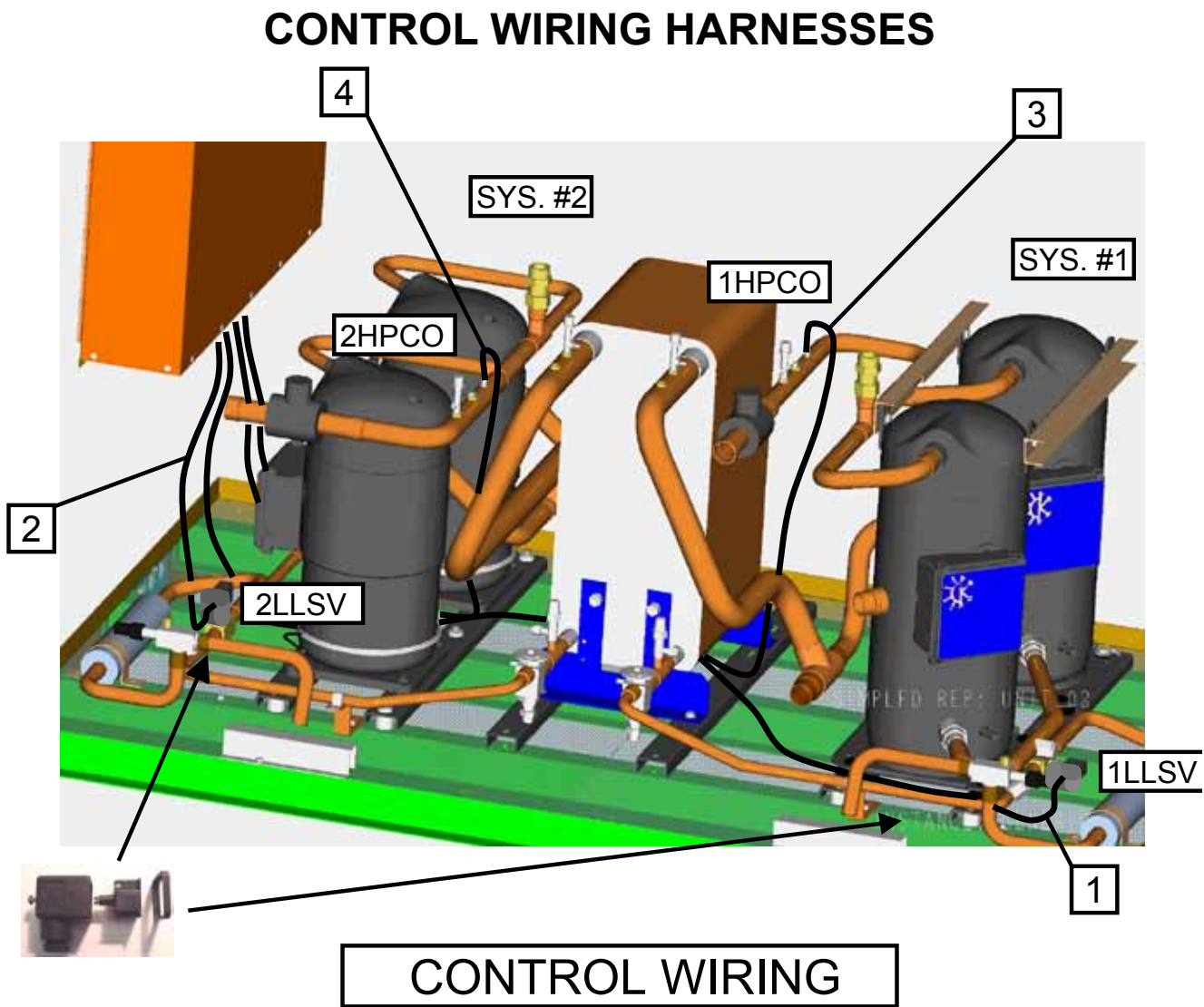
FIG. 7 – CONTROL WIRING HARNESSES (REF. TABLE 9)
