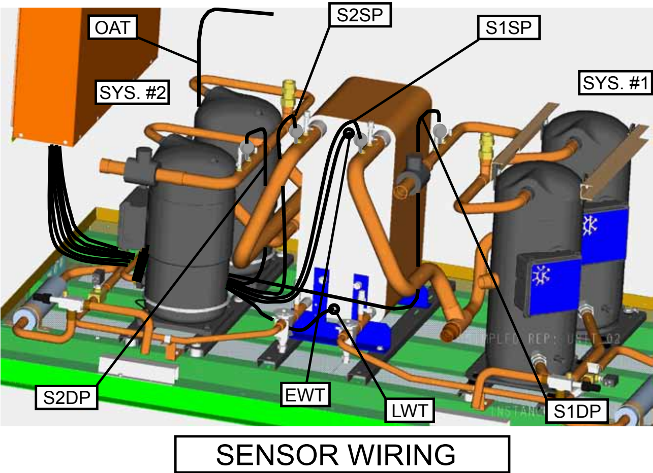
FIG. 8 – SENSOR WIRING HARNESSES (REF. TABLE 10)
