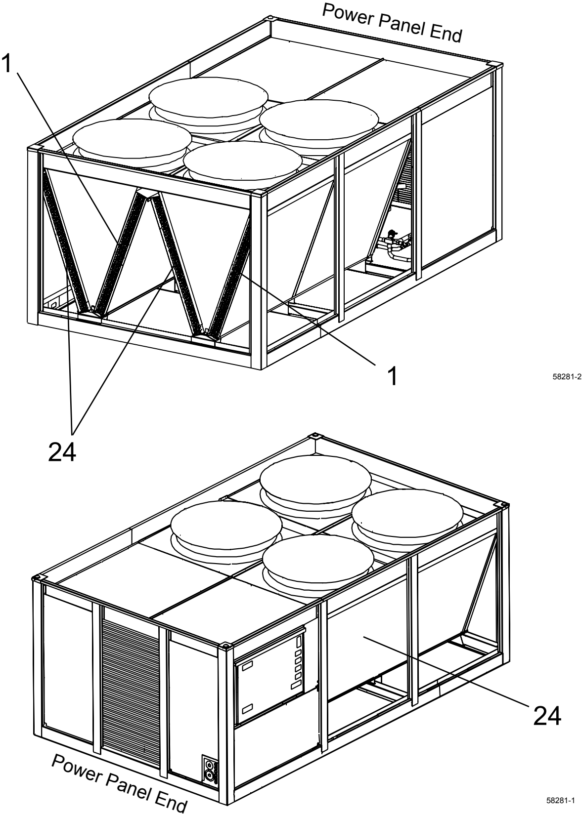
FIG. 2 – CONDENSER COIL LAYOUT (REF. TABLE 2, PAGE 9)
