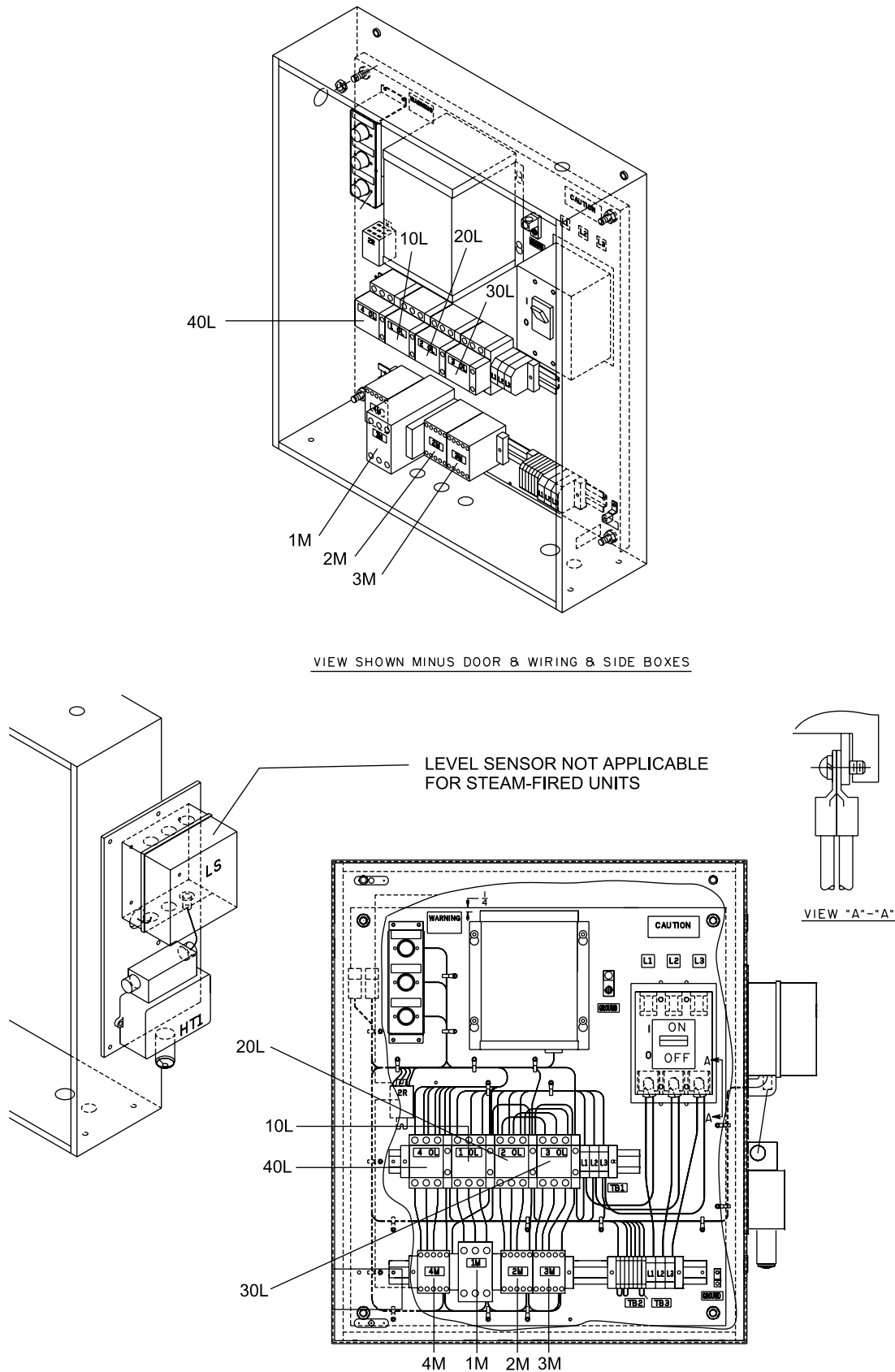
FIGURE 14 - 3 PUMP UNITS
