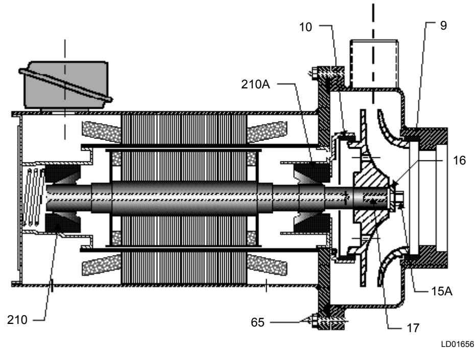
FIGURE 15 - SINGLE-ENDED PUMP
