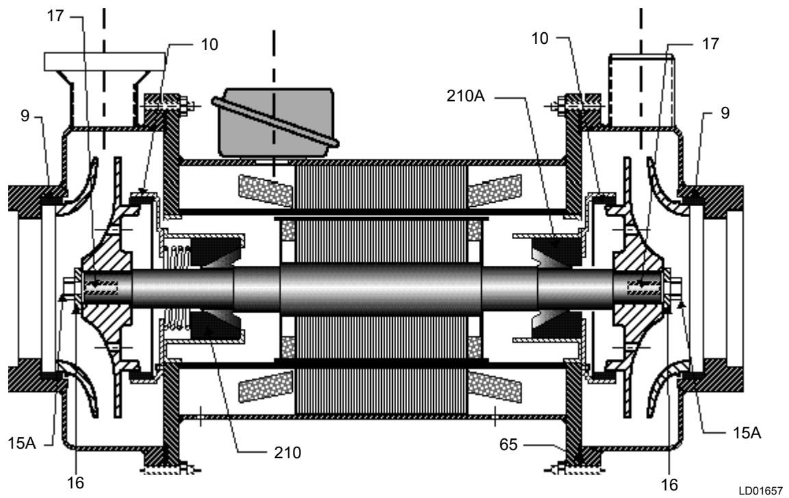
FIGURE 16 - DOUBLE-ENDED PUMP
