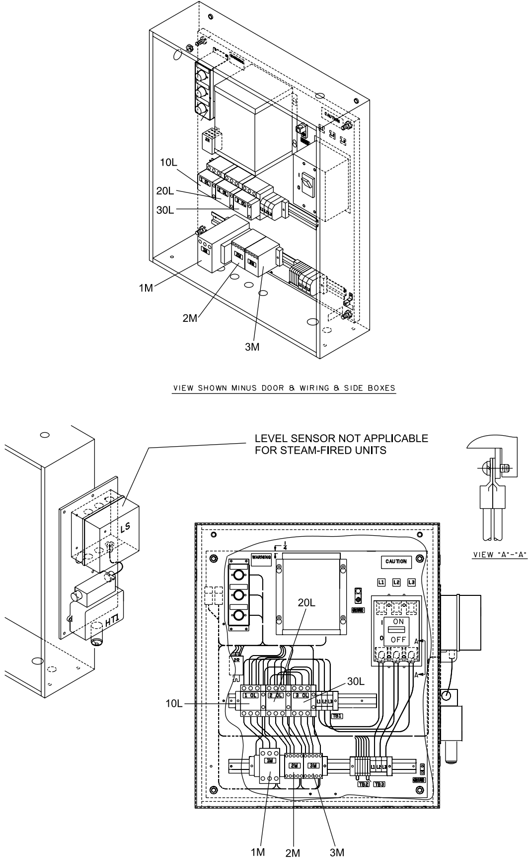
FIGURE 13 - 2 PUMP UNITS
