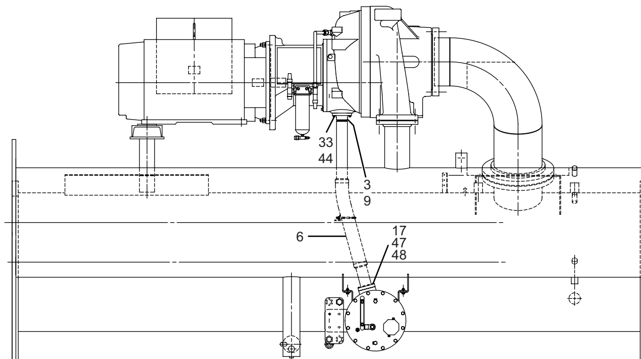
FIGURE 30 - OIL RETURN LINE
