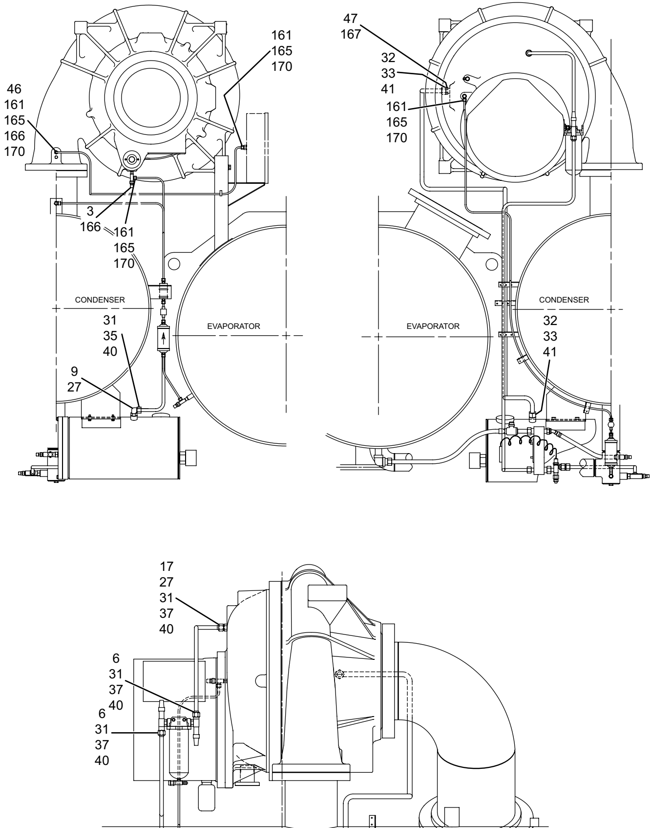
FIGURE 31 - COMPRESSOR PIPING
