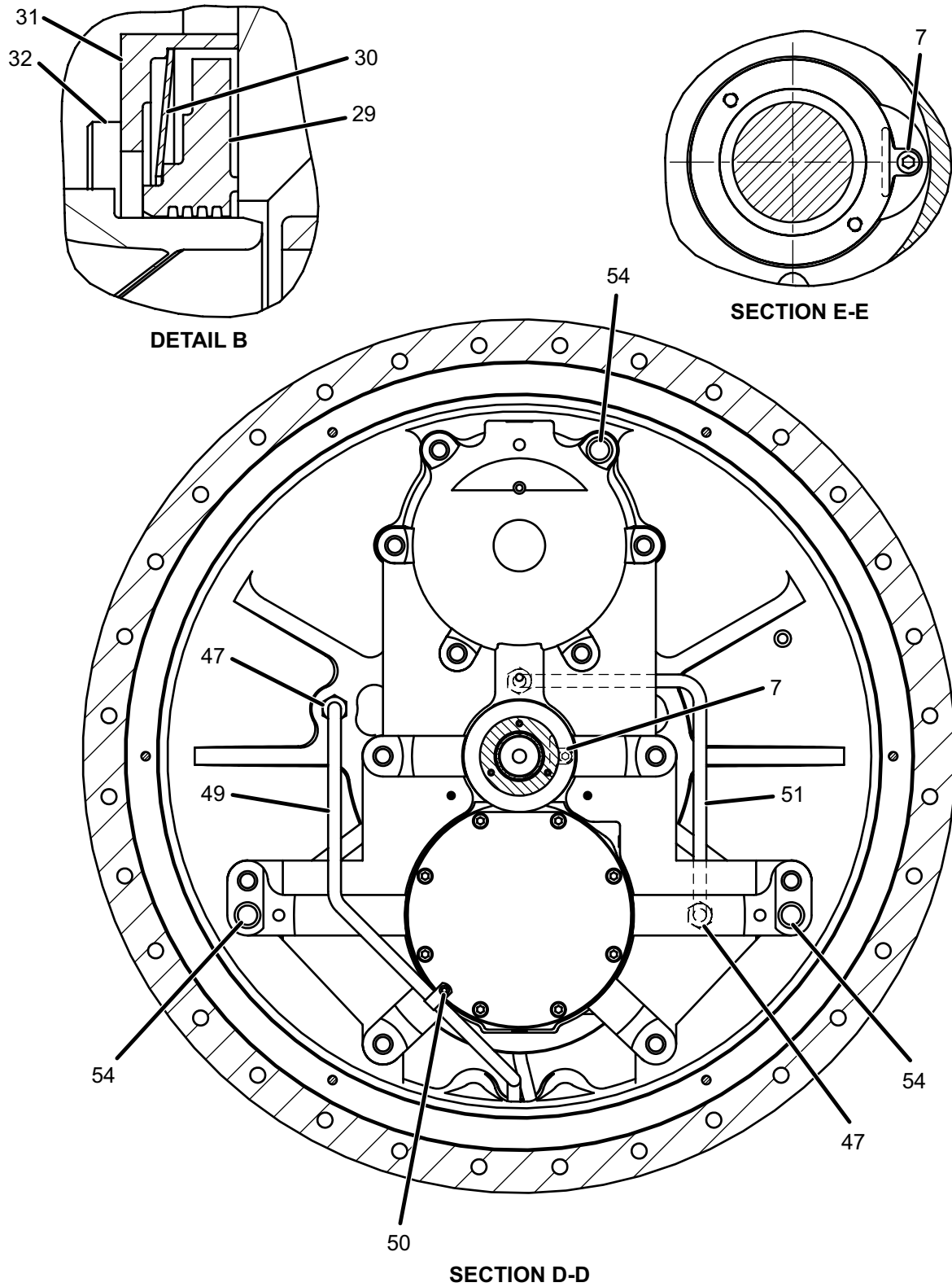
FIGURE 24 - Q7 COMPRESSOR WITH VGD
