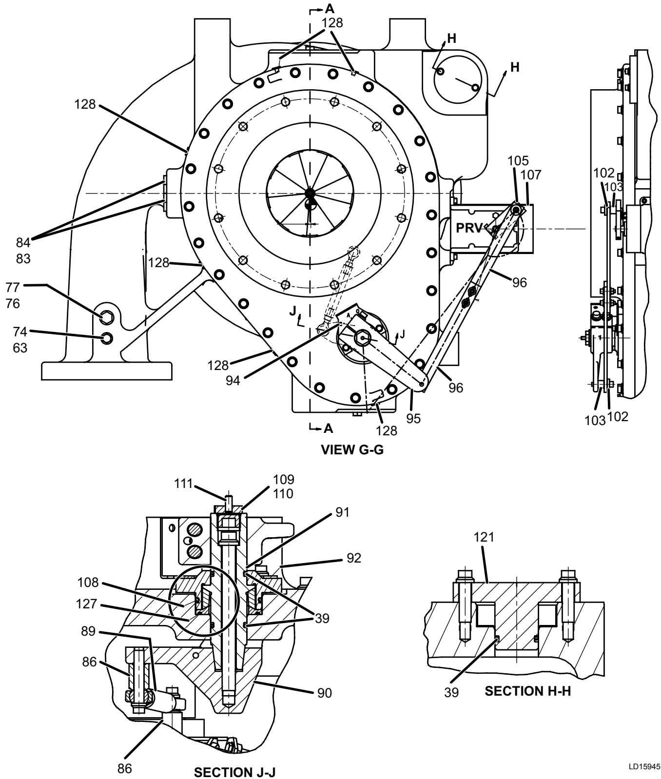
FIGURE 21 - Q7 COMPRESSOR WITHOUT VGD
