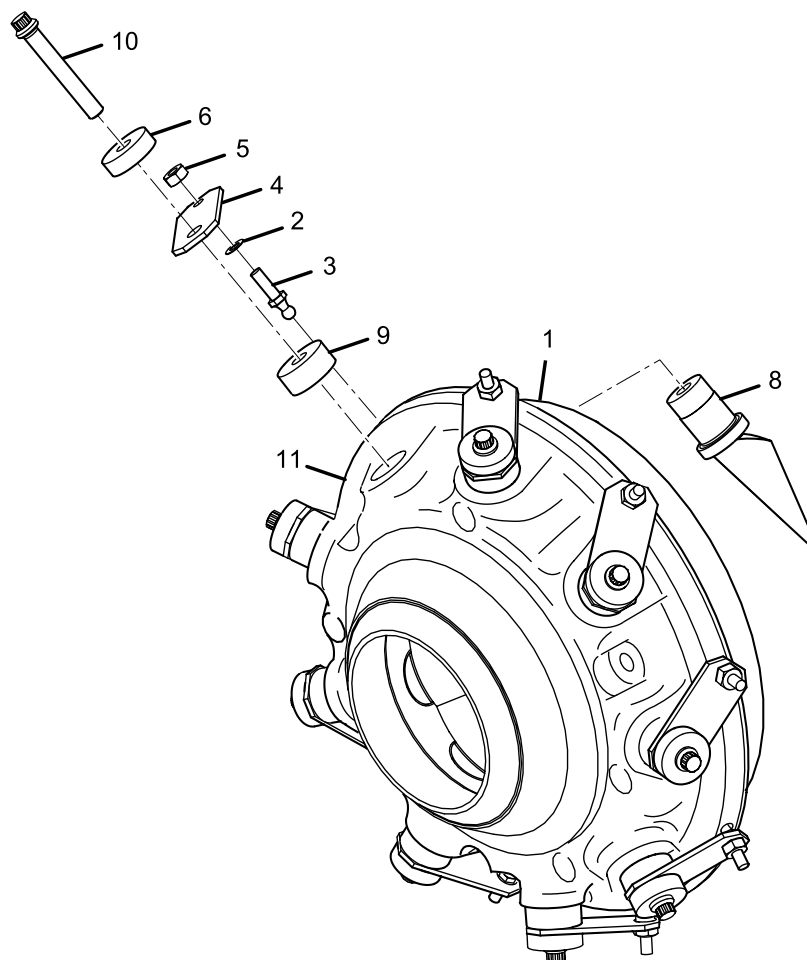
FIGURE 9 - DEVICE PRE-ROTATION
