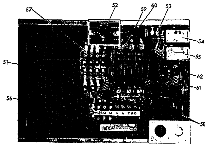
FIG. 10—Model LCH5A-25A-Control Panel
