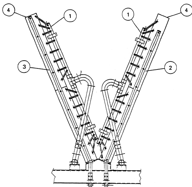
TYP. 3-ROW COIL
