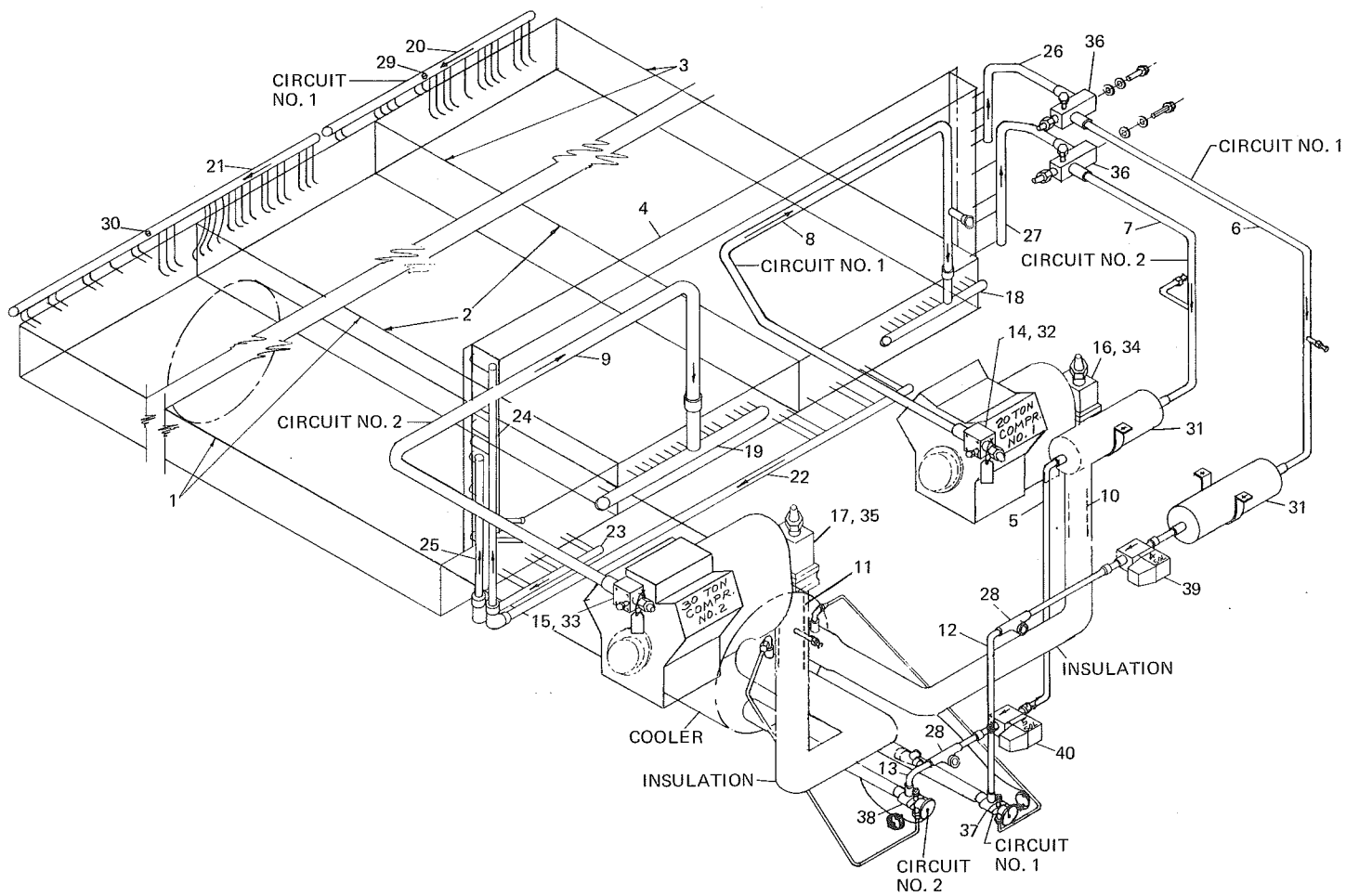
FIG. 5—REFRIGERANT PIPING
