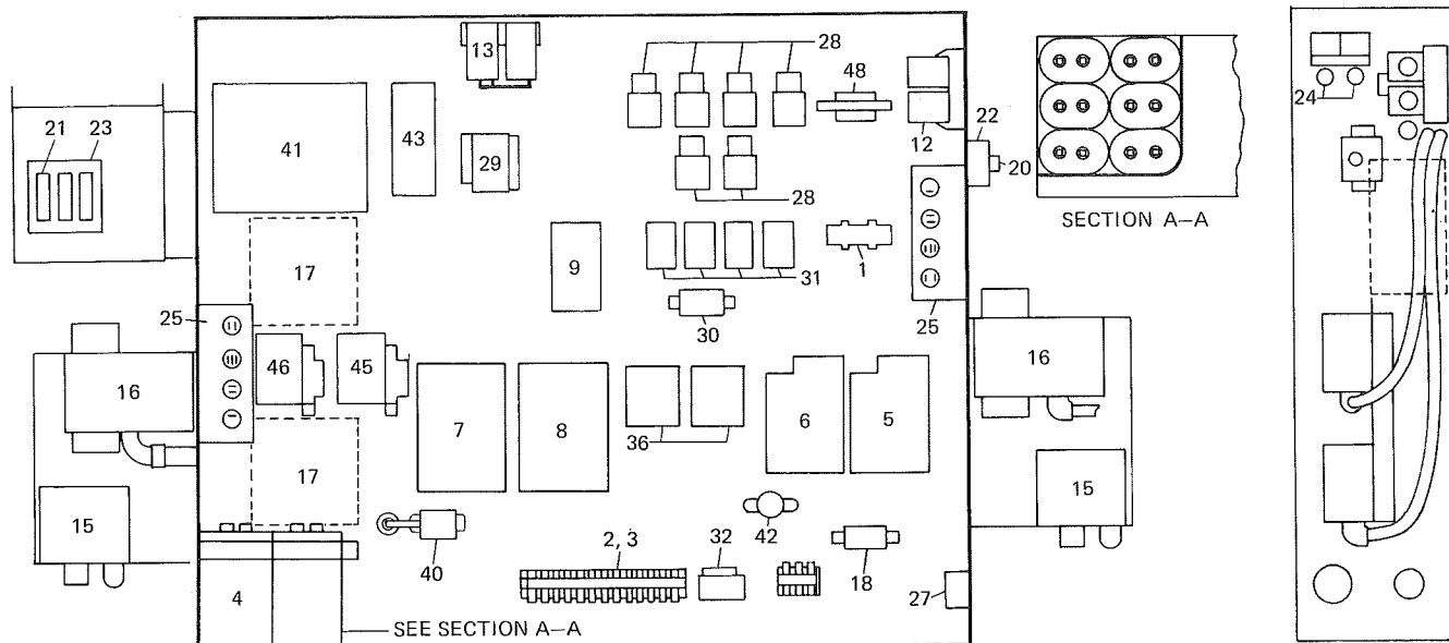
FIG. 2—MAIN CONTROL PANEL, LCHA45-25A AND -61A
