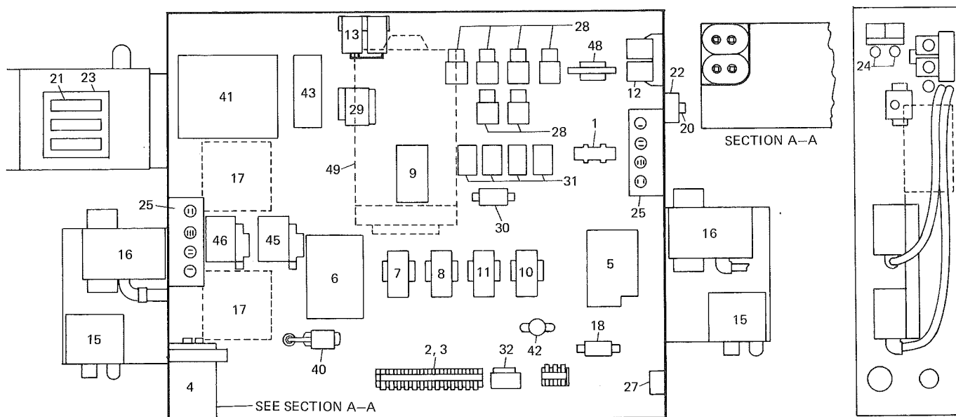
FIG. 3—MAIN CONTROL PANEL, LCHA45-46A, -58A AND -67A
