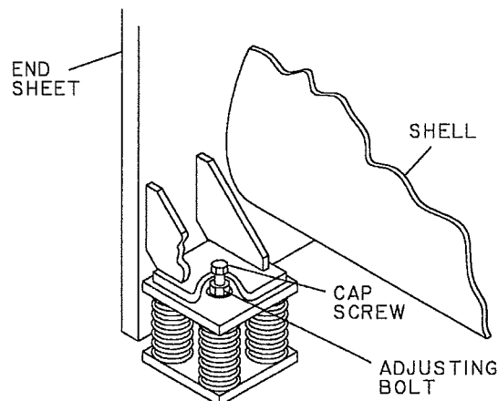
SPRING ISOLATORS
