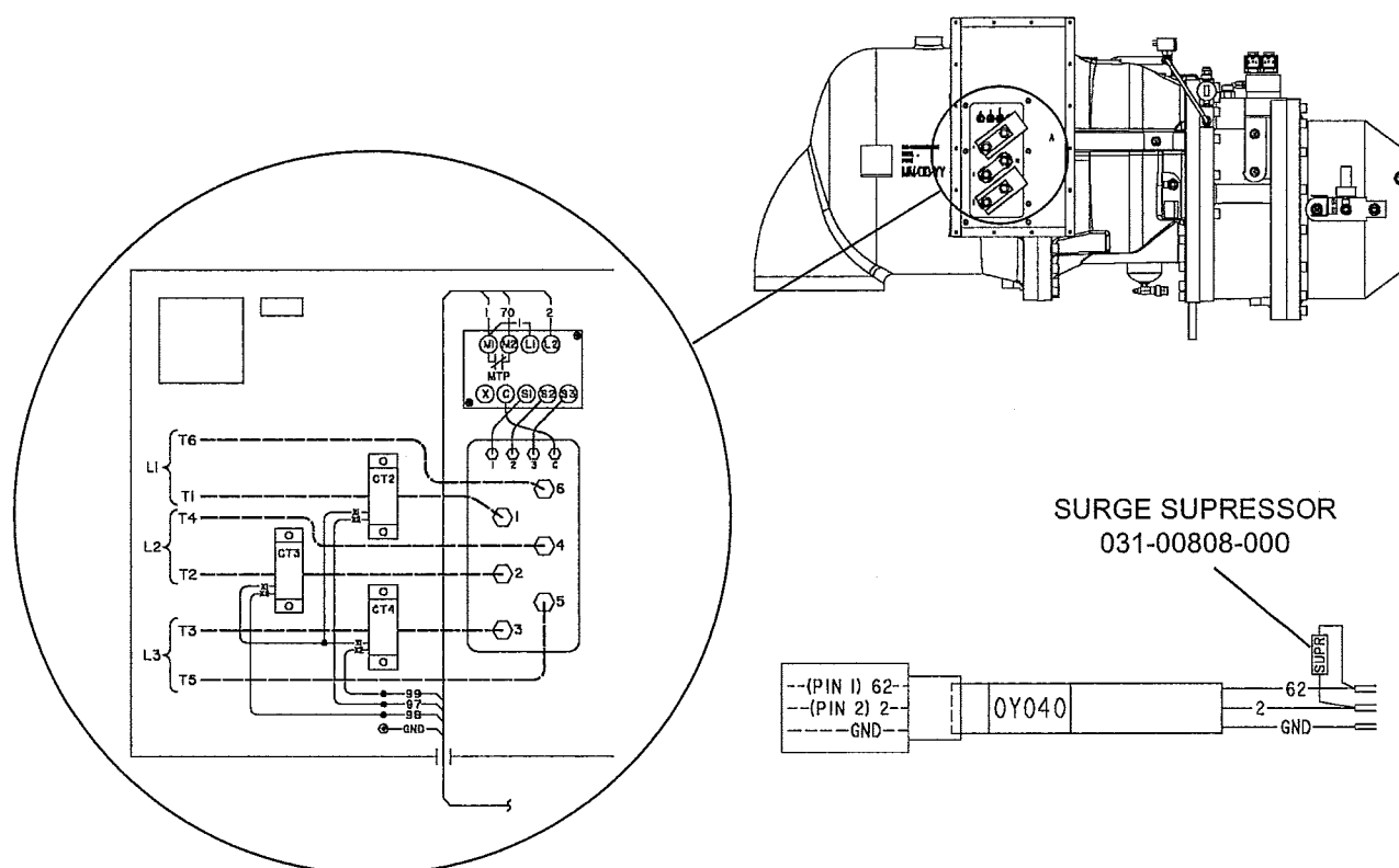
FIG. 13 - CURRENT TRANSFORMER KIT
