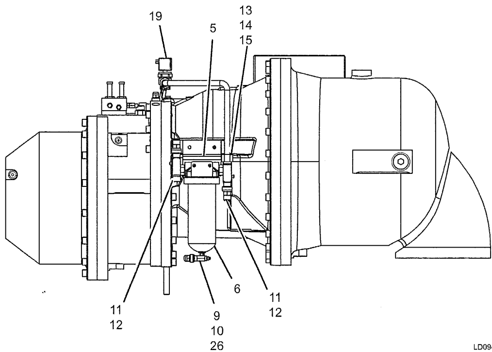
FIG. 10 - SINGLE FILTER COMPRESSOR COMPONENTS
