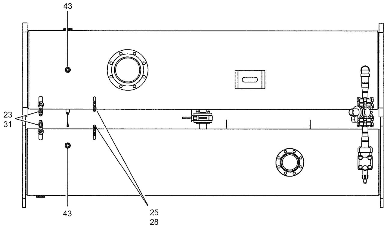
FIG. 5 - VARIABLE ORIFICE / HOT GAS BYPASS
