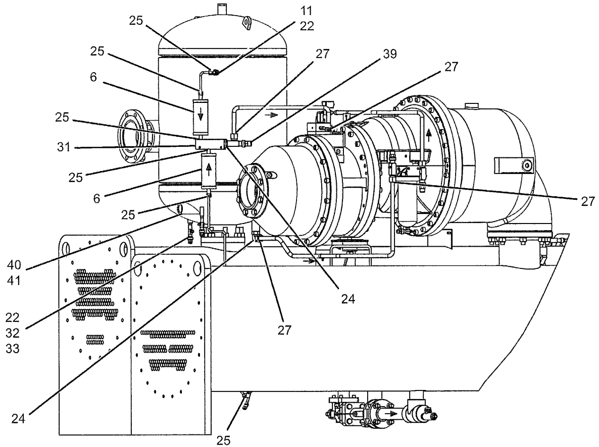
FIG. 2 - UNIT PIPING
