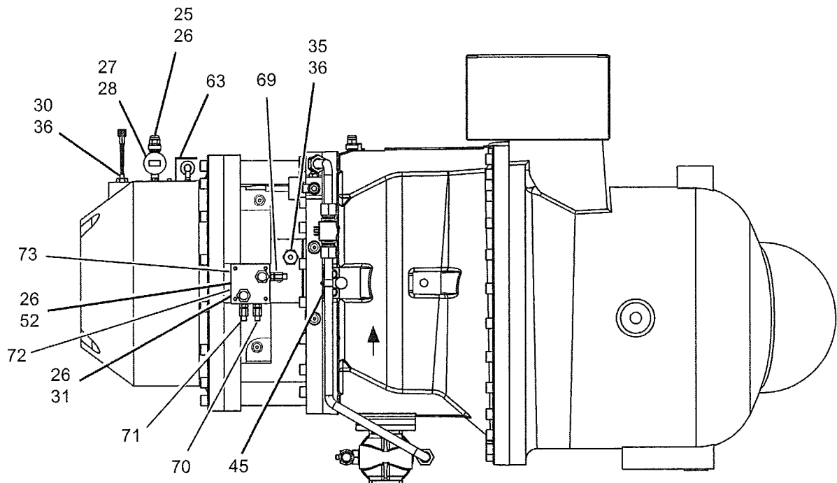
FIG. 8 - SINGLE FILTER COMPRESSOR COMPONENTS
