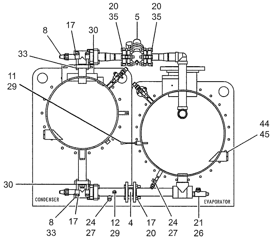
FIG. 5 - VARIABLE ORIFICE / HOT GAS BYPASS
