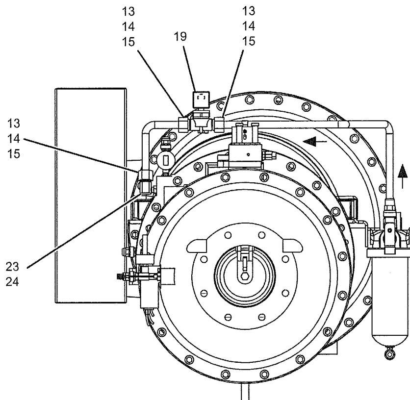
FIG. 9 - SINGLE FILTER COMPRESSOR COMPONENTS
