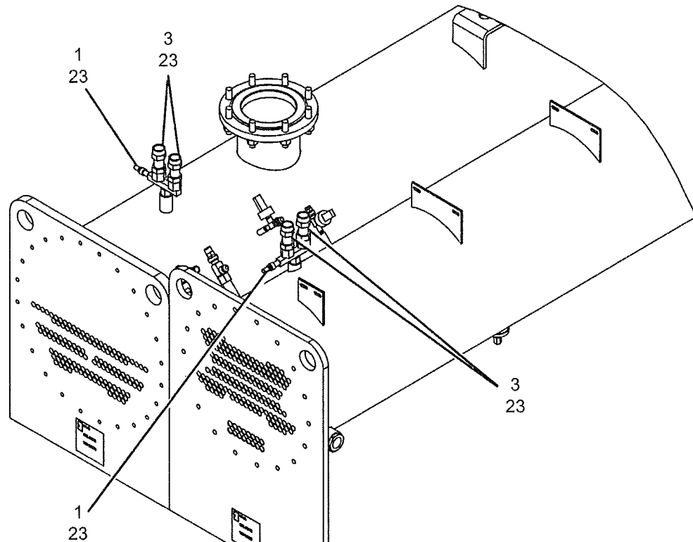
FIG. 3 - OPTIONAL DUAL RELIEF VALVES
