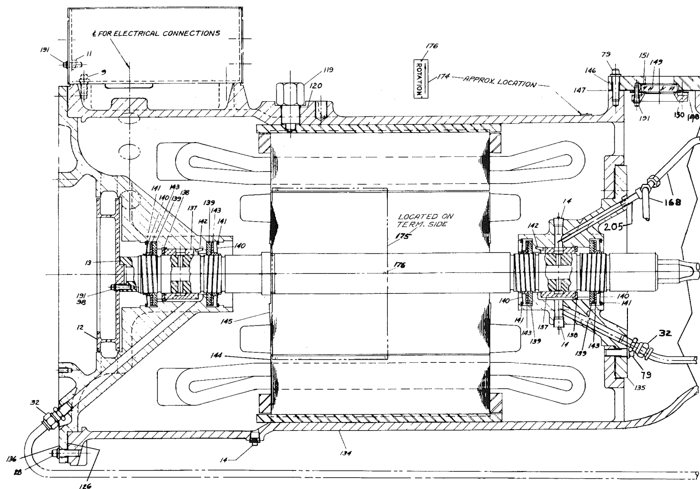
FIG. 1- Cross Section View of Compressor - Hermetic
