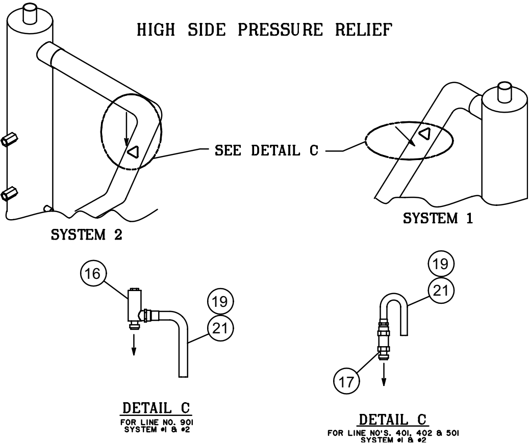
FIG. 5 – RELIEF VALVES AND CUTOUT SWITCHES (REF. TABLE 5)
