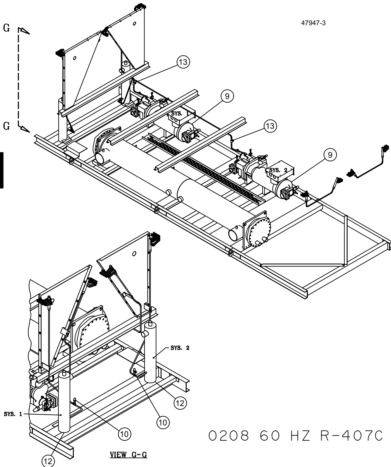
FIG. 4 – REFRIGERANT PIPING COMPONENTS - MODEL YCAS0208 SHOWN (REF. TABLE 4)
