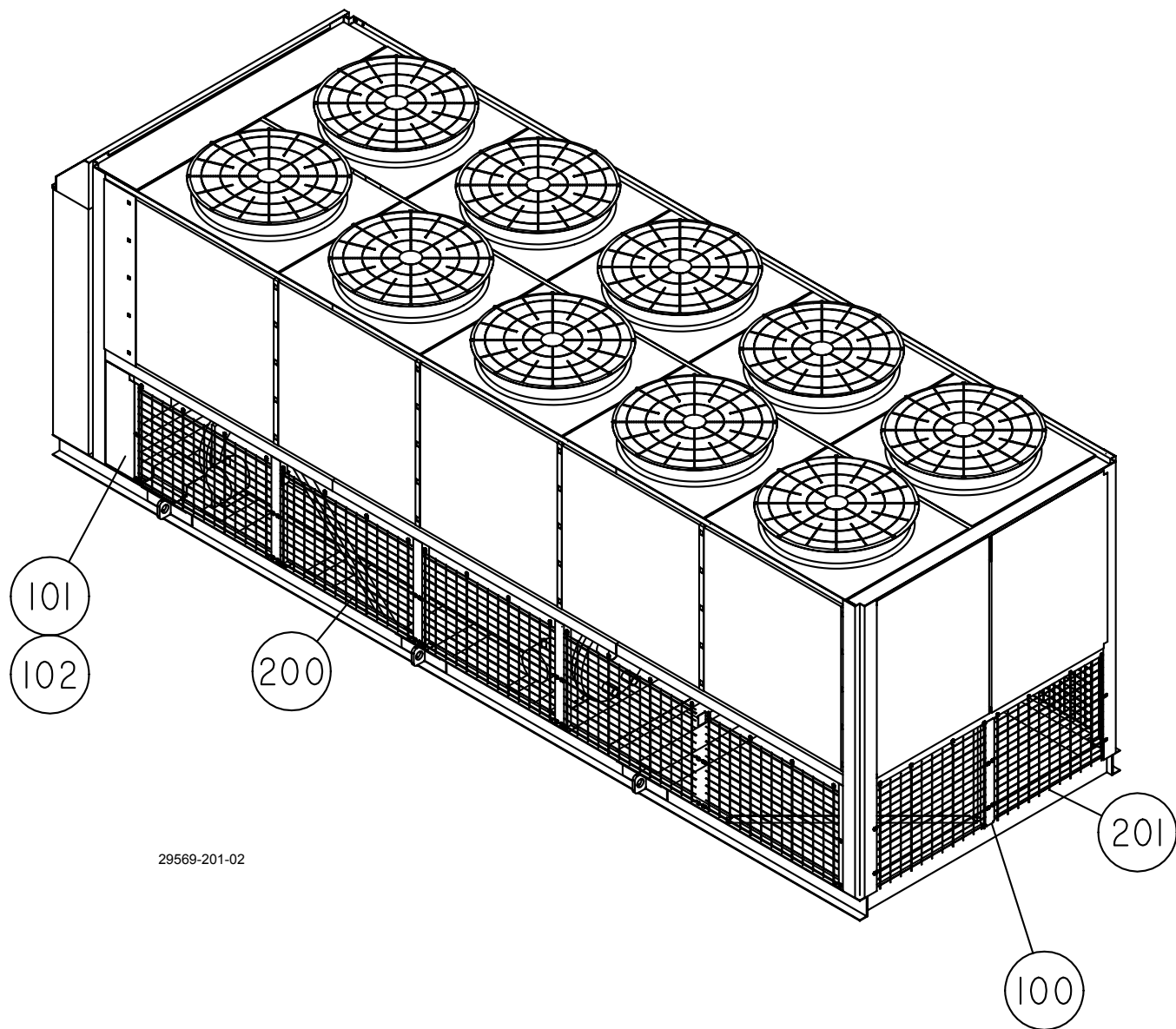
FIG. 20 – WIRE ENCLOSURE (BOTTOM SECTIONS) - 375-29569-201 SHOWN (REF. TABLE 21)
