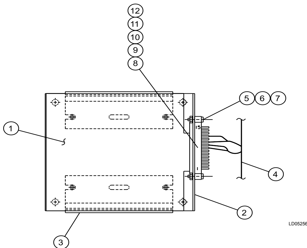
FIG. 24 – REMOTE CURRENT/TEMPERATURE RESET COMPONENTS
