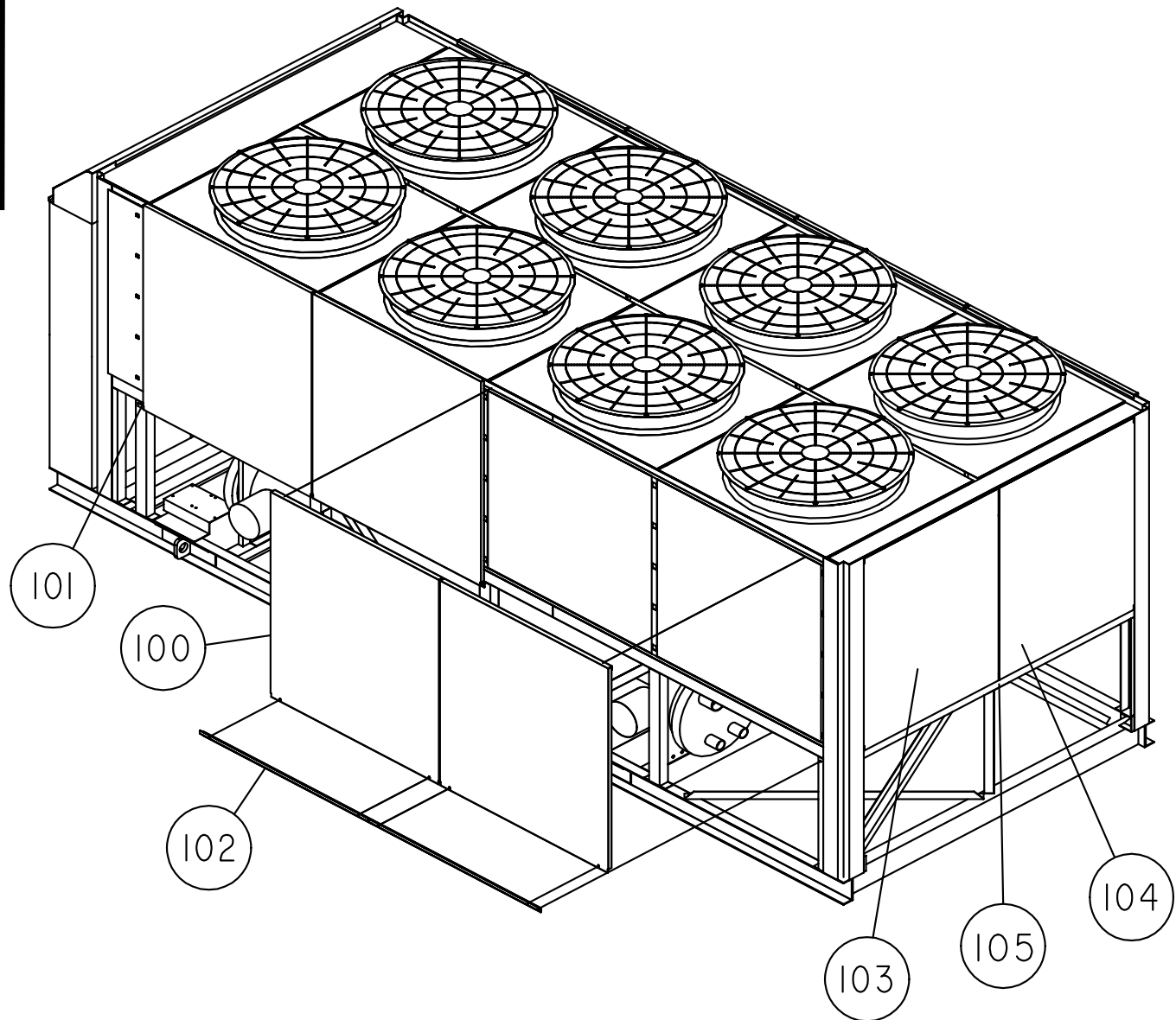
FIG. 21 – LOUVERED ENCLOSURE (TOP SECTIONS) - 375-29571-160 SHOWN (REF. TABLE 22)
