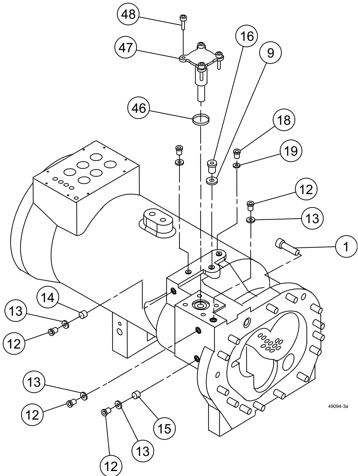
FIG. 6a – 124MM, 136MM & 145MM DXS COMPRESSOR COMPONENTS PARTIAL EXPLODED VIEW (REF. TABLE 7)
