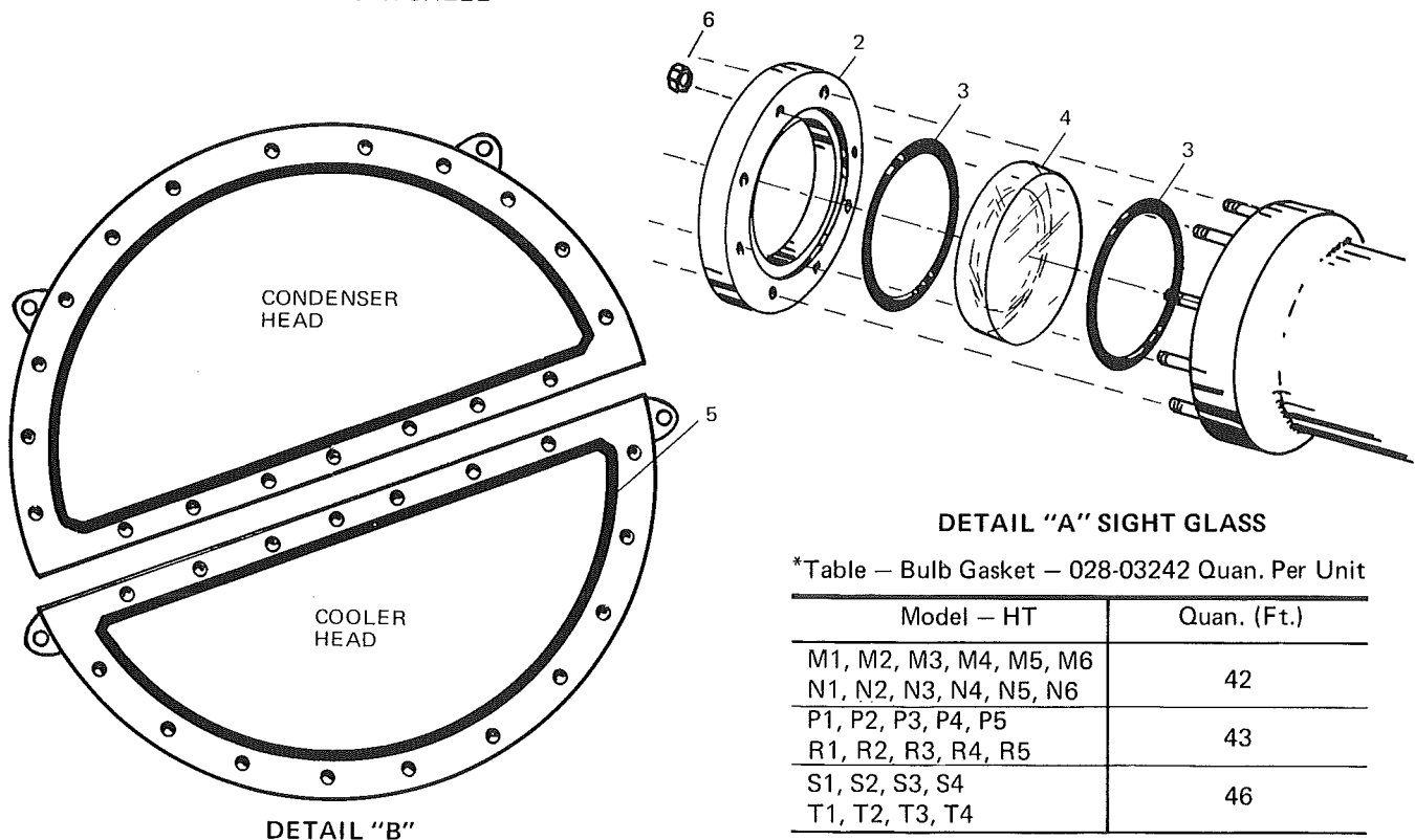
FIG. 1—COOLER-CONDENSER SHELL
