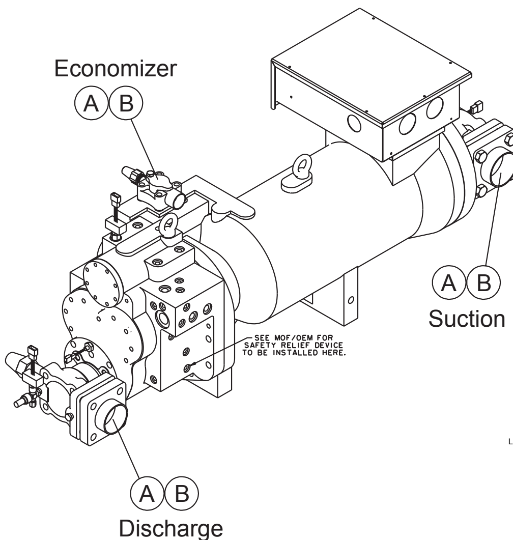
FIG. 8 – COMPRESSOR AND CONTROL COMPONENTS (REF. TABLE 9)
