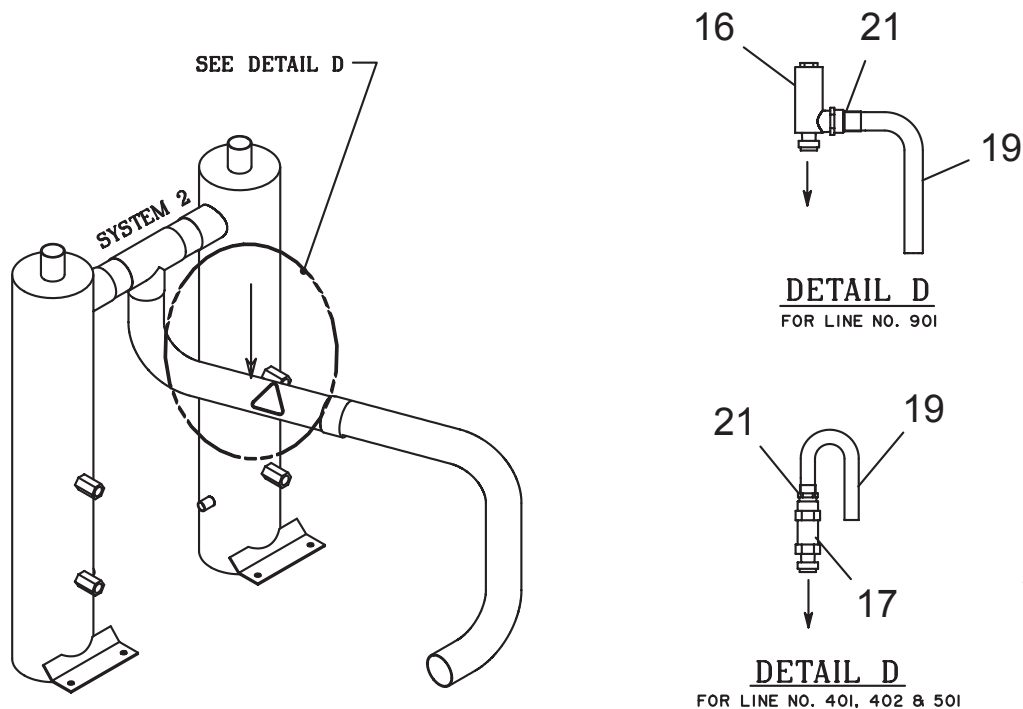
FIG. 6 – RELIEF VALVES AND CUTOUT SWITCHES (REF. TABLE 6, PAGE 25)
