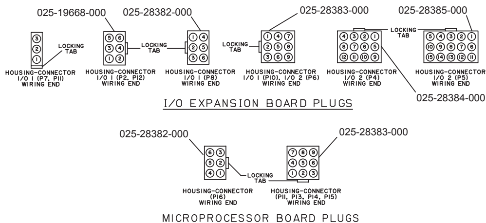
FIG. 16B – SENSOR HOUSING PART NUMBERS
