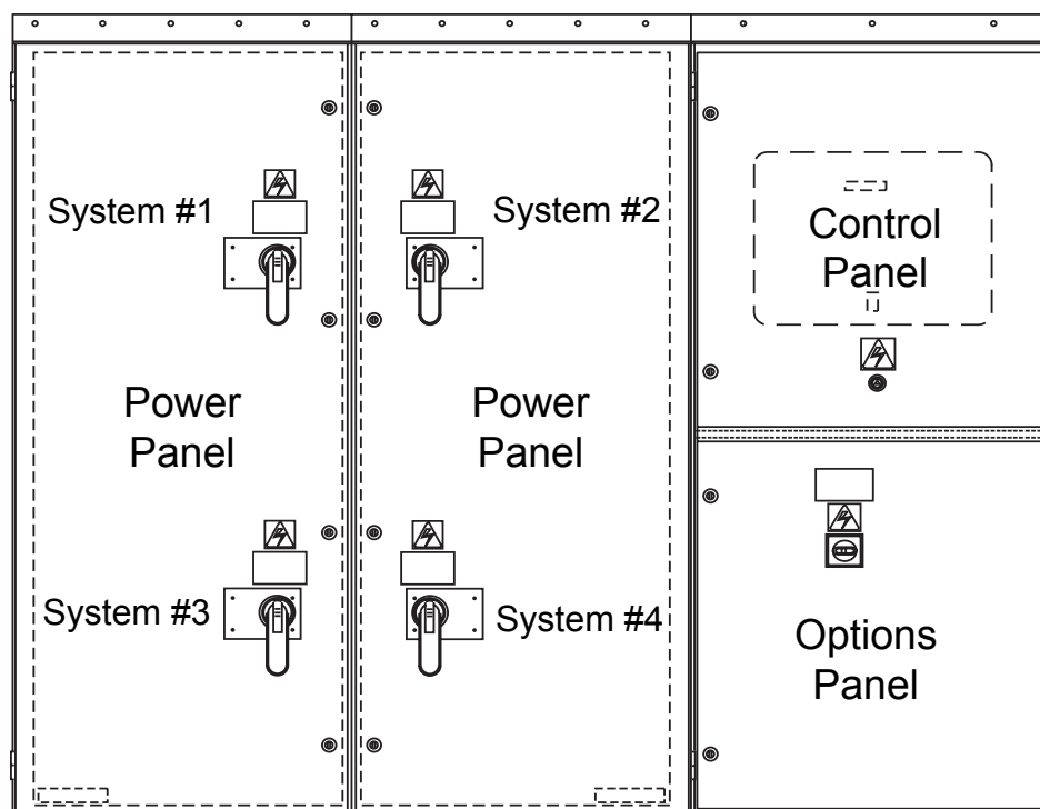
FIG. 10 – CONTROL, OPTIONS AND POWER PANELS LAYOUT
