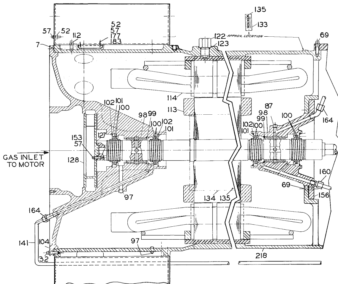
FIG. 1 - Cross Section View of Compressor - Hermetic
