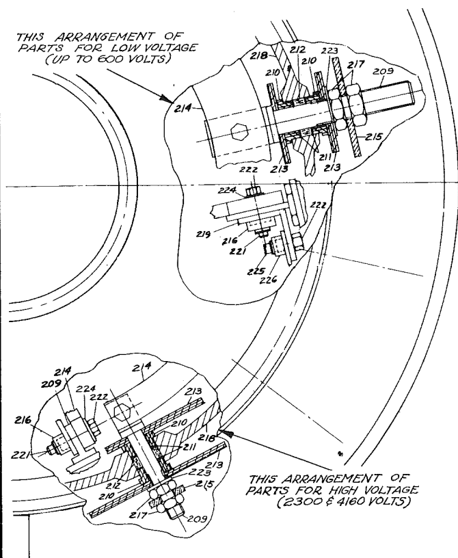
FIG. 6- Motor Terminals
