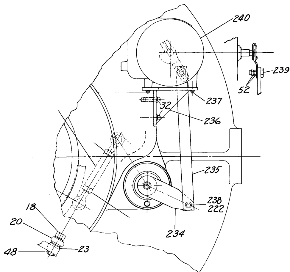
FIG. 8- Electric Motor
