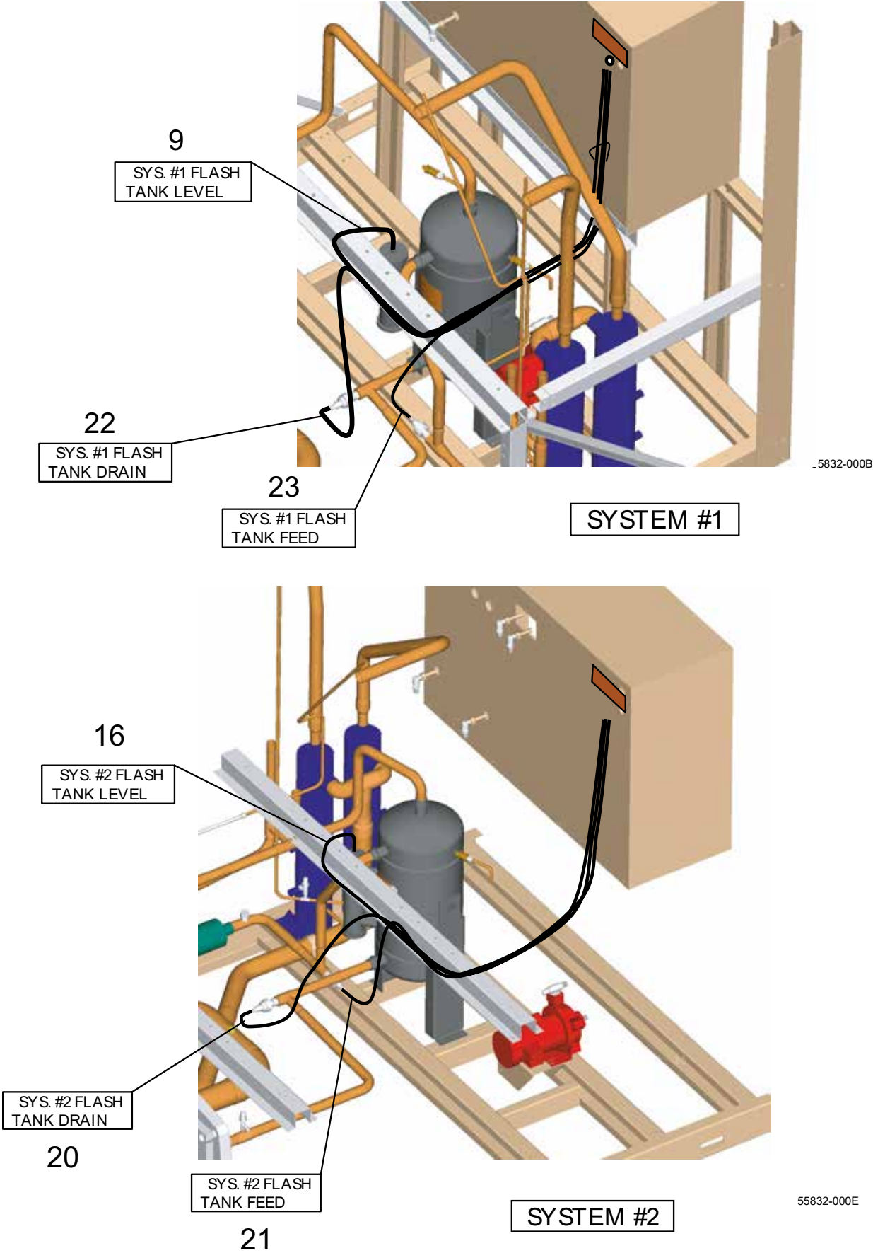
FIG. 12C – HARNESS LAYOUT (REF. TABLE 13, PAGES 52, 53 AND 54)
