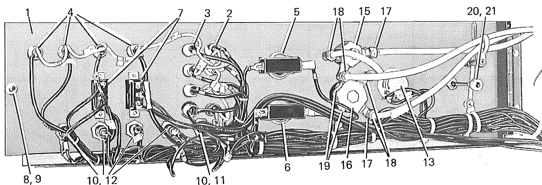
FIG. 3 — CENTER PANEL PARTS (MOTOR DRIVE)
