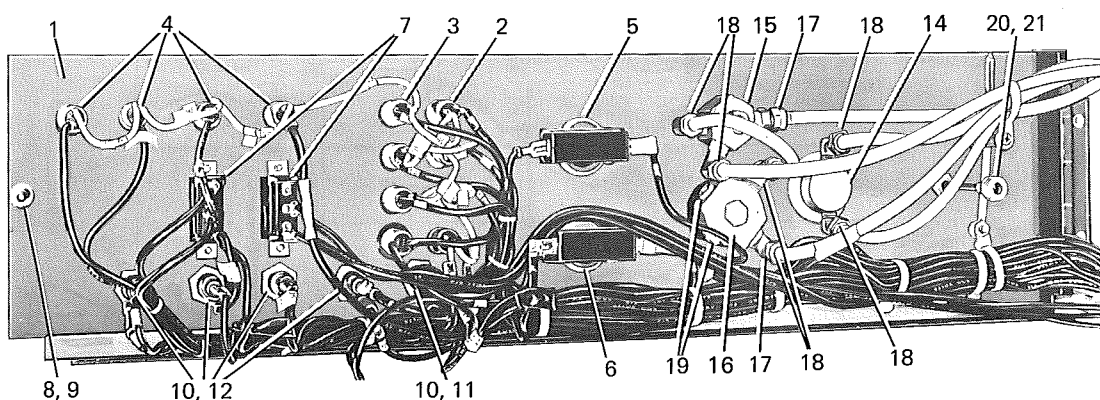
FIG. 4 — CENTER PANEL PARTS (TURBINE DRIVE)
