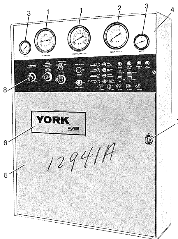
FIG. 2 — TURBINE DRIVE - PART NO'S. 366-56226 & 366-55225
