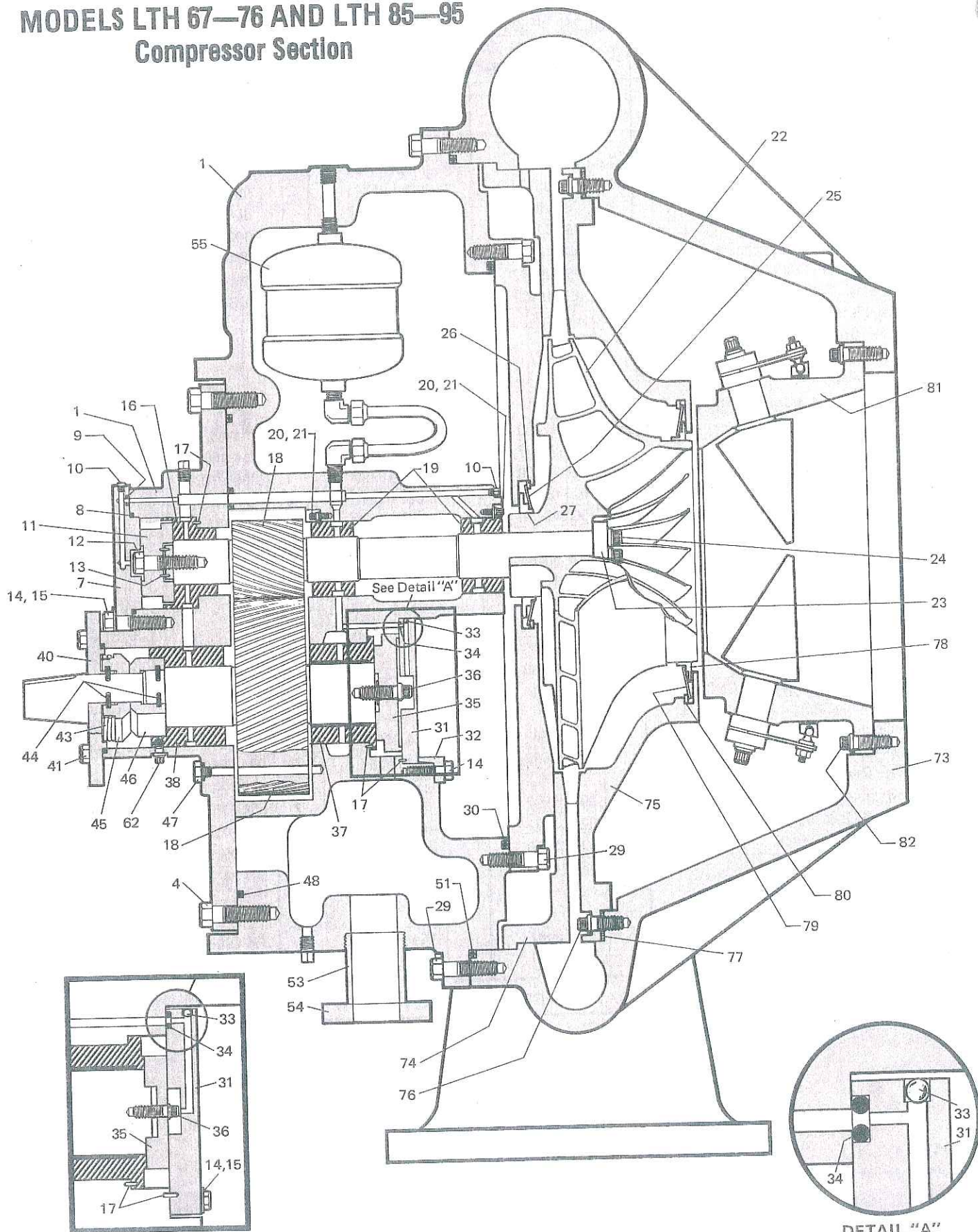
FIG. 2 — CUTAWAY VIEW — LTH 67, 76, 85 AND 95
