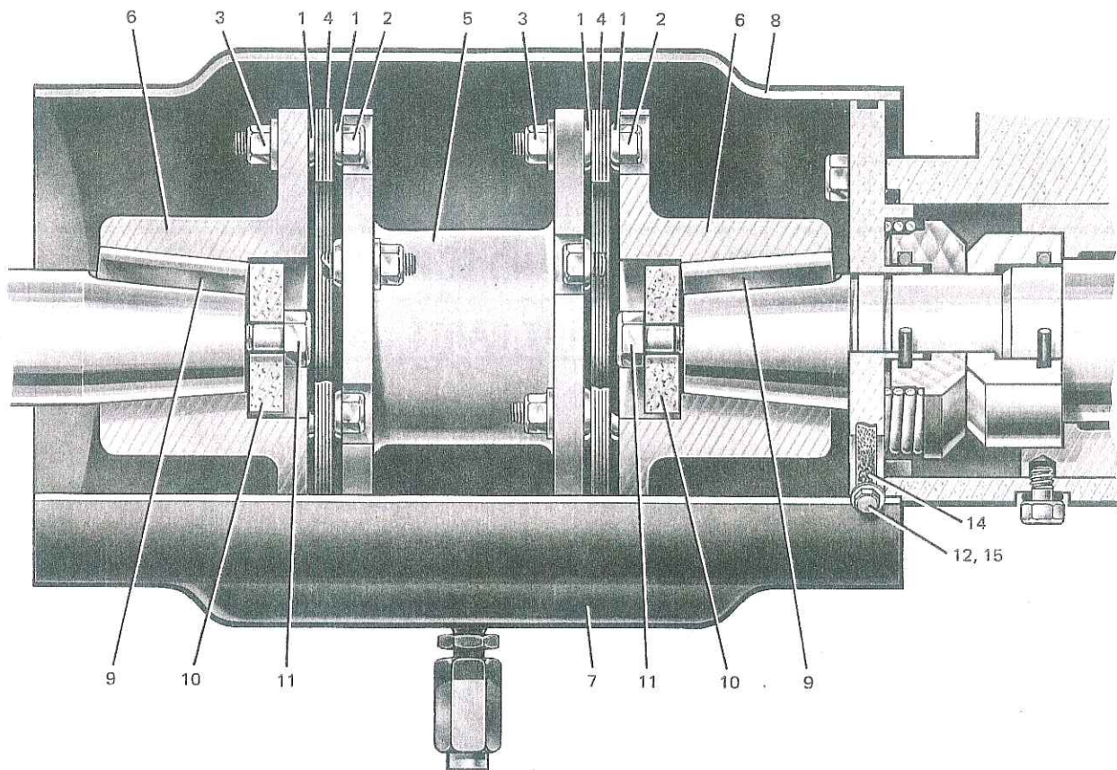
FIG. 22 — COUPLING OPEN TYPE — MODELS LTH 67, 76, 85 AND 95
