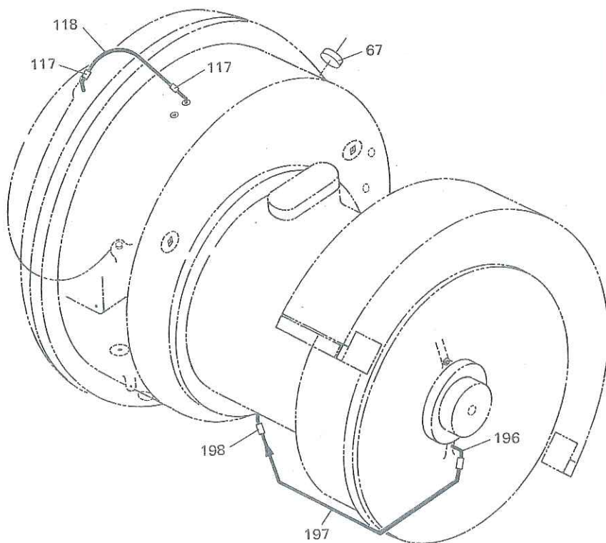
FIG. 15 — HERMETIC COMPRESSOR—MODELS MTH 85 AND 95
