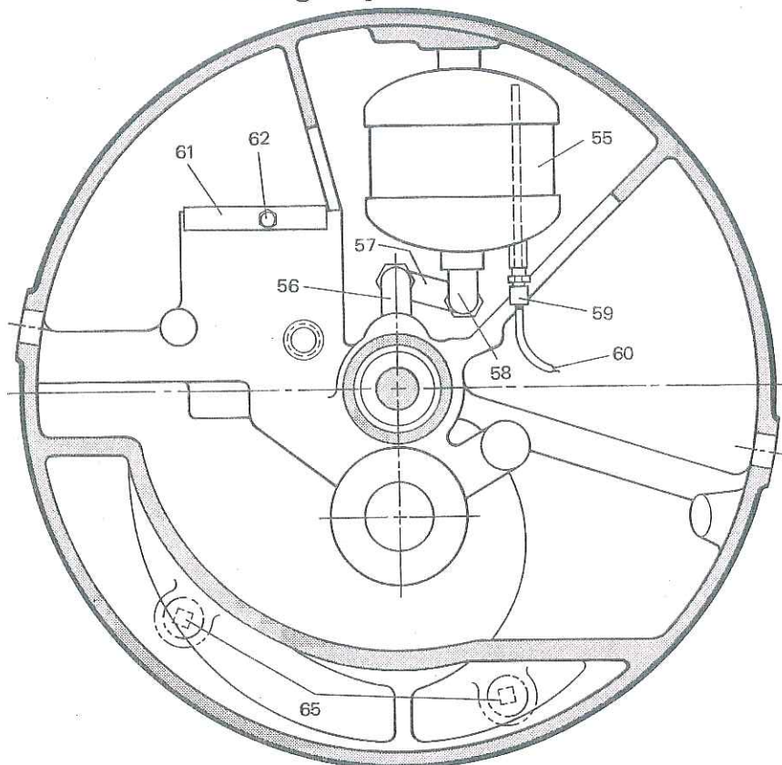
FIG. 3 — EMERGENCY OIL RESERVOIR — MODELS MTH/LTH 67 OR 76
