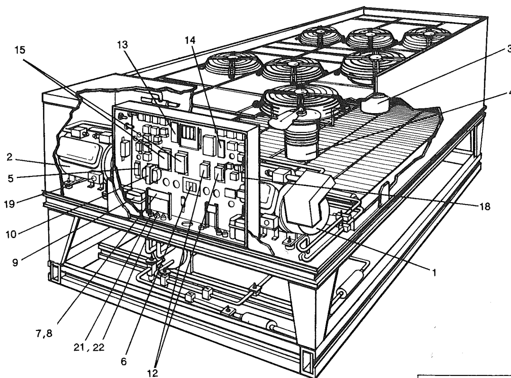
FIG. 1 - AIR COOLED WATER CHILLER
