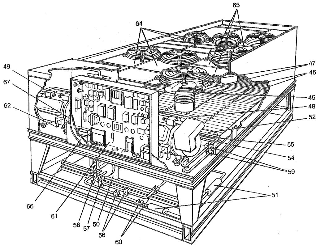
FIG. 3 - AIR COOLED WATER CHILLER
