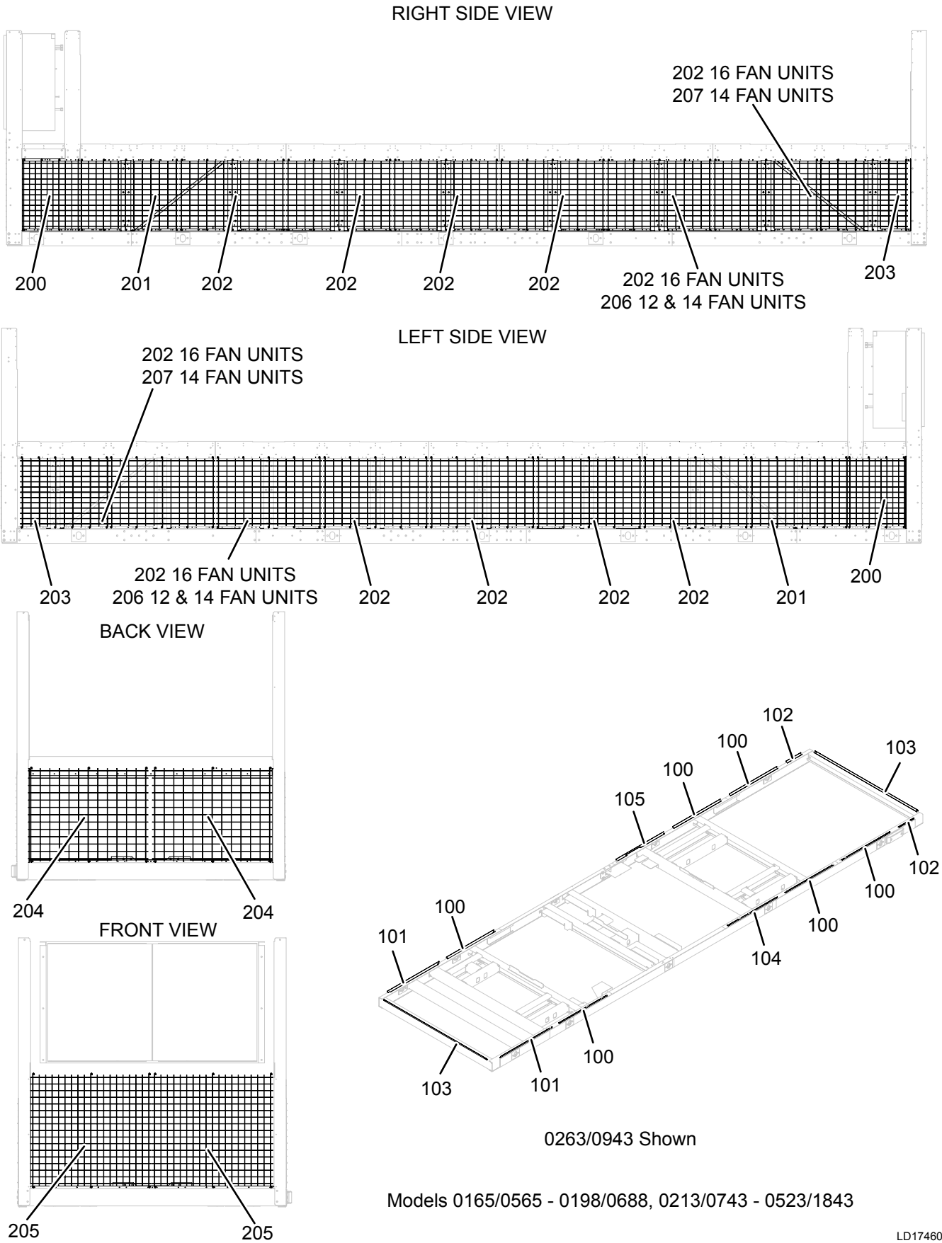
FIGURE 101 - WIRE ENCLOSURE KIT COMPONENTS - MODELS 0165/0565 - 0198/0688, 0213/0743 - 0523/1843
