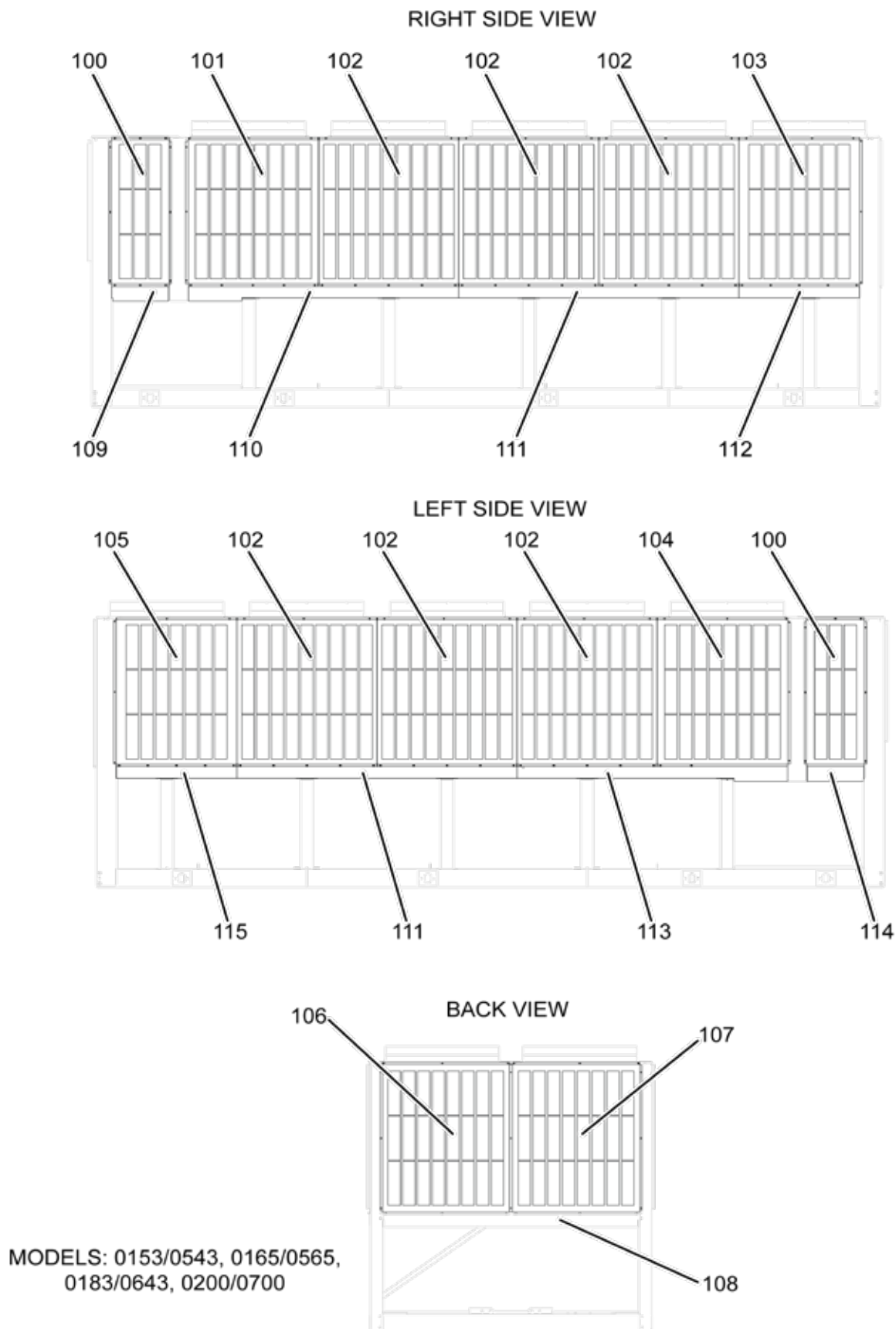
FIGURE 68 - TOP SECTION: LOUVERED ENCLOSURE KIT COMPONENTS - MODELS 0153/0543, 0165/0565, 0183/0643 AND 0200/0700
