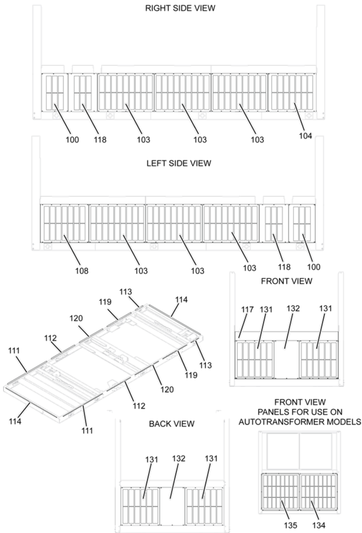
FIGURE 76 - BOTTOM SECTION: LOUVERED ENCLOSURE KIT COMPONENTS - MODEL 0200/0700
