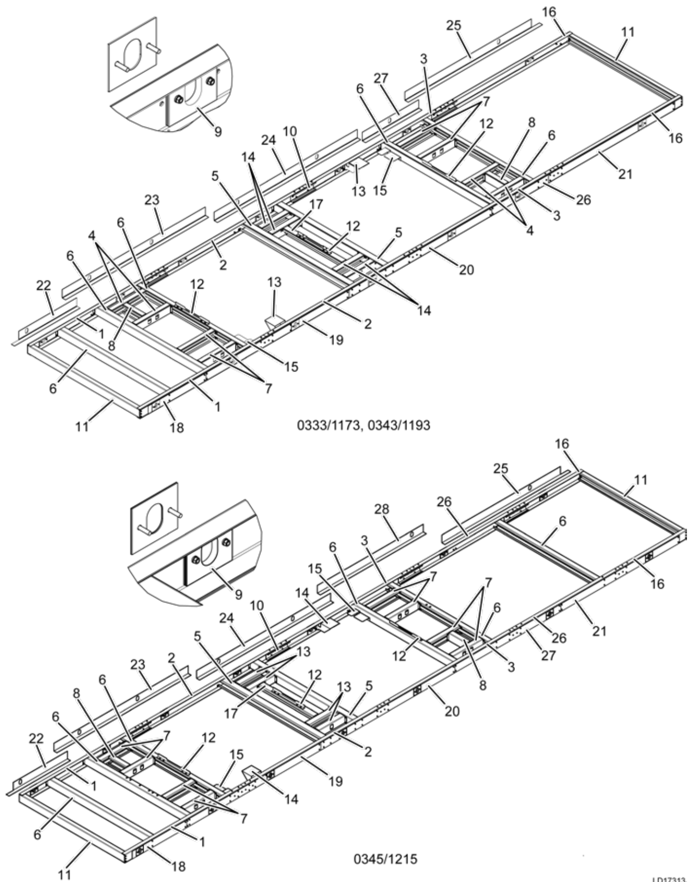
FIGURE 20 - BASE ASSEMBLY (0333/1173, 0343/1193, 0345/1215)
