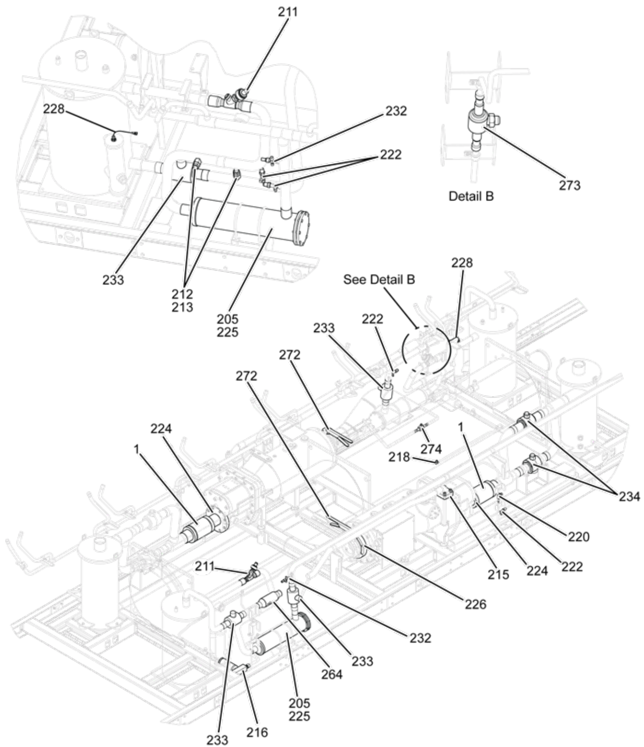
FIGURE 60 - PIPING ASSEMBLY 0475 / 1665
