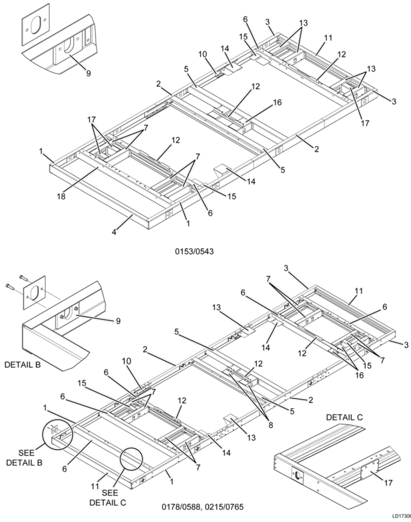
FIGURE 13 - BASE ASSEMBLY (0153/0543, 0178/0588, 0215/0765)
