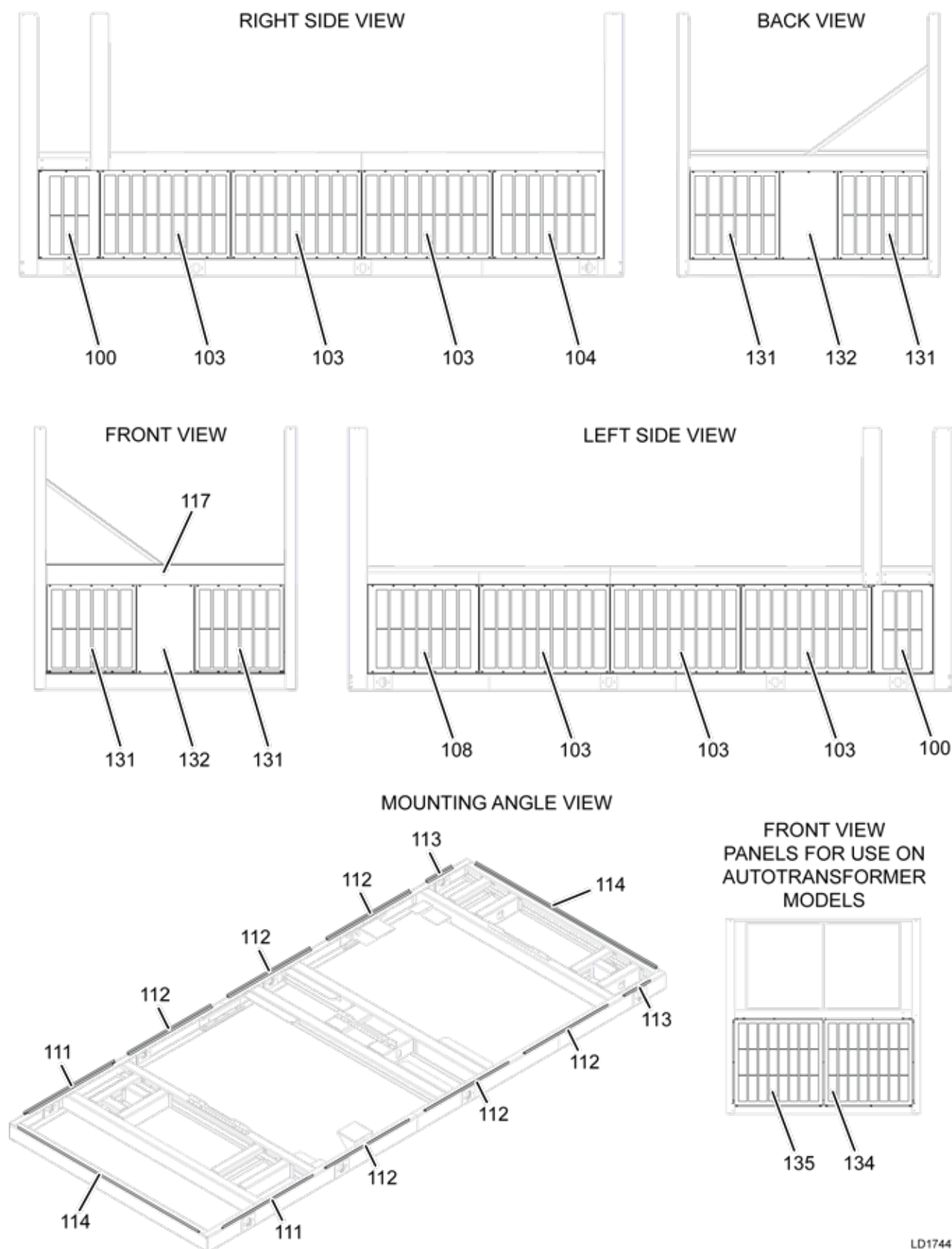
FIGURE 74 - BOTTOM SECTION: LOUVERED ENCLOSURE KIT COMPONENTS - MODEL 0153/0543
