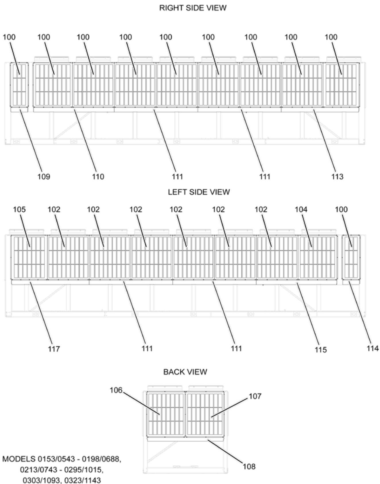
FIGURE 86 - LOUVERED ENCLOSURE (COND. ONLY) MODEL 0153/0543 - 0198/0688, 0213/0743 - 0295/1015, 0303/1093, 0323/1143
