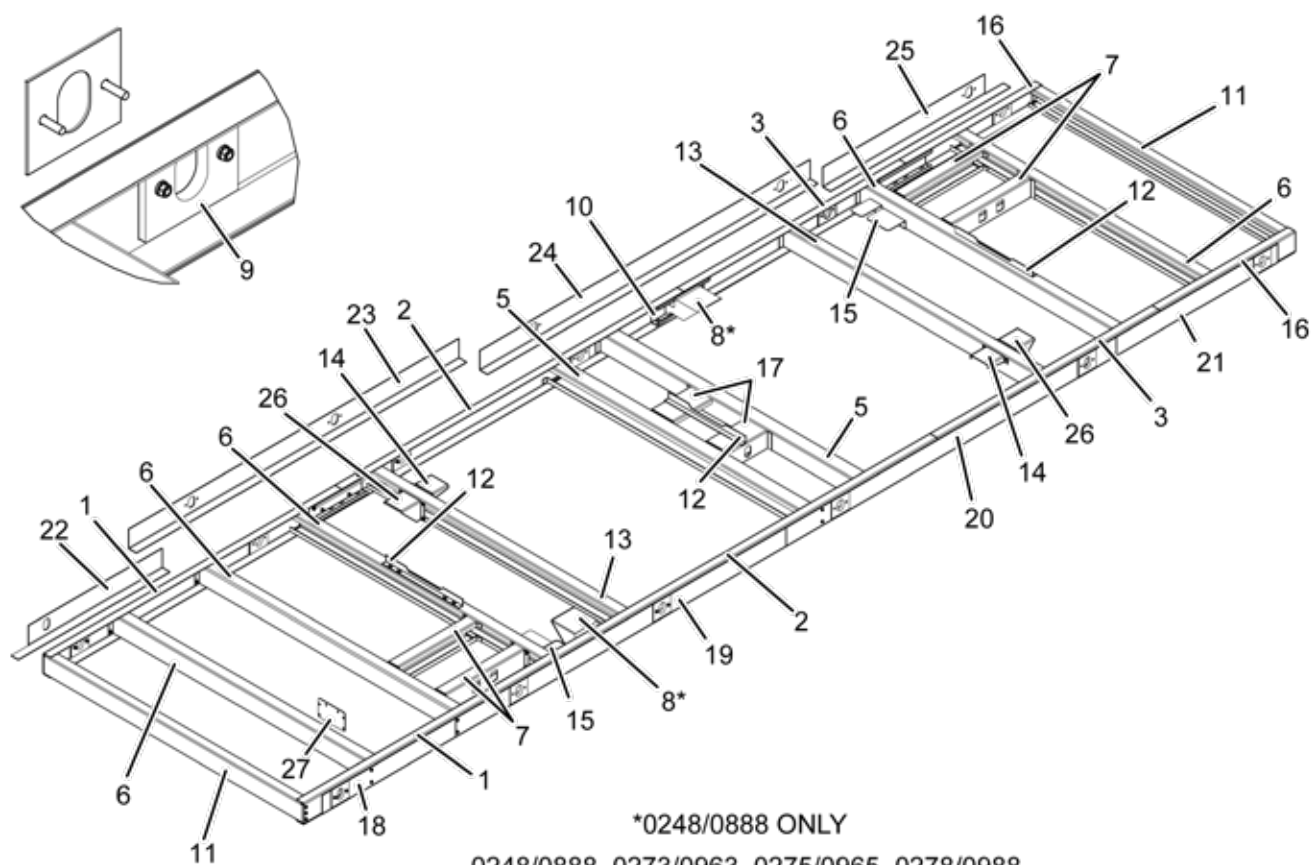
FIGURE 16 - BASE ASSEMBLY (0233/0843, 0248/0888, 0273/0963, 0275/0965, 0278/0988)
