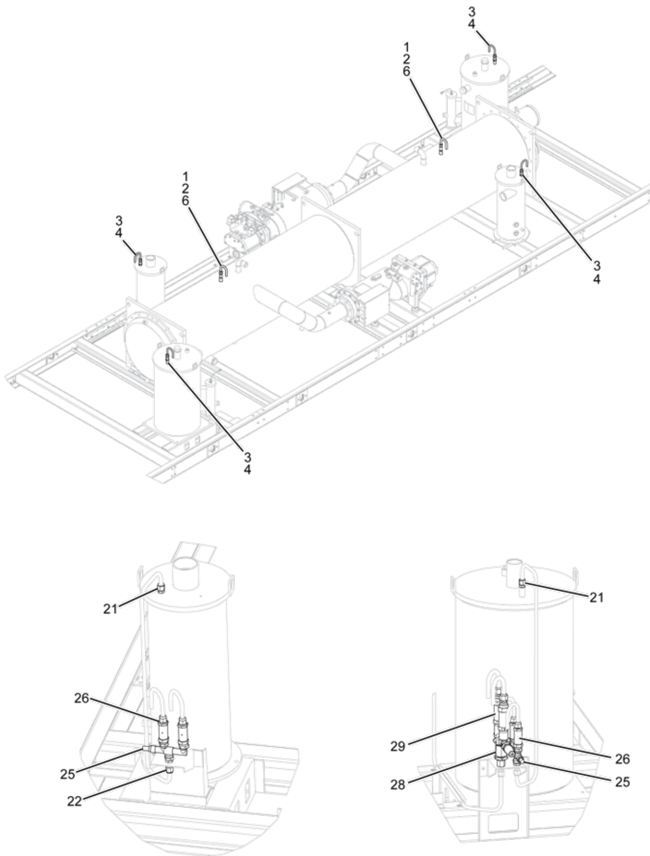
FIGURE 98 - PRESSURE RELIEF
