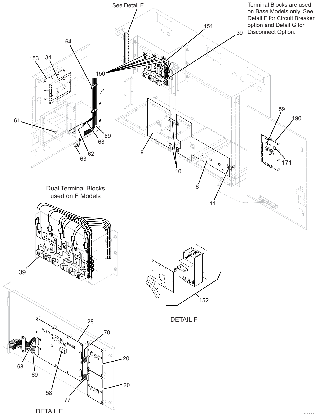
FIGURE 3 - CONTROL PANEL COMPONENTS
