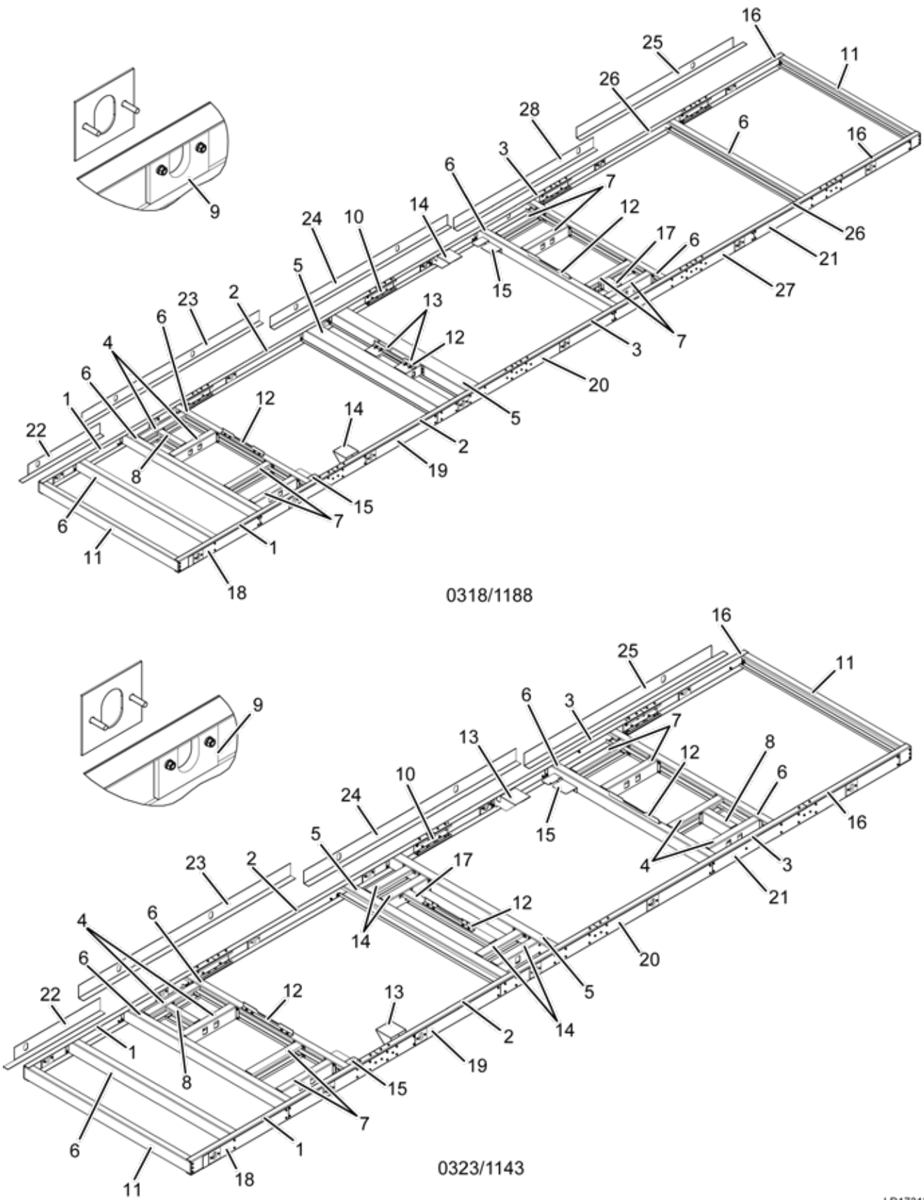
FIGURE 19 - BASE ASSEMBLY (0318/1188, 0323/1143)
