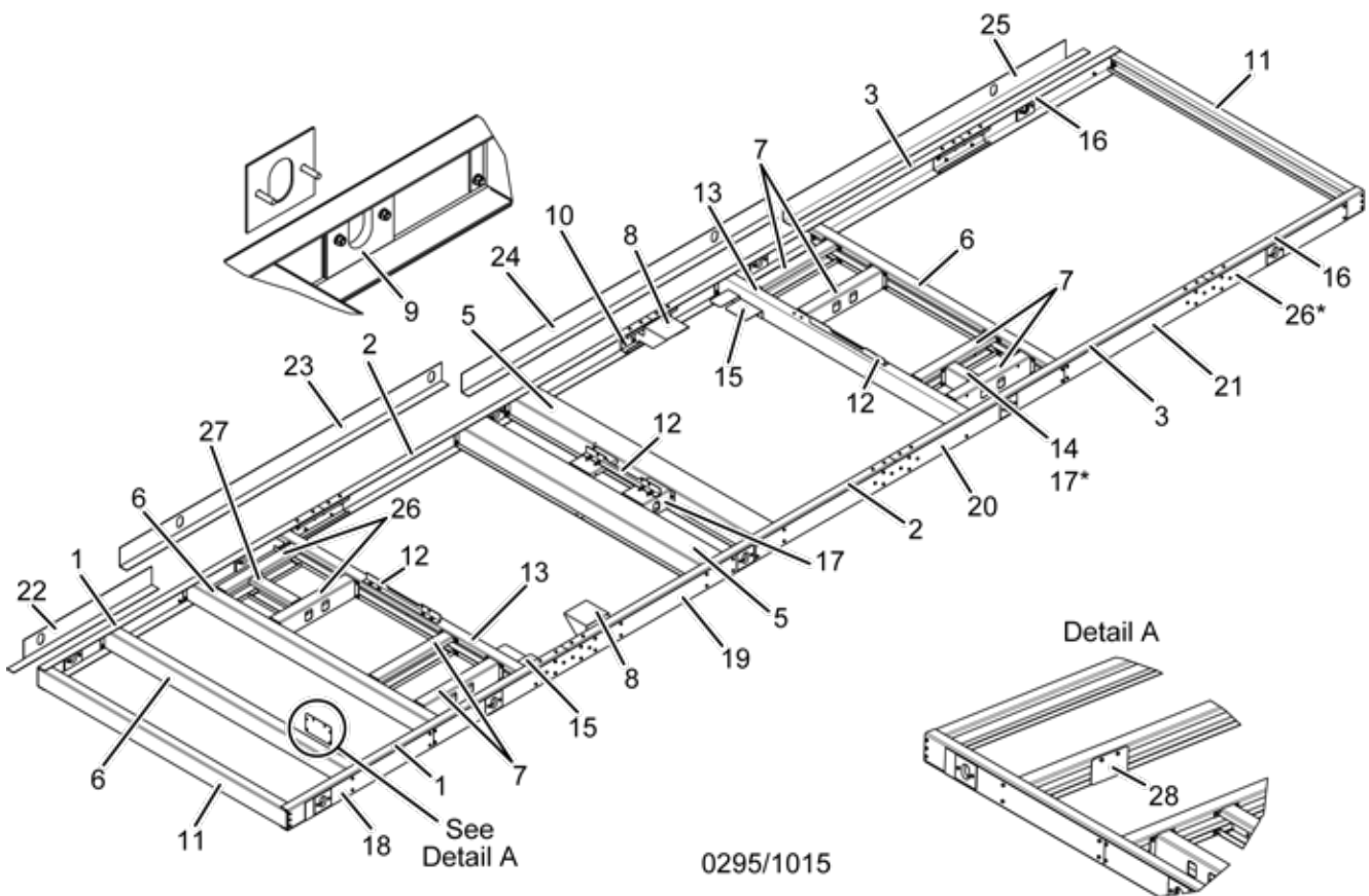
FIGURE 18 - BASE ASSEMBLY (0303/1093, 0305/1065, 0295/1015)
