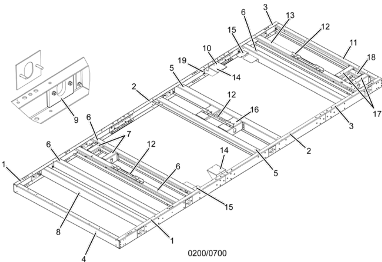
FIGURE 15 - BASE ASSEMBLY (0198/0688, 0200/0700)
