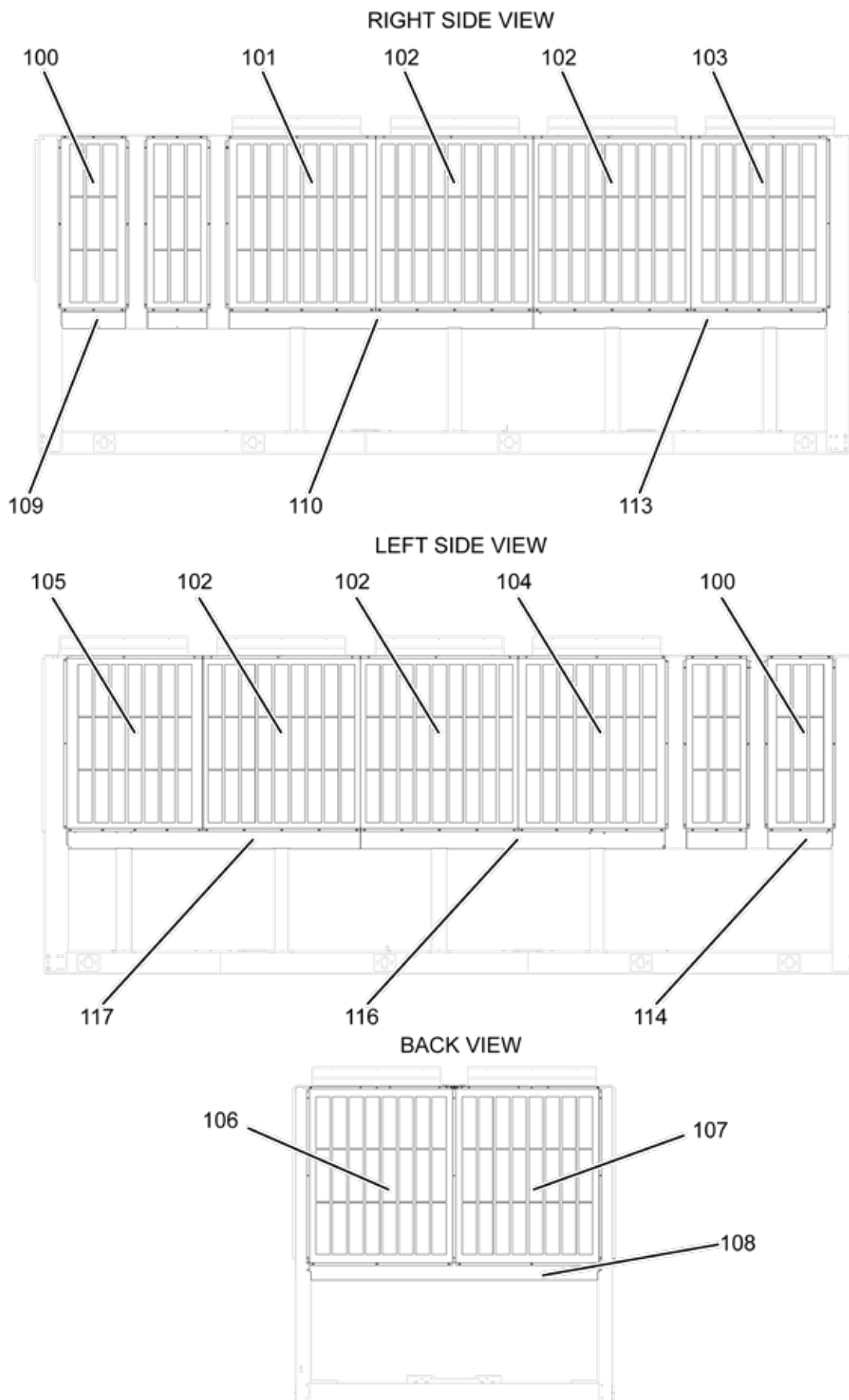
FIGURE 84 - LOUVERED ENCLOSURE (COND. ONLY) MODEL 0200/0700
