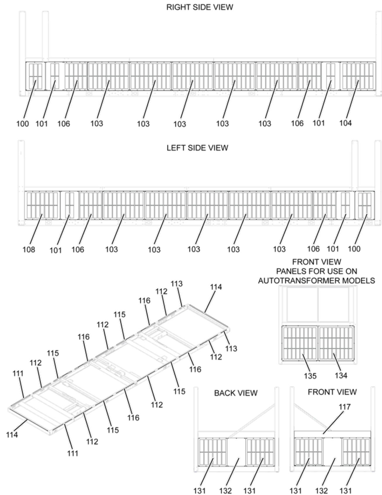
FIGURE 75 - BOTTOM SECTION: LOUVERED ENCLOSURE KIT COMPONENTS - MODEL 0165/0565 - 0198/0688, 0213/0743 - 0295/1015, 0323/1143, 0343/1193
