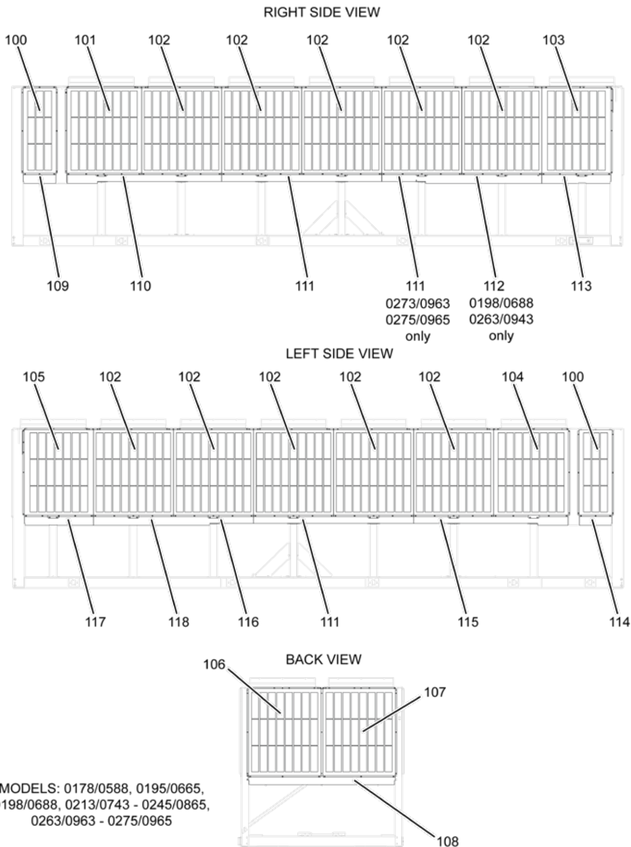
FIGURE 69 - TOP SECTION: LOUVERED ENCLOSURE KIT COMPONENTS - MODELS 0178/0588, 0195/0665, 0198/0688, 0213/0743 - 0245/0865, 0263/0963, 0275/0965
