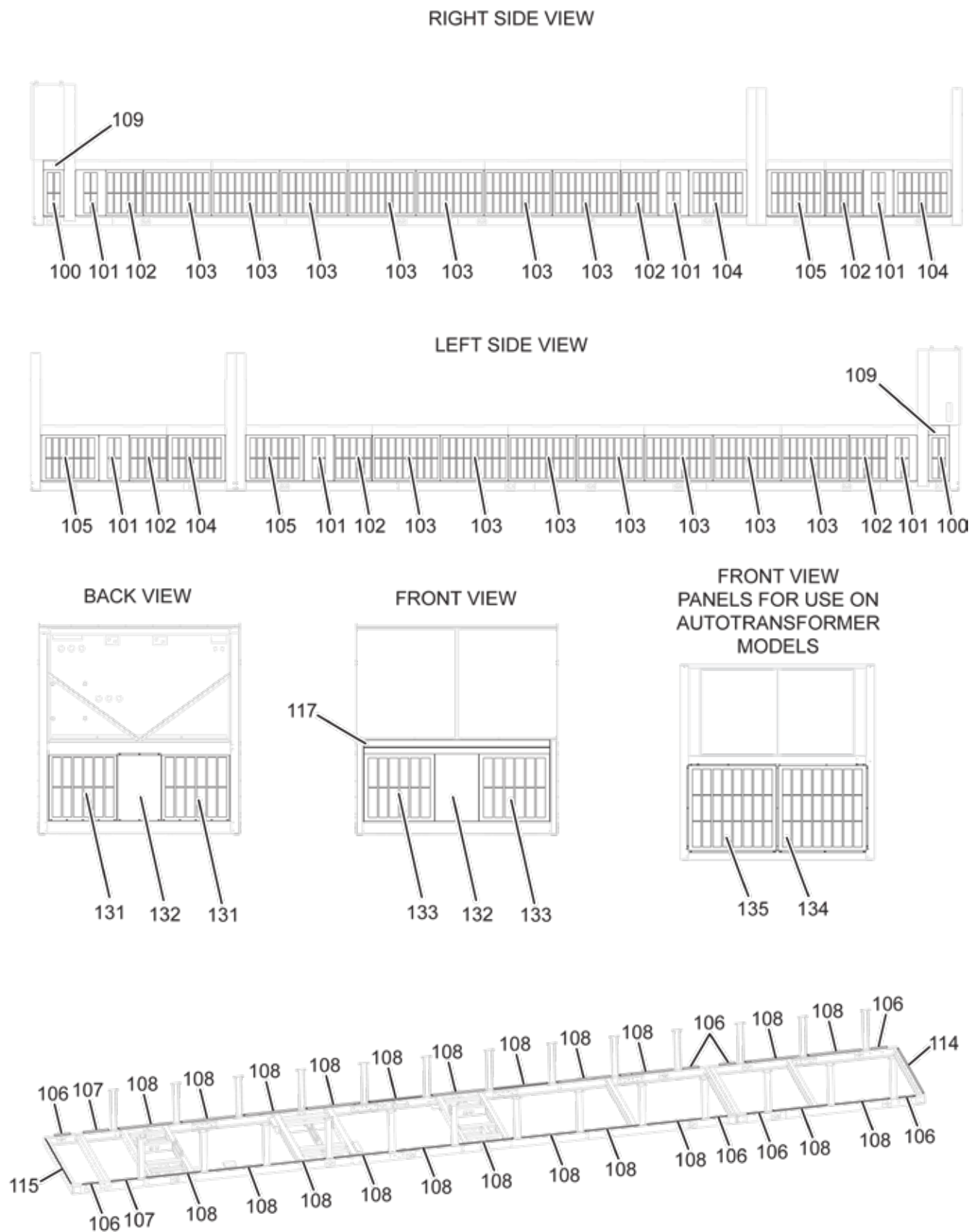
FIGURE 82 - BOTTOM SECTION: LOUVERED ENCLOSURE KIT COMPONENTS - MODEL 0428/1488, 0475/1665, 0483/1693, 0523/1843
