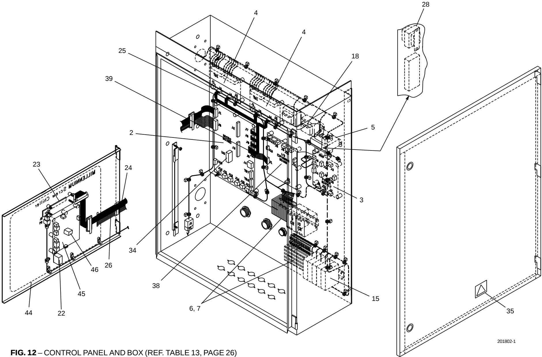
FIG. 12 – CONTROL PANEL AND BOX (REF. TABLE 13, PAGE 26)
