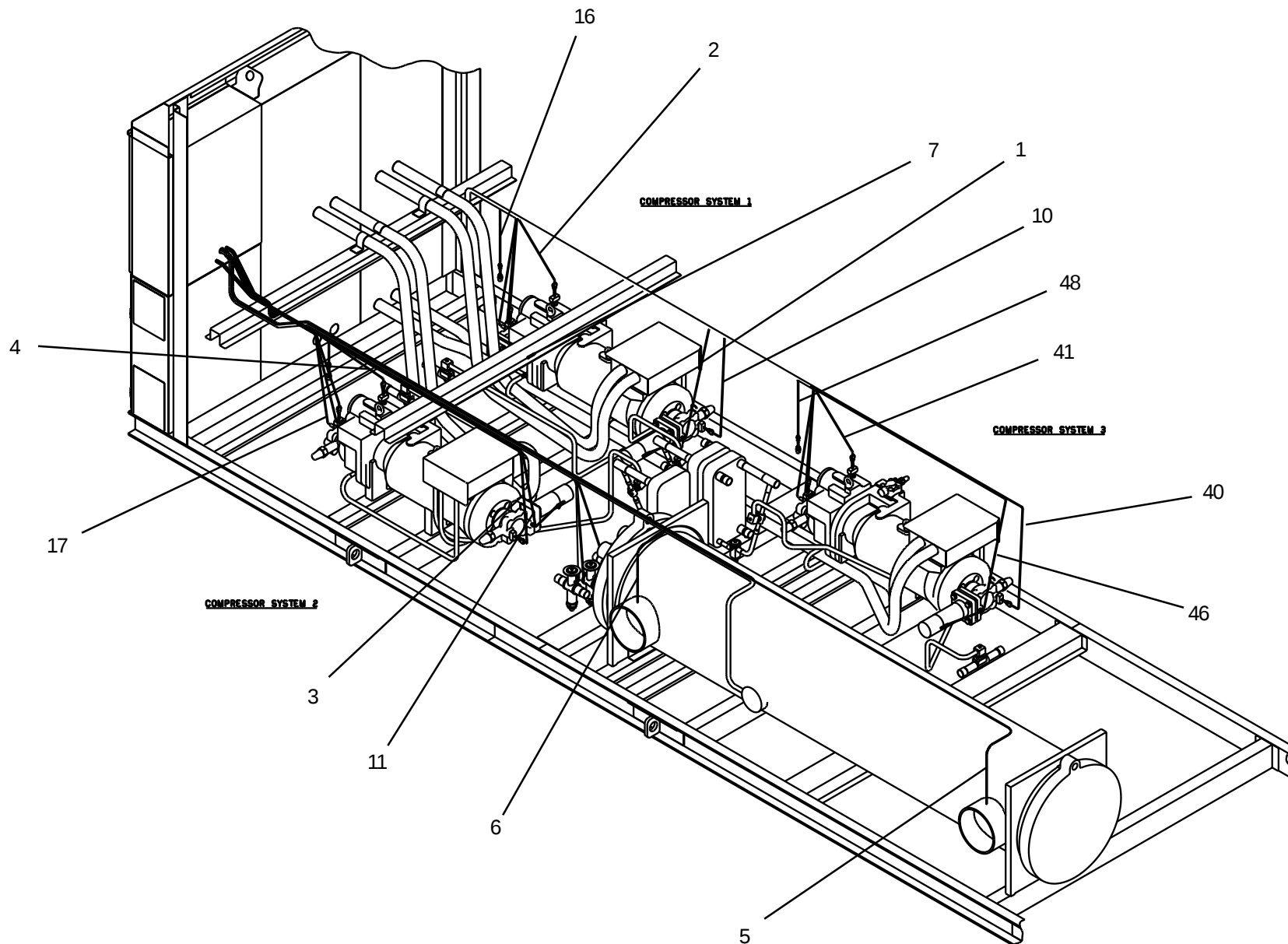
FIG. 15 – HARNESS LAYOUT (REF. TABLE 14, PAGES 29 AND 30)
