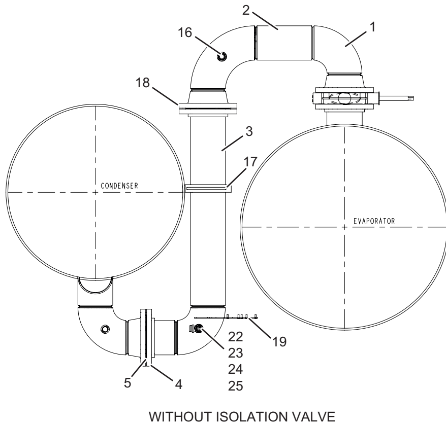
FIGURE 15 - LIQUID LINE (MOTOR - MA068AA AND MA095AA)
