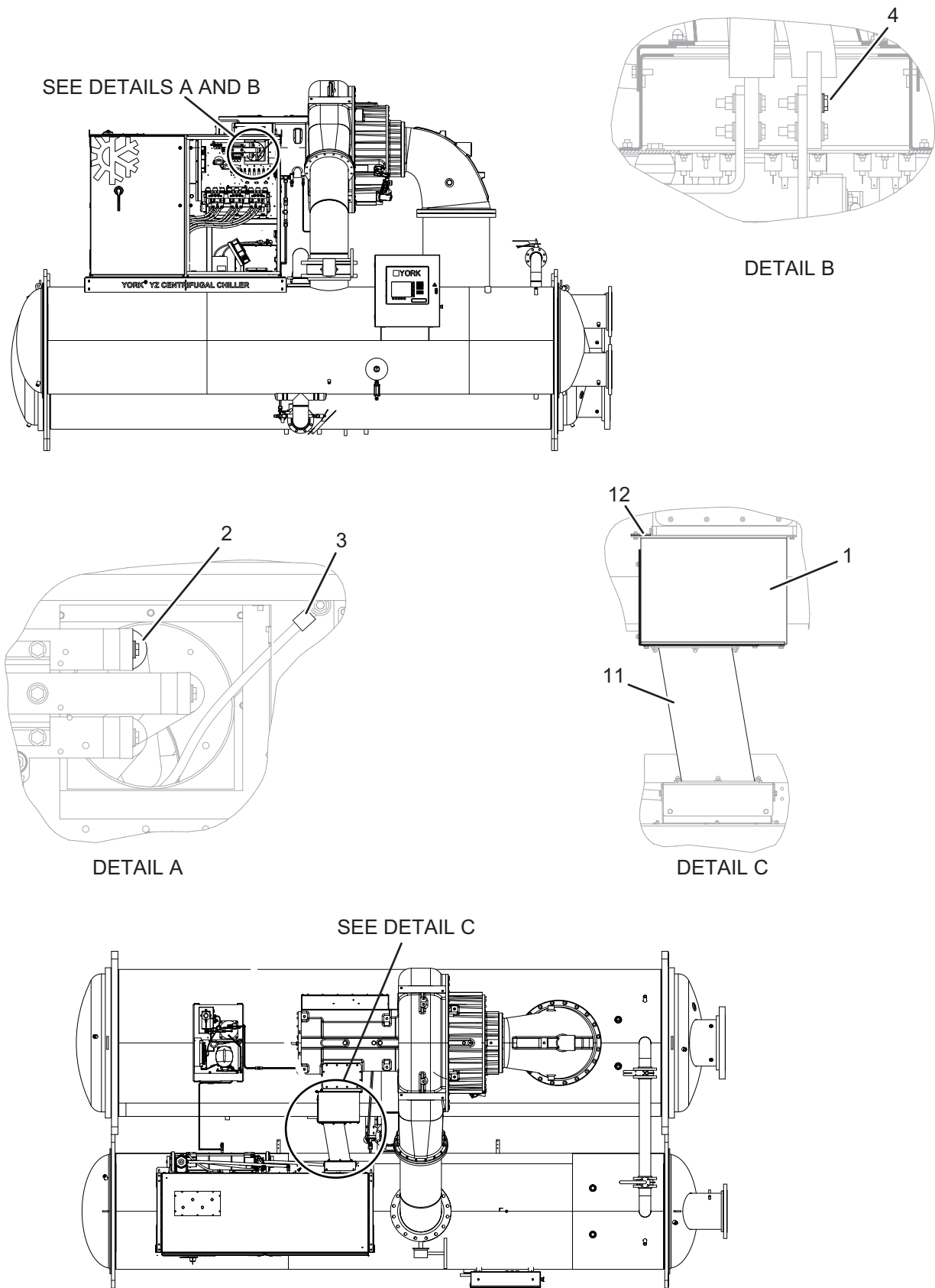
FIGURE 8 - MOTOR WIRING KIT - VSD PYT1280A
