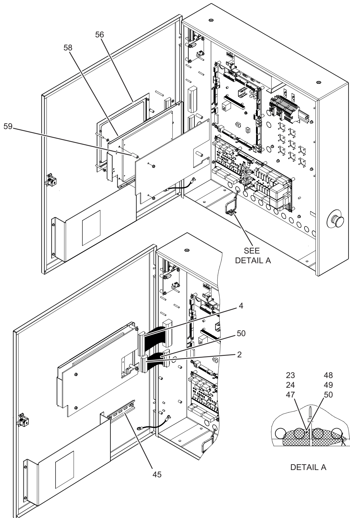
FIGURE 22 - OPTIVIEW PANEL
