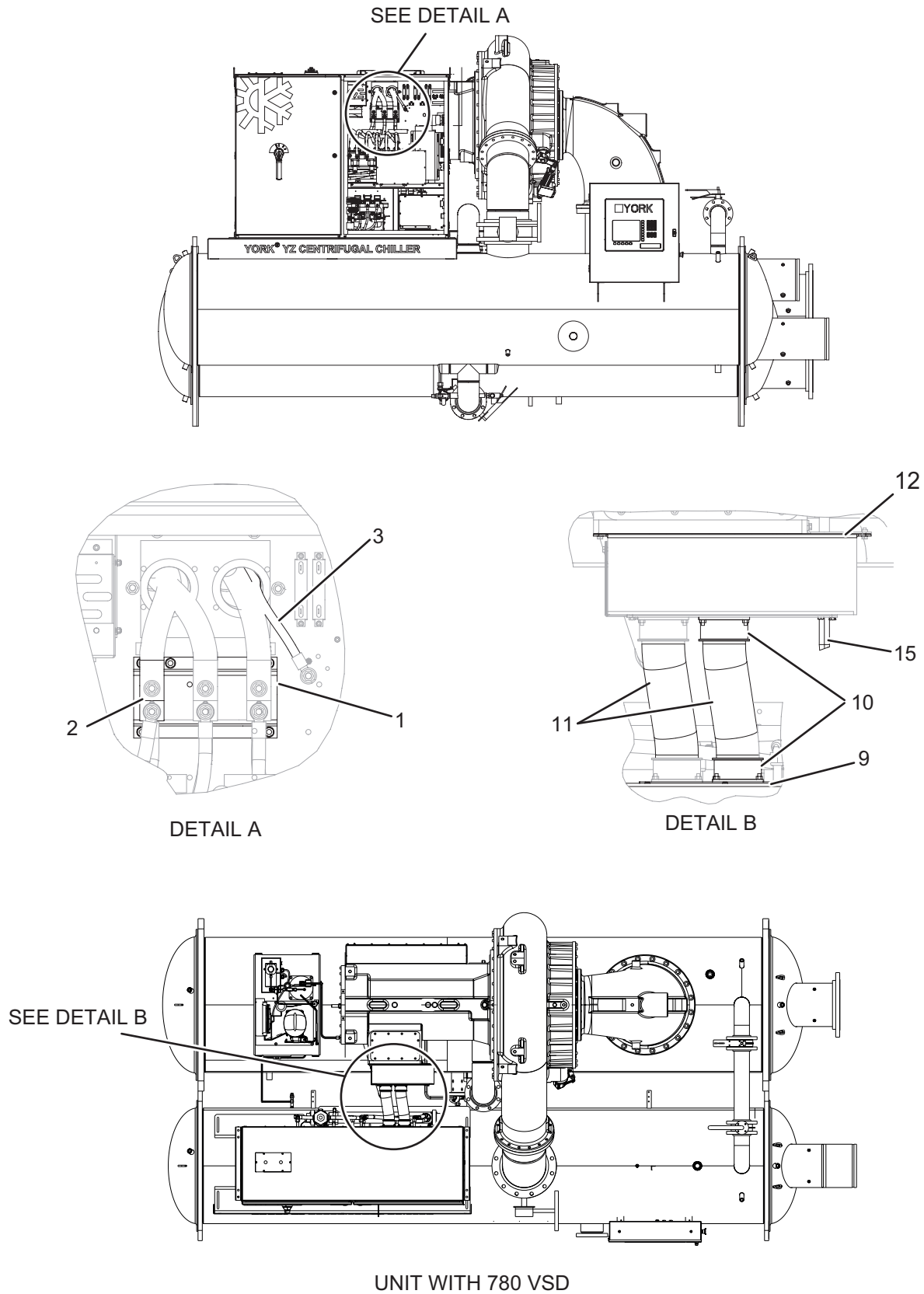
FIGURE 6 - MOTOR WIRING KIT - VSD PYT780A
