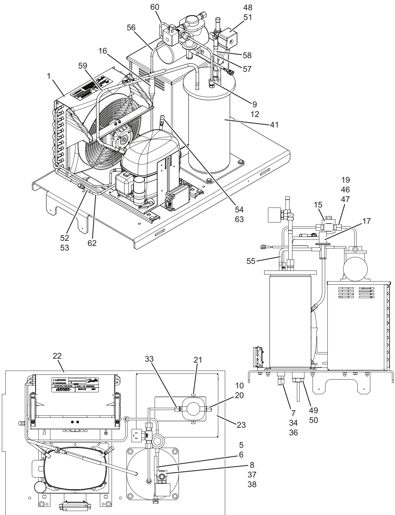
FIGURE 11 - PURGE UNIT
