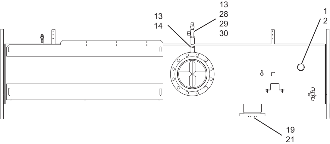
FIGURE 3 - CONDENSER CLOSURES
