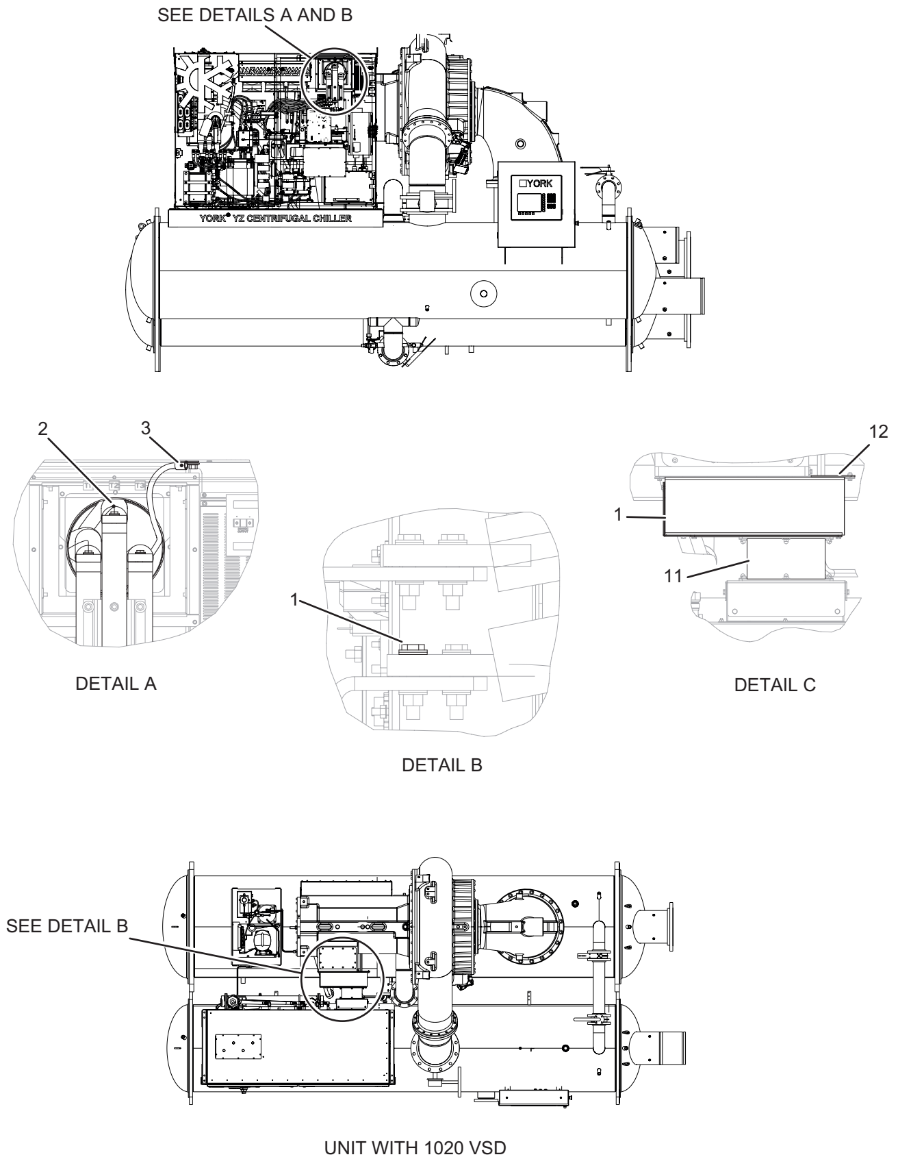
FIGURE 7 - MOTOR WIRING KIT - VSD PYT1020A
