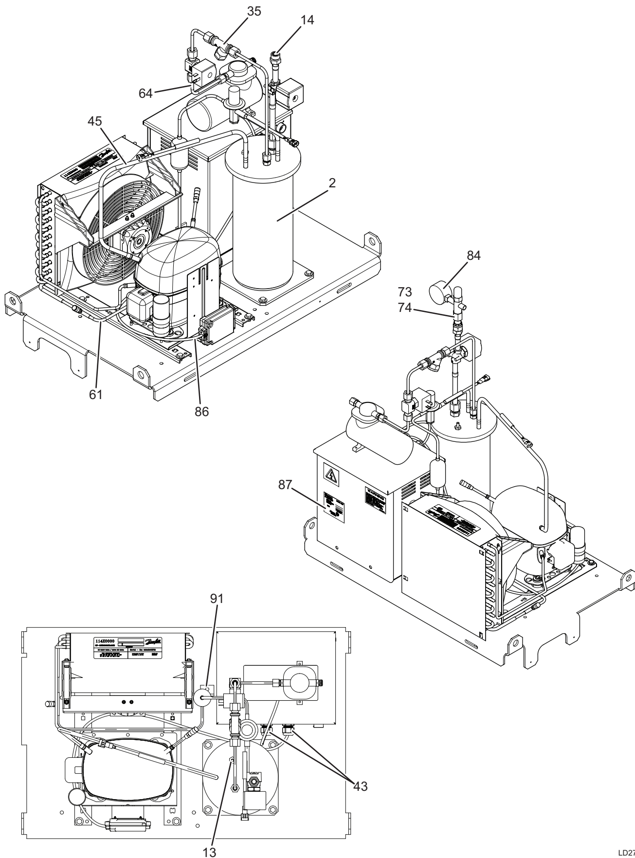
FIGURE 12 - PURGE UNIT
