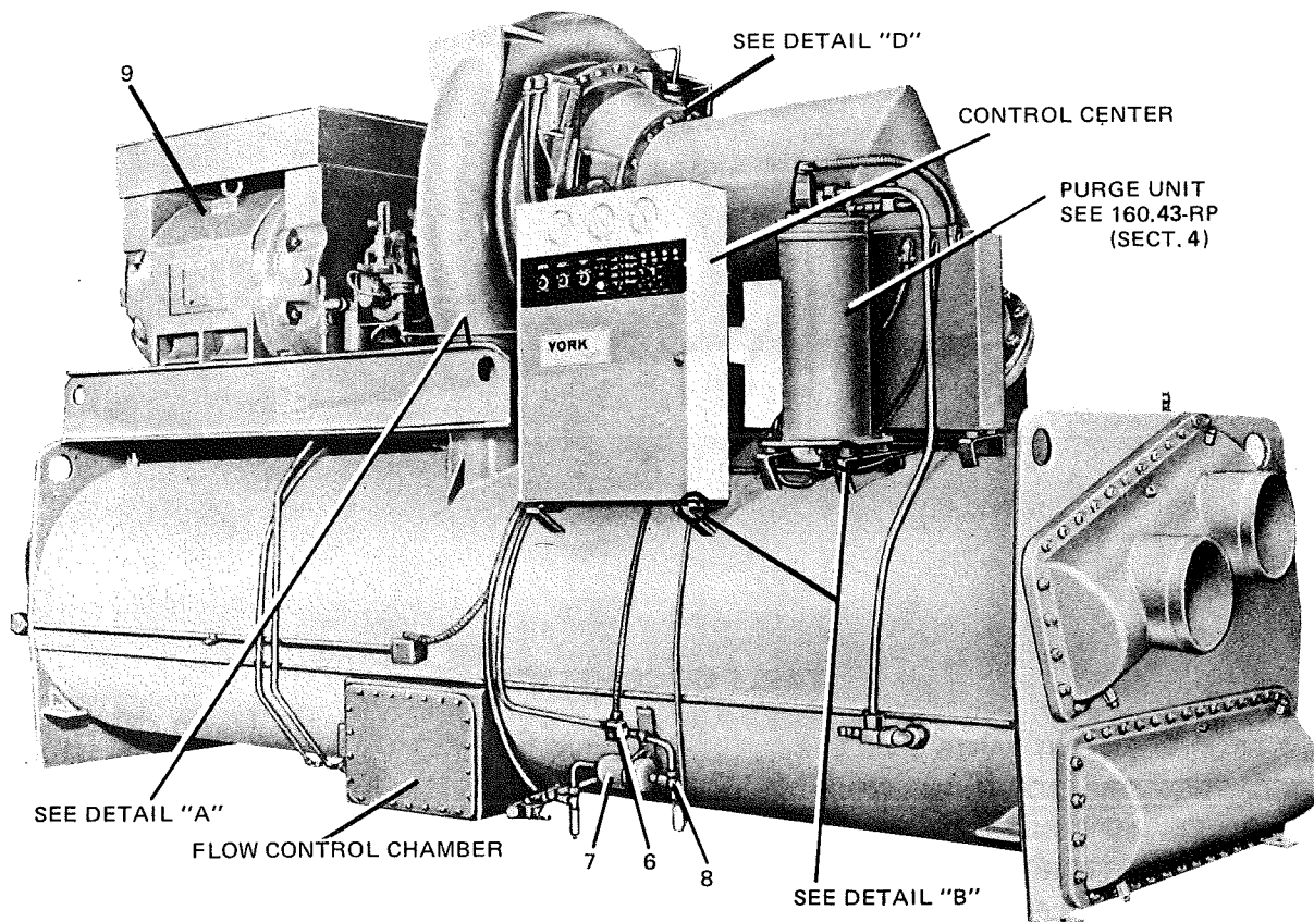
FIG. 1 — OPEN TURBOPAK — FRONT VIEW
