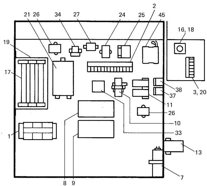
FIG. 2—MAIN CONTROL PANEL, LCHA35-25A AND -61A
