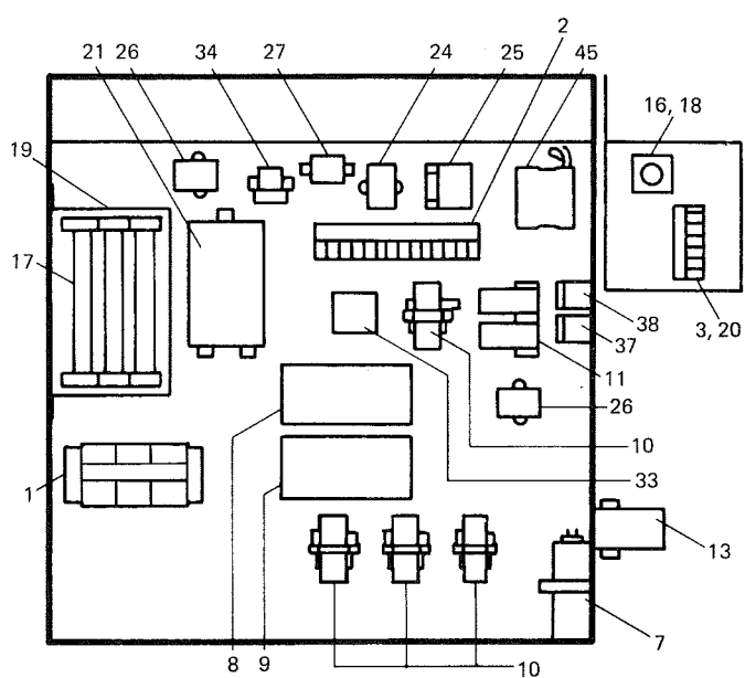
FIG. 3—MAIN CONTROL PANEL, LCHA35-46A, -58A AND -67A
