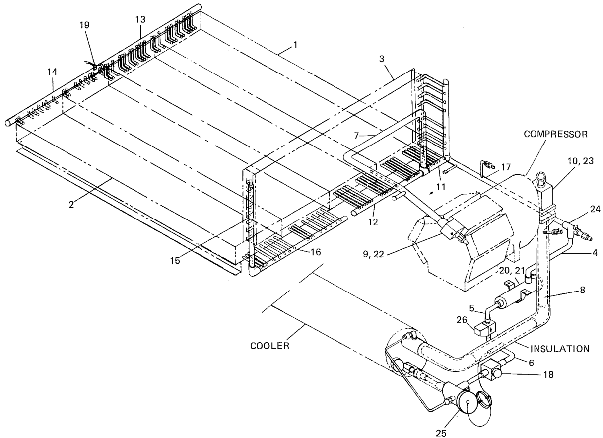
FIG. 5—REFRIGERANT PIPING
