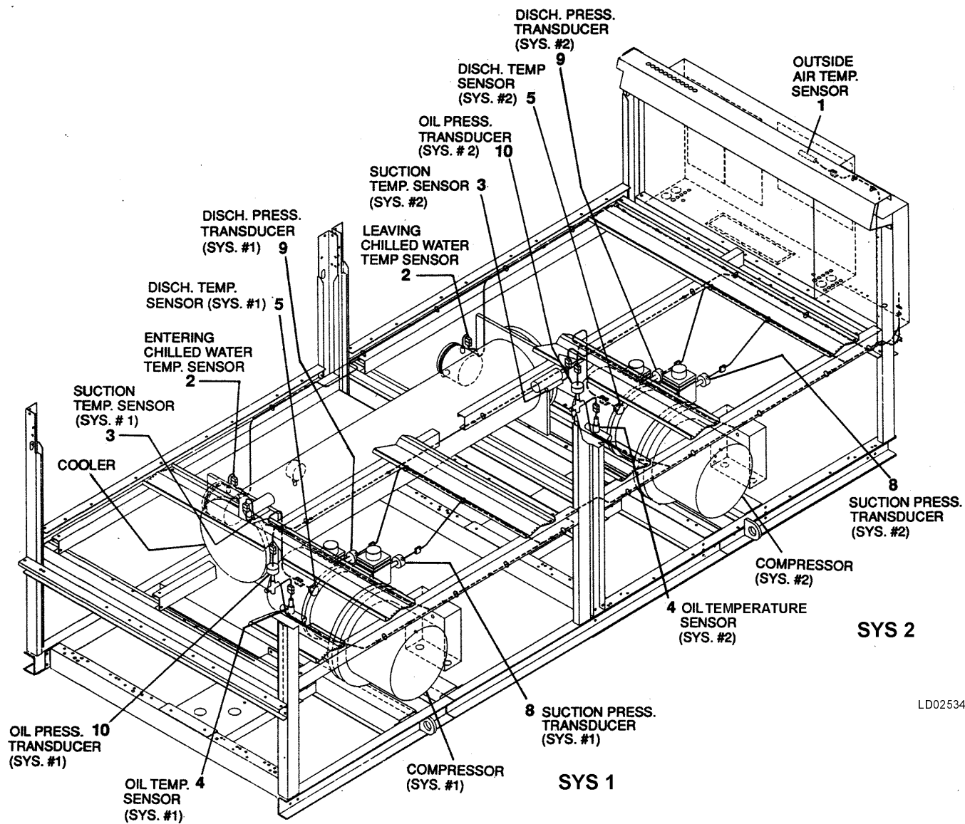
FIG. 2 – SYSTEM CONTROLS (Standard Unit Shown) Control Locations also Typical for Reverse Unit Components Except: System 1 = System 3; System 2 = System 4; No Item 1, OAT Sensor
