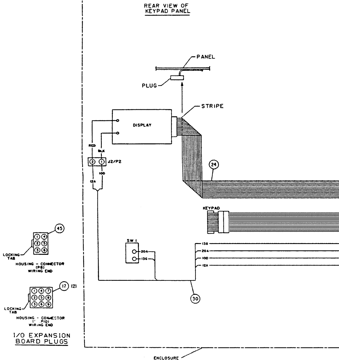
FIG. 5 – STANDARD UNIT CONTROL PANEL, CONNECTION DIAGRAM
