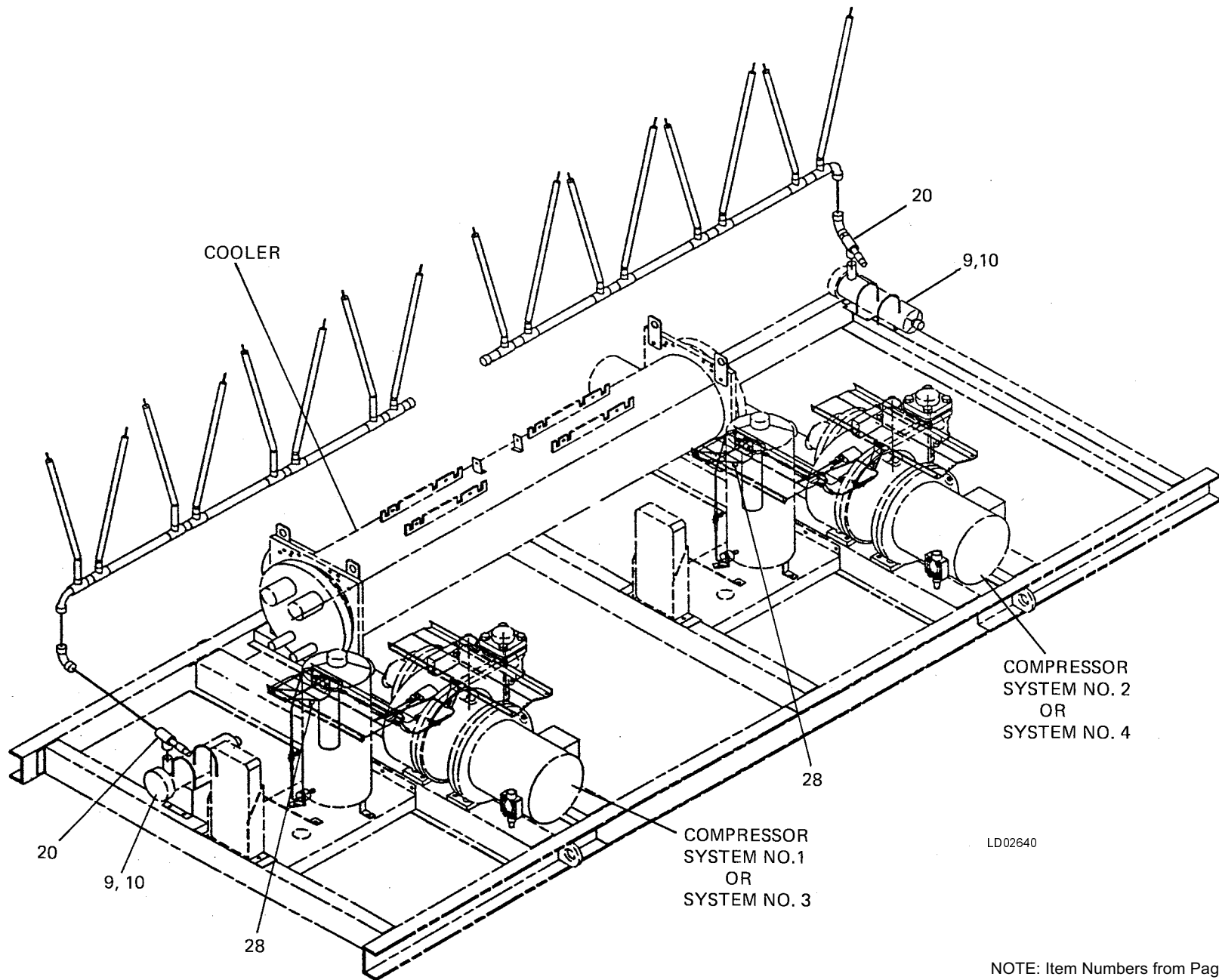
FIG. 10 – SYSTEM PIPING (Liquid Piping to Dehydrator)
