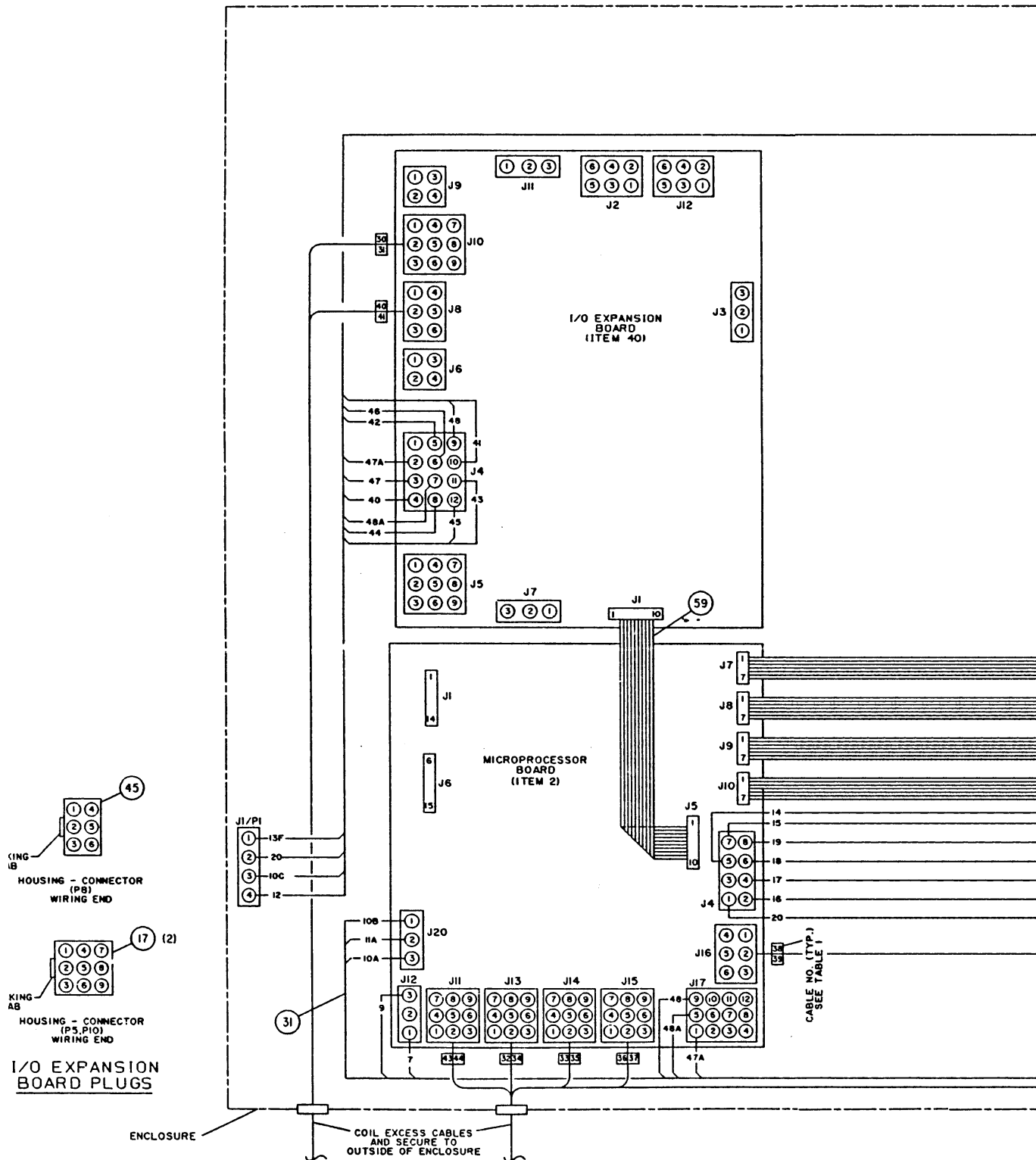
FIG. 7 – REVERSE UNIT CONTROL PANEL, CONNECTION DIAGRAM
