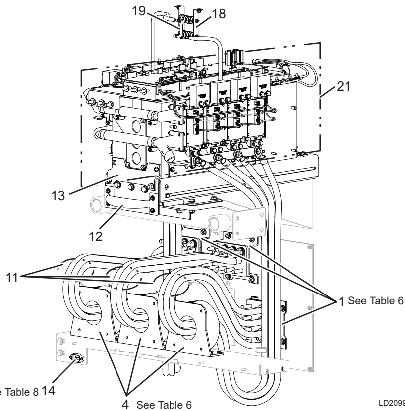
FIGURE 13 - POWER ASSEMBLY COMPONENTS
