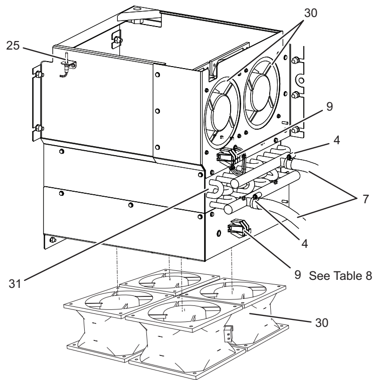
FIGURE 7 - COOLING SYSTEM COMPONENTS
