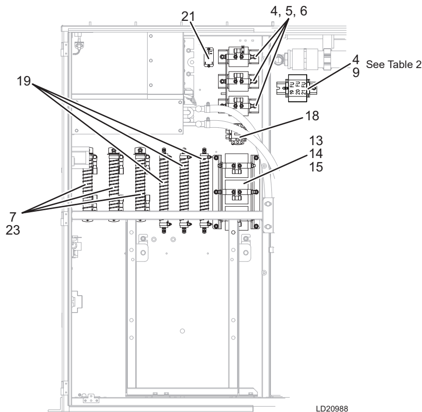
FIGURE 2 - INPUT COMPONENTS
