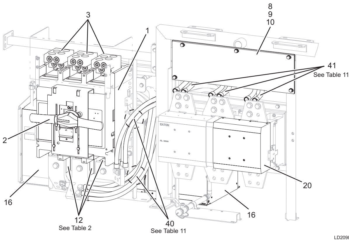
FIGURE 1 - INPUT COMPONENTS
