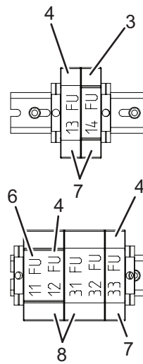
Detail B
