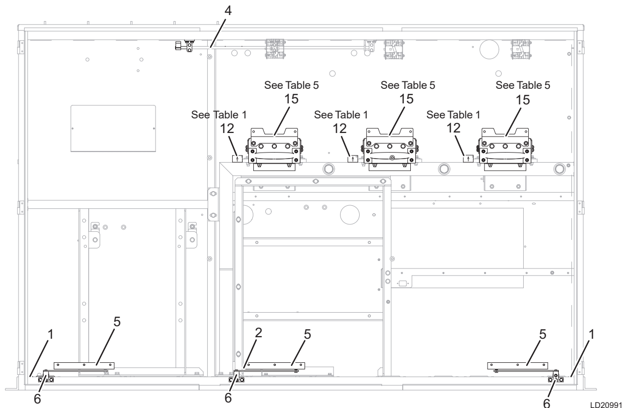
FIGURE 6 - DOOR COMPONENTS
