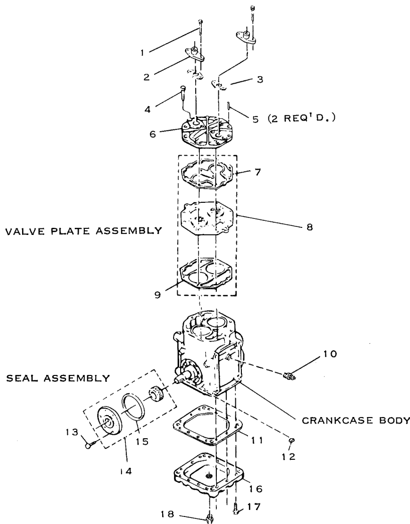
FIG. 2— REFRIGERANT TRANSFER UNIT COMPRESSOR PARTS
