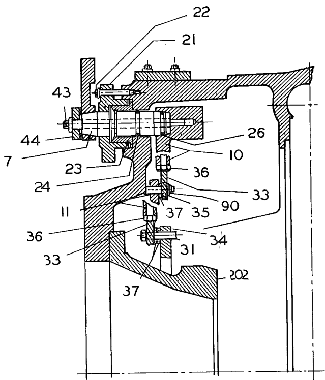
FIG. 5— Internal PRV Control Shaft
