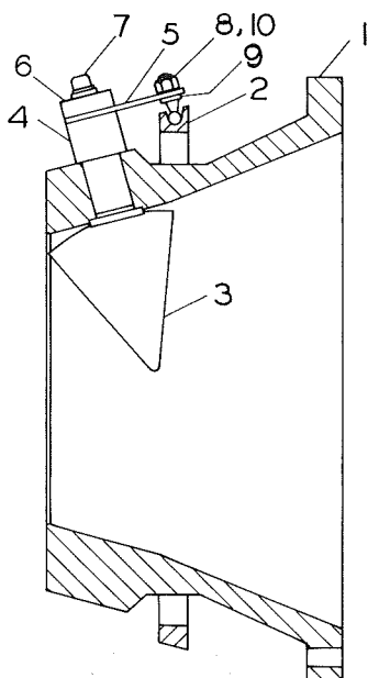
FIG. 9- Cross Section View of Pre-Rotation Device
