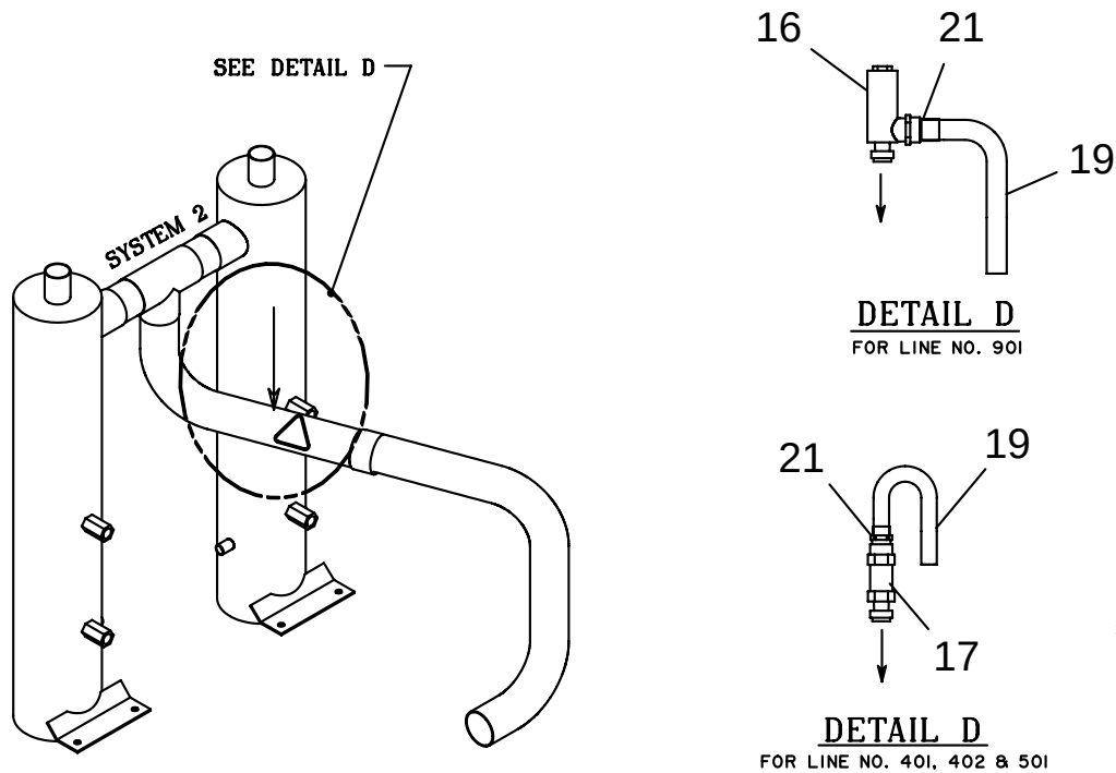
FIG. 6 – RELIEF VALVES AND CUTOUT SWITCHES (REF. TABLE 6, PAGE 27)
