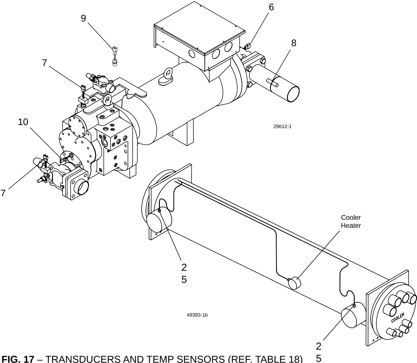
FIG. 17 – TRANSDUCERS AND TEMP SENSORS (REF. TABLE 18)
