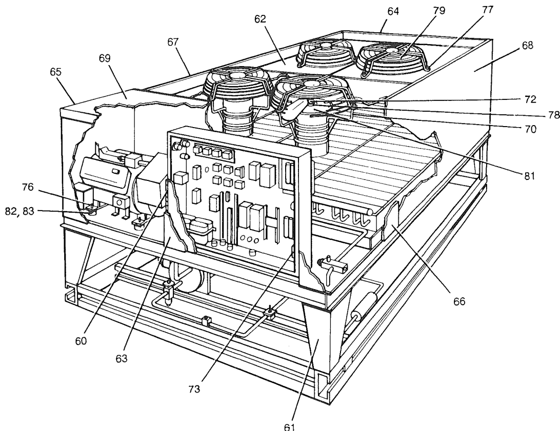
FIG. 4 - AIR COOLED WATER CHILLER
