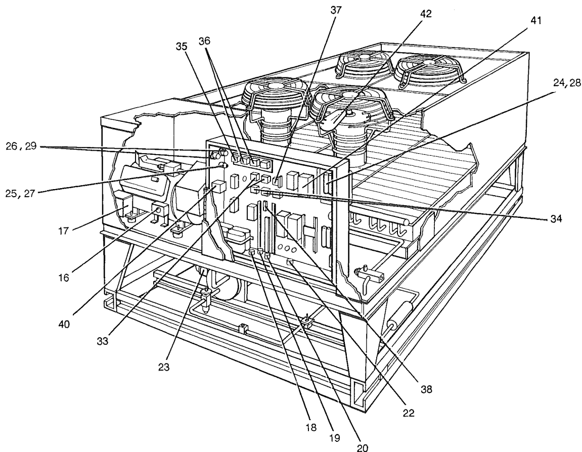
FIG. 2 - AIR COOLED WATER CHILLER
