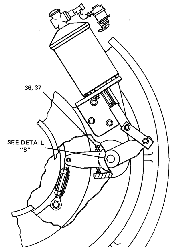
FIG. 5 – PNEUMATIC PRV POSITION LEVER – ADJUSTMENT PARTS
