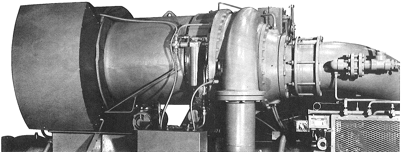
FIG. 1 – HERMETIC-MOTOR COMPRESSOR, MODEL MKC
