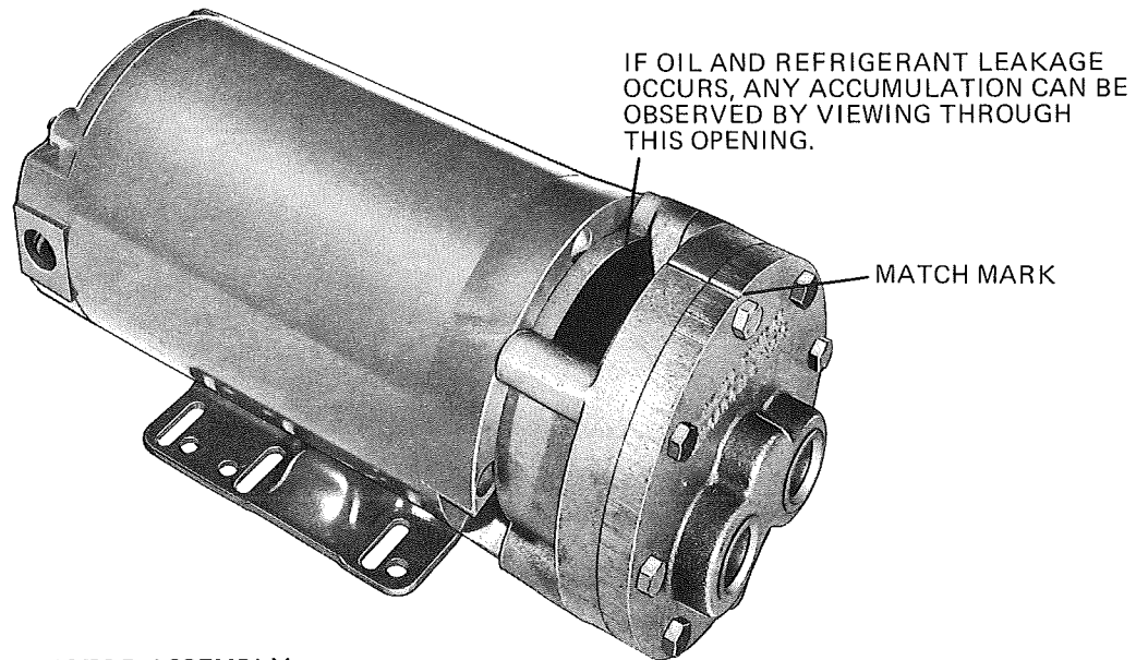
FIG. 13— OIL PUMP AND MOTOR ASSEMBLY
