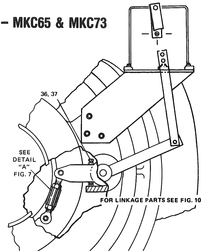
FIG. 4 – ELECTRIC MOTOR LEVER – ADJUSTMENT PARTS
