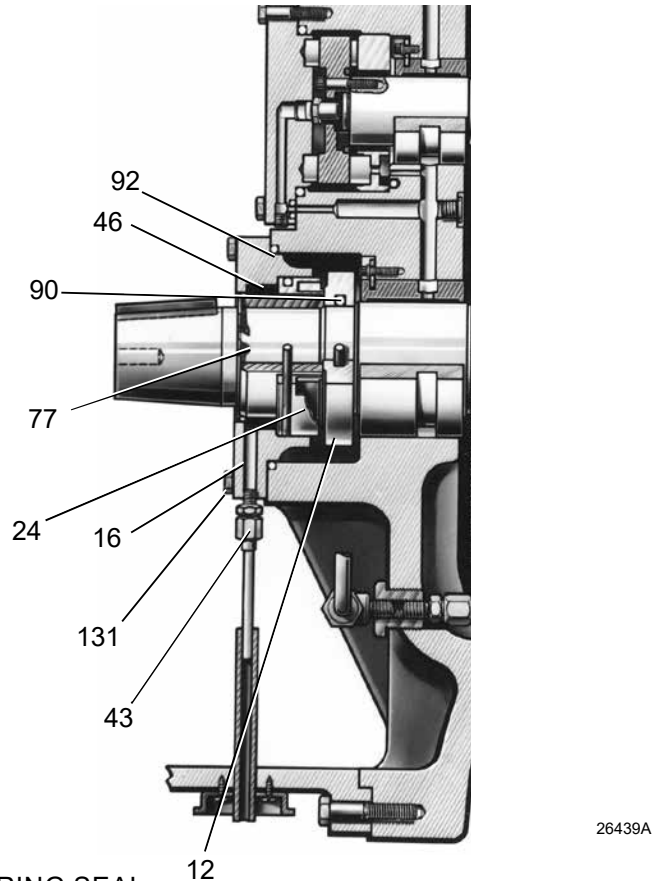
FIGURE 8 - DYNAMIC O-RING SEAL
