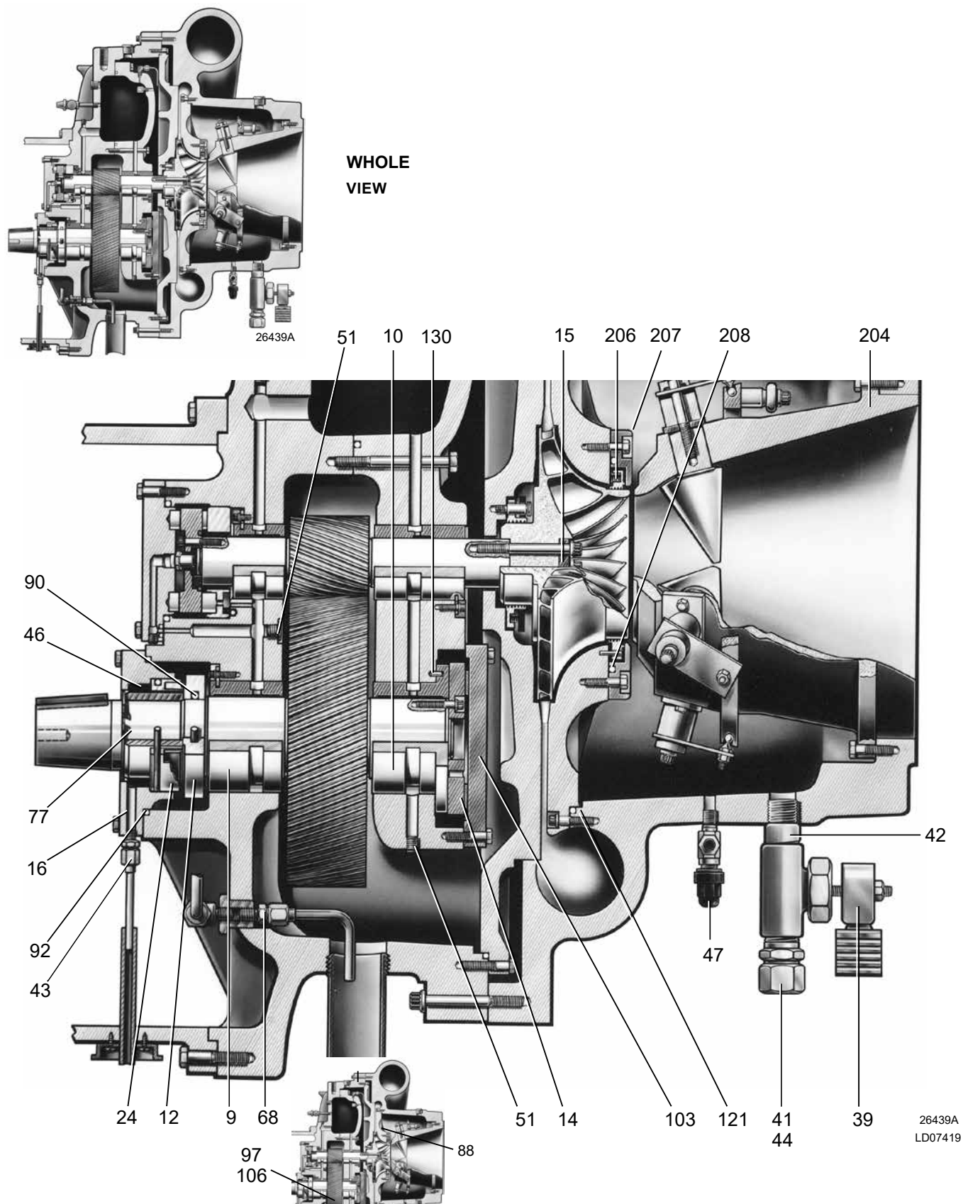
FIGURE 3 - HA46, HA50, HA57, HB57 AND HB61
