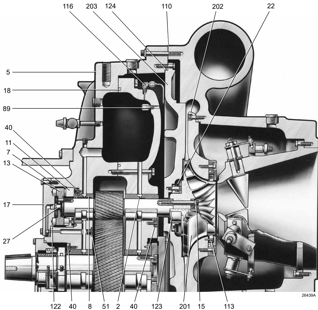
FIGURE 5 – HA65, HA70, HA73, HA81 AND HA90 (CONT'D)
