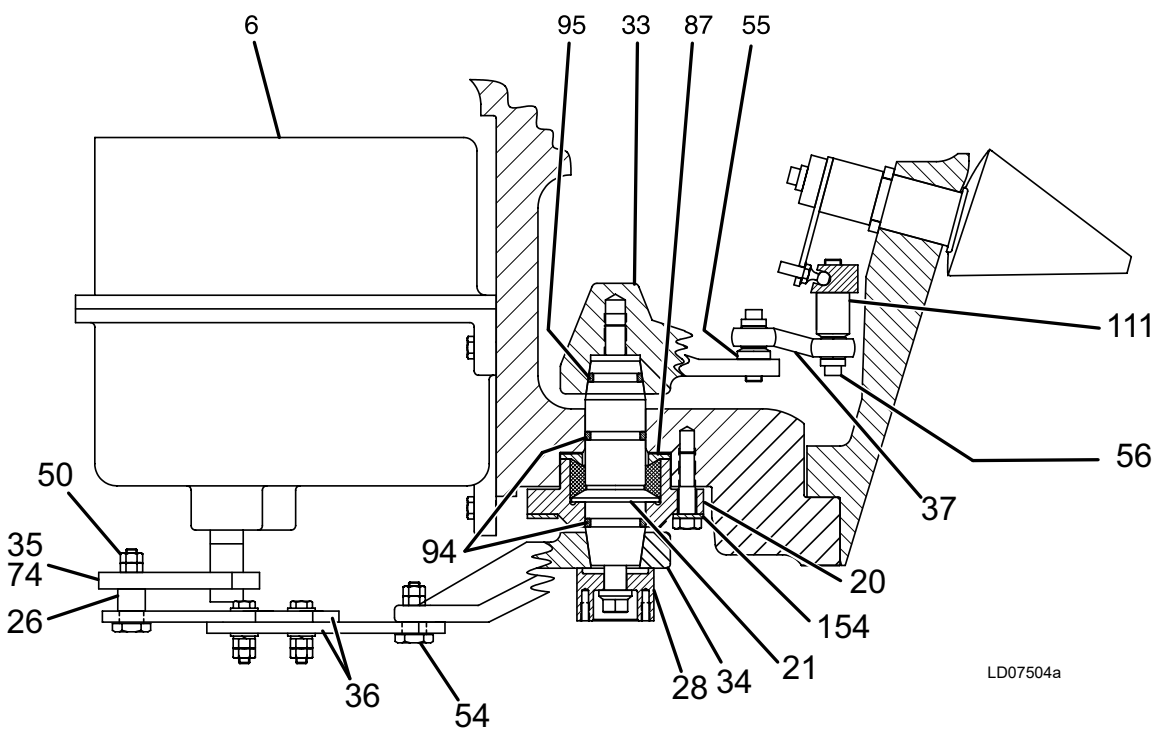
FIGURE 5 – HA65, HA70, HA73, HA81 AND HA90 (CONT'D)
