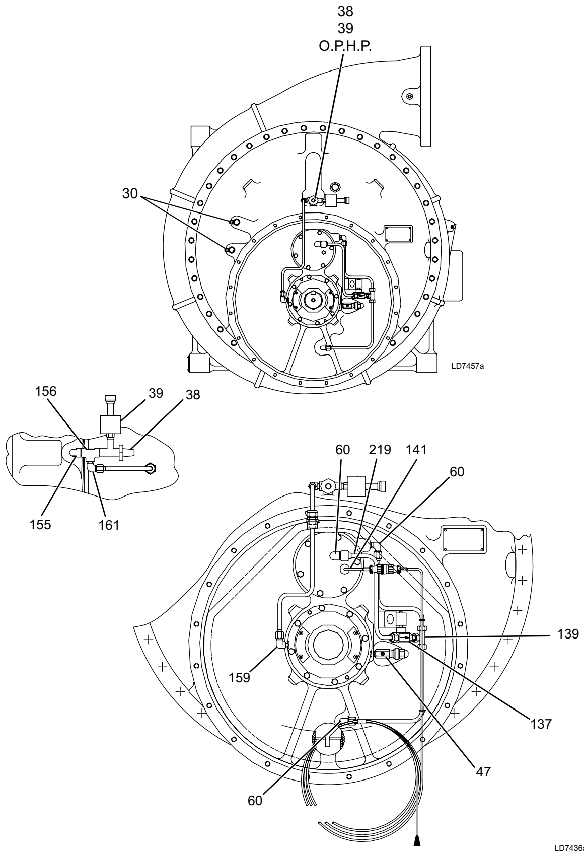
FIGURE 6 - HA65, HA73, HA81 AND HA90 (CONT'D)
