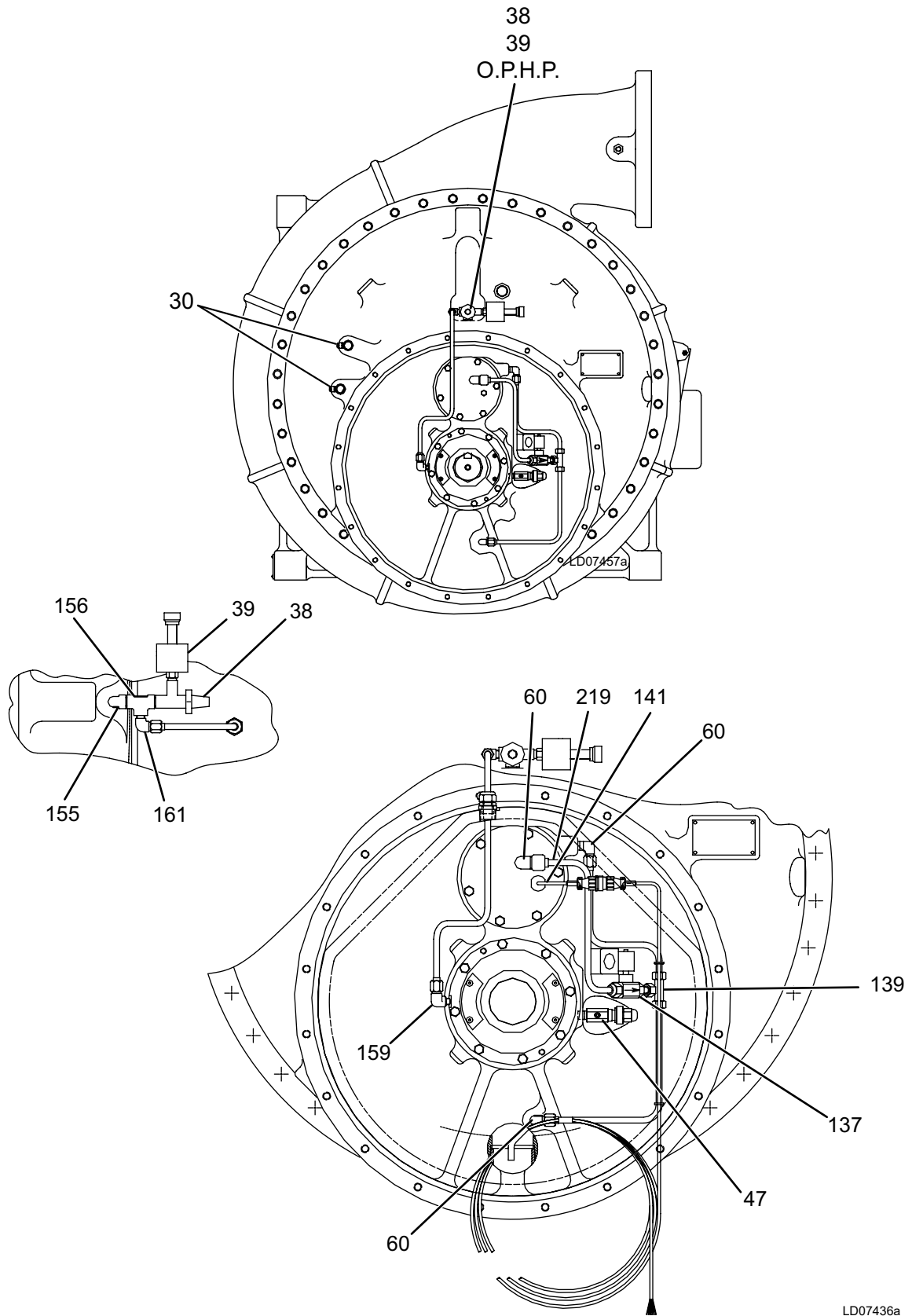
FIGURE 5 – HA65, HA70, HA73, HA81 AND HA90 (CONT'D)
