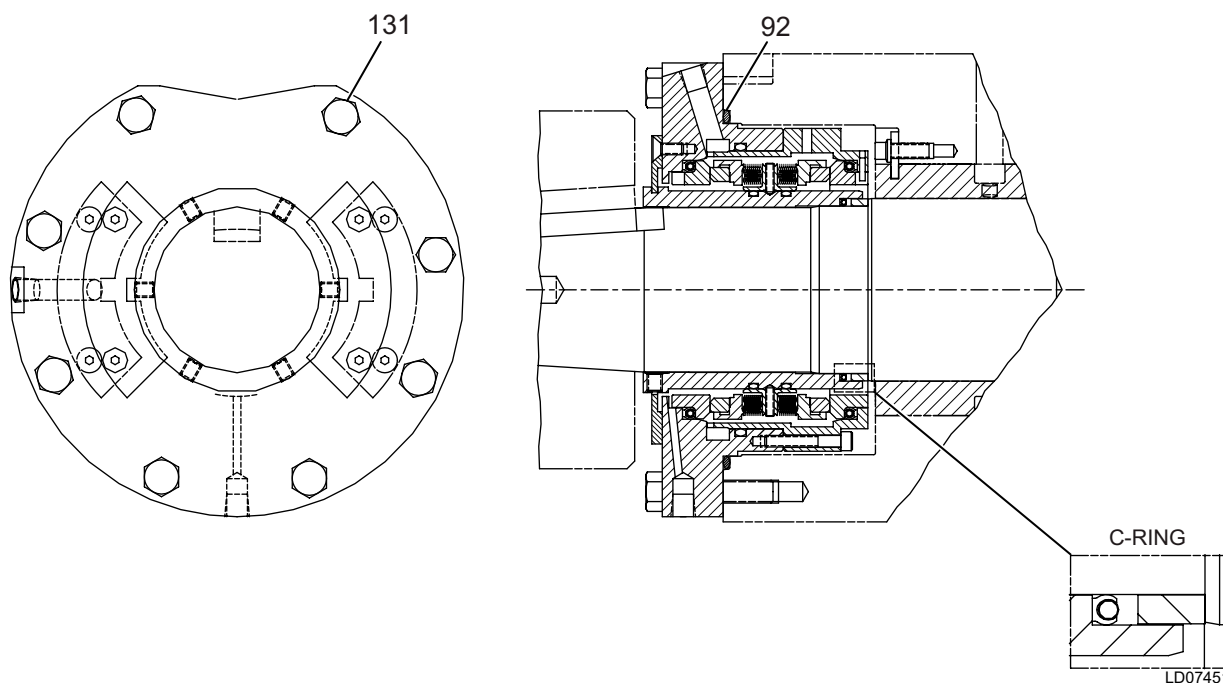
FIGURE 9 - BELLOWS SEALS
