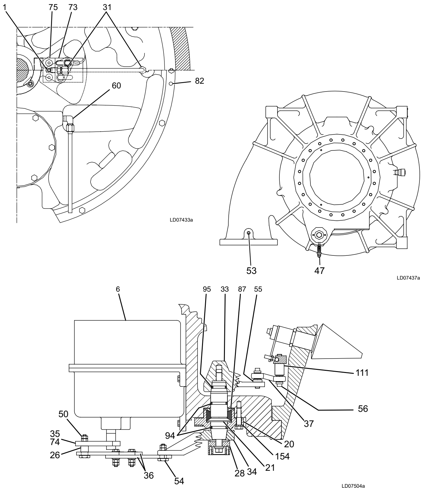
FIGURE 6 - HA65, HA73, HA81 AND HA90 (CONT'D)
