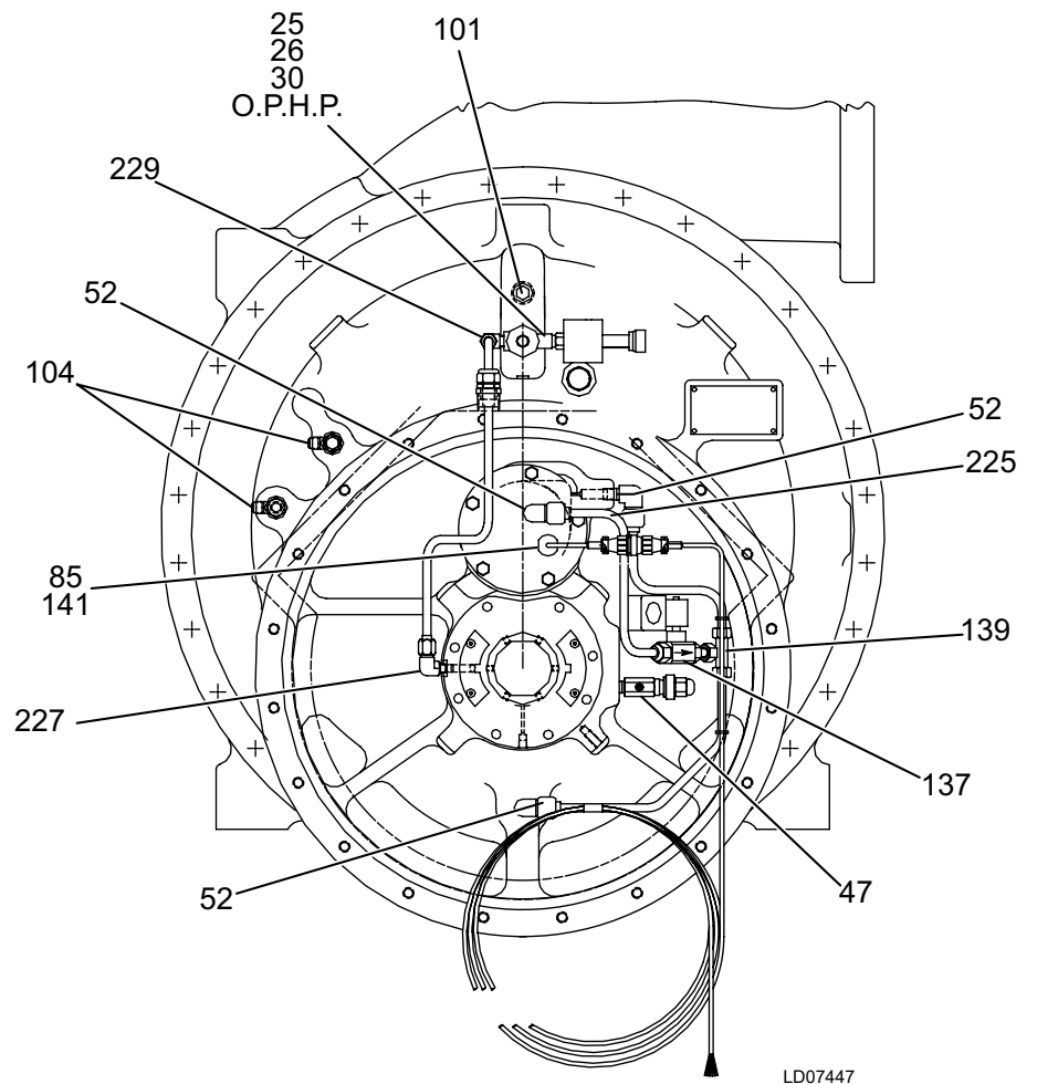
FIGURE 3 – HA46, HA50, HA57, HB57 AND HB61 (CONT'D)
