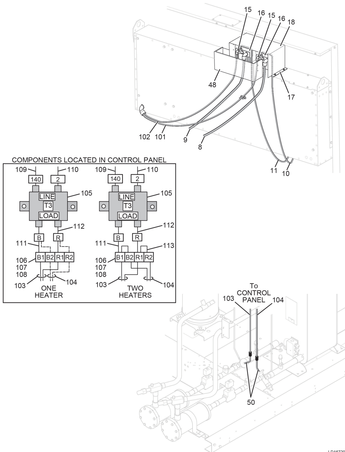
FIGURE 58 - LOW AMBIENT KIT
