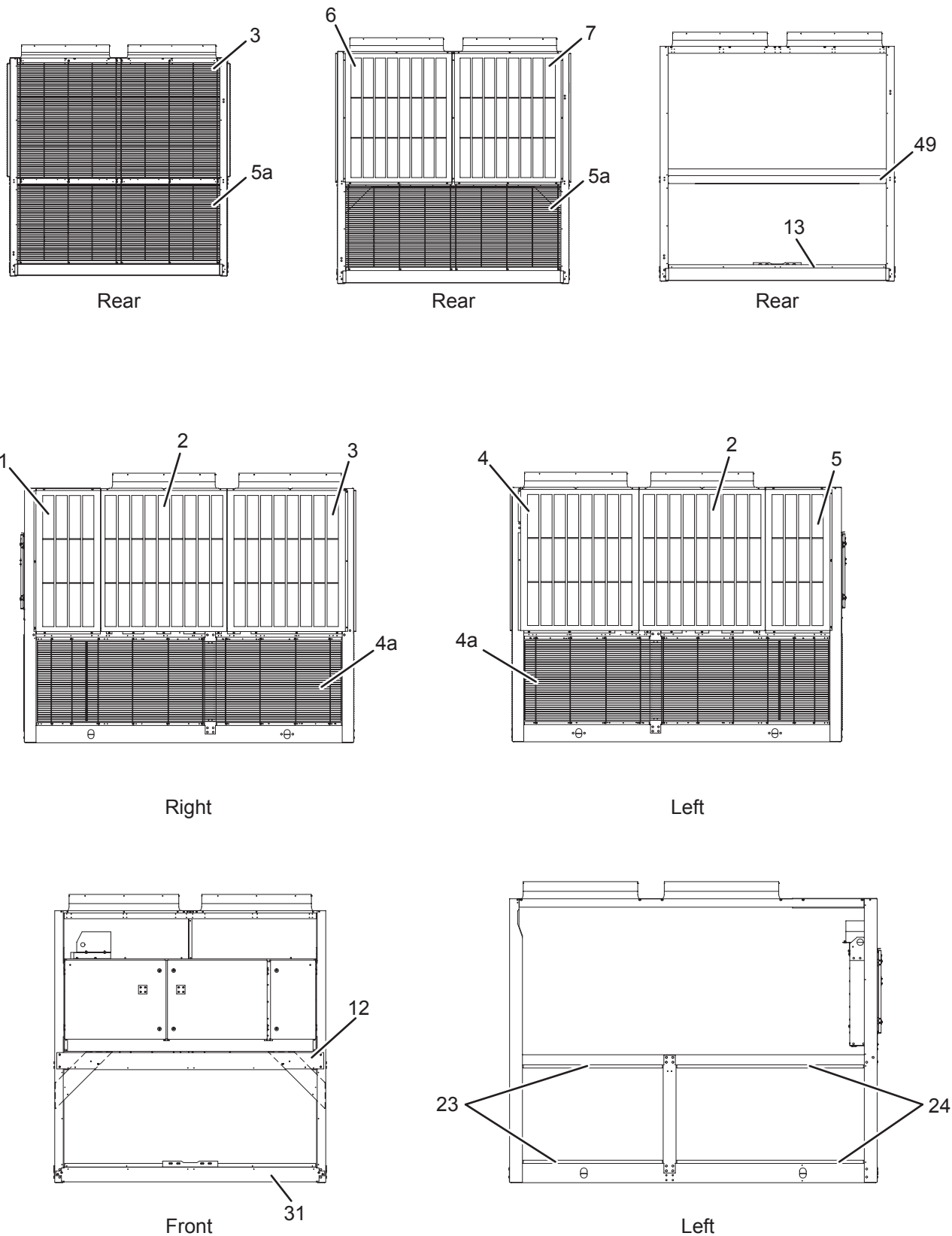
FIGURE 71 - WIRE LOUVER ENCLOSURE PANELS (YLAA0058 - YLAA0089)
