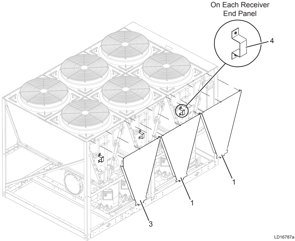
FIGURE 82 - AESTHETIC PANEL
