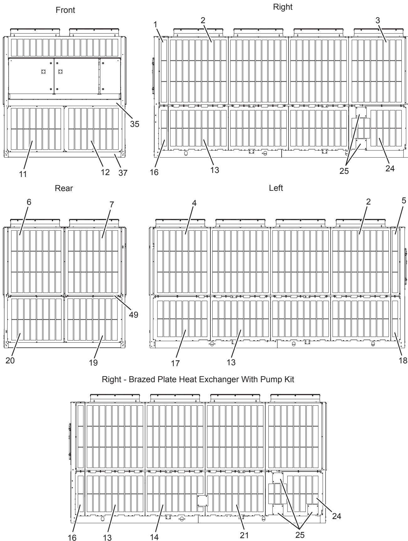
FIGURE 68 - LOUVERED ENCLOSURE PANELS (YLAA0125 - YLAA0155)
