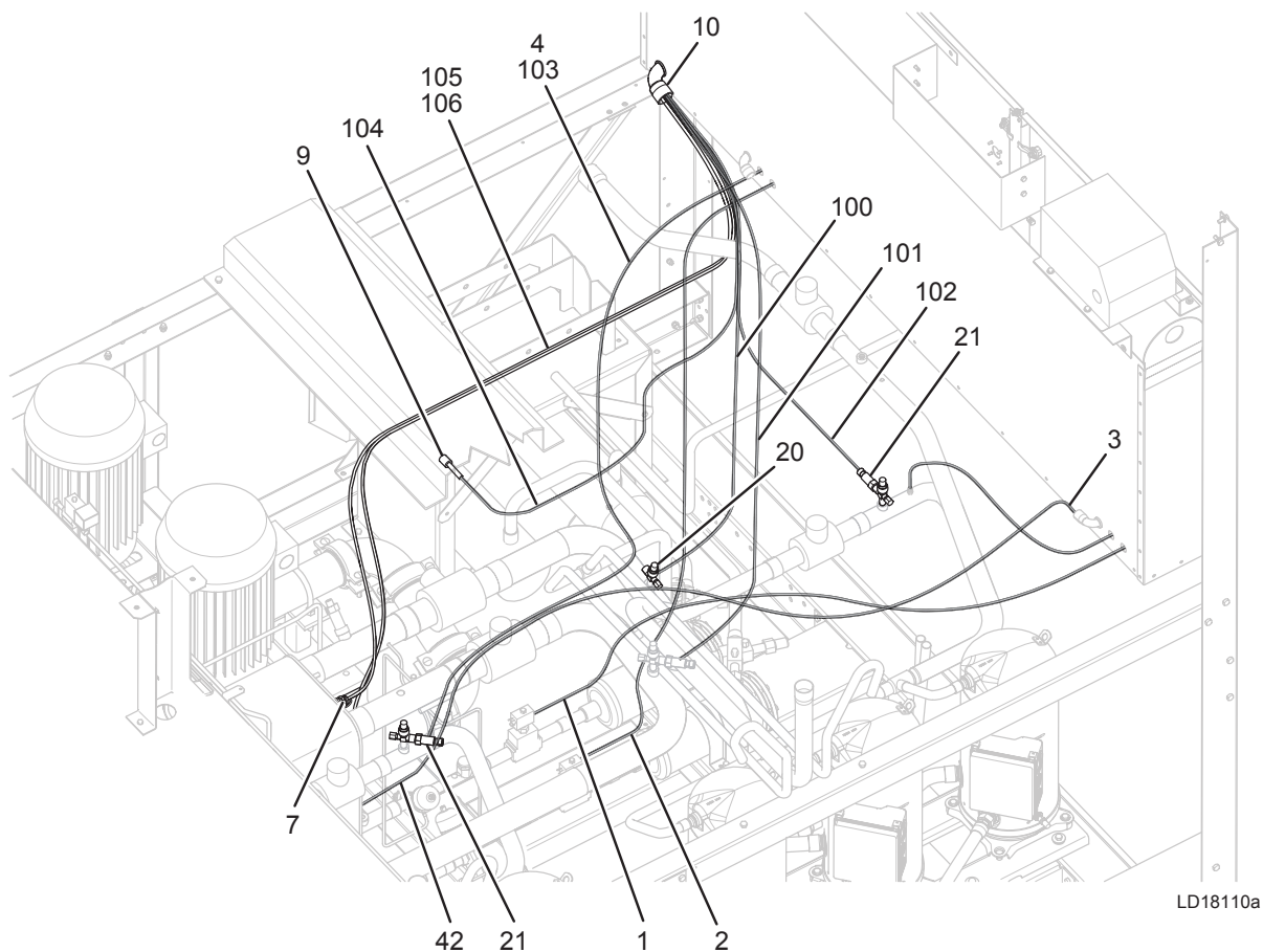
FIGURE 27 - SYSTEM WIRING
