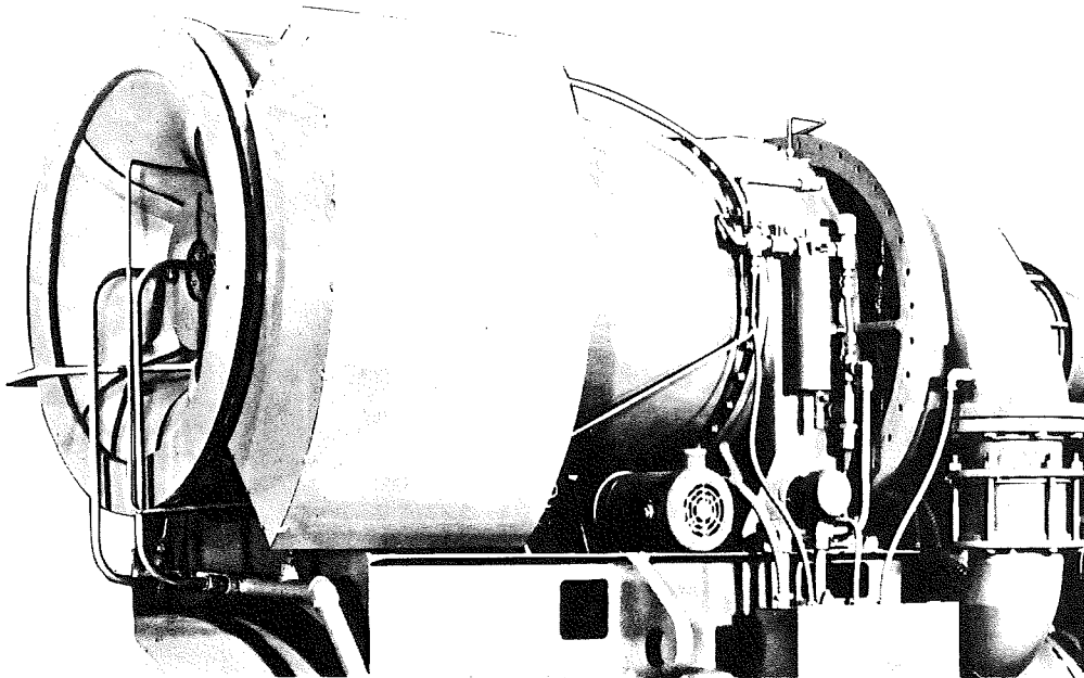
FIG. 1—HERMETIC—MOTOR COMPRESSOR, MODEL MKA
