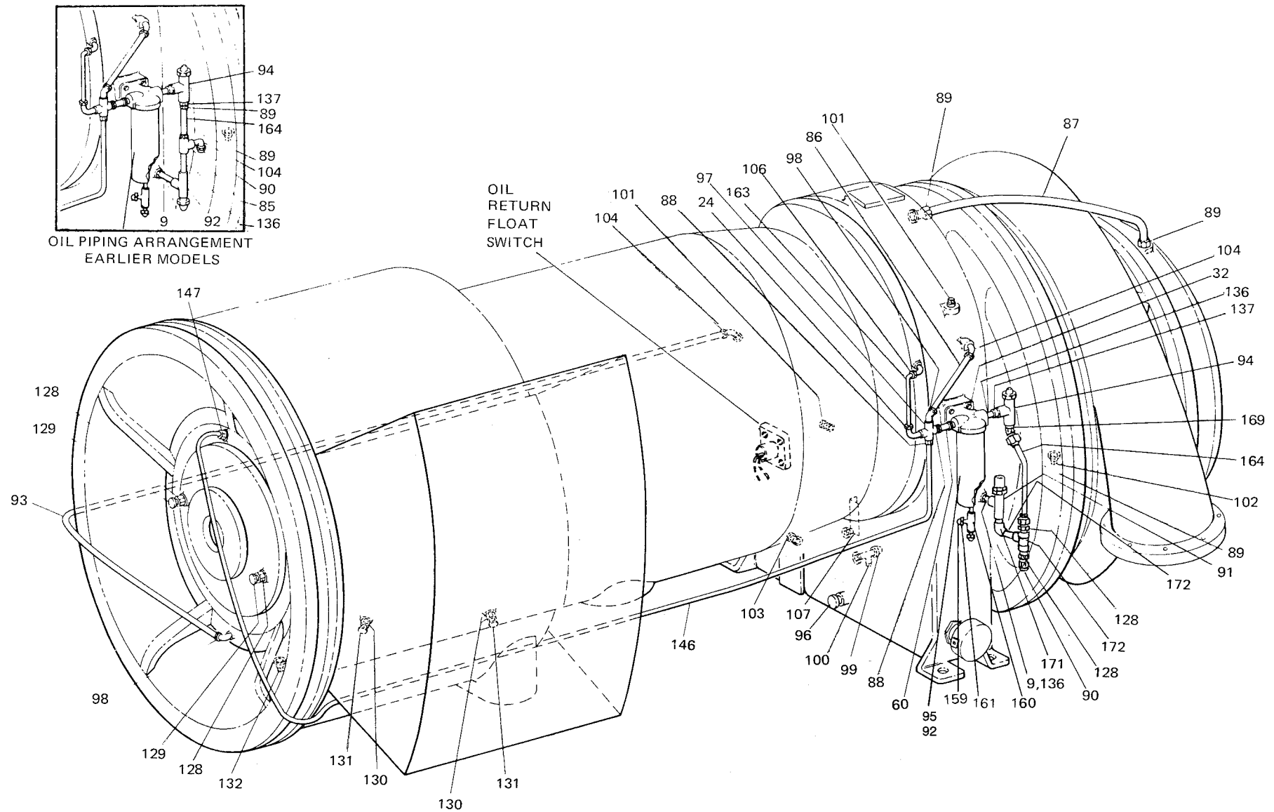
FIG. 3—MODEL MKA65 & MKA73 COMPRESSORS, EXTERIOR VIEW — PARTS LOCATION
