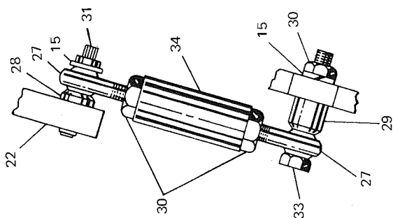
DETAIL "A" ADJUSTABLE ROD
