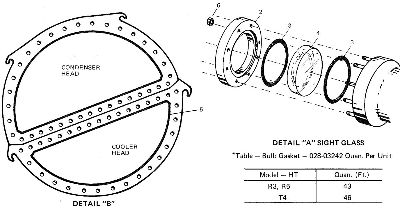
FIG. 1—COOLER—CONDENSER SHELL
