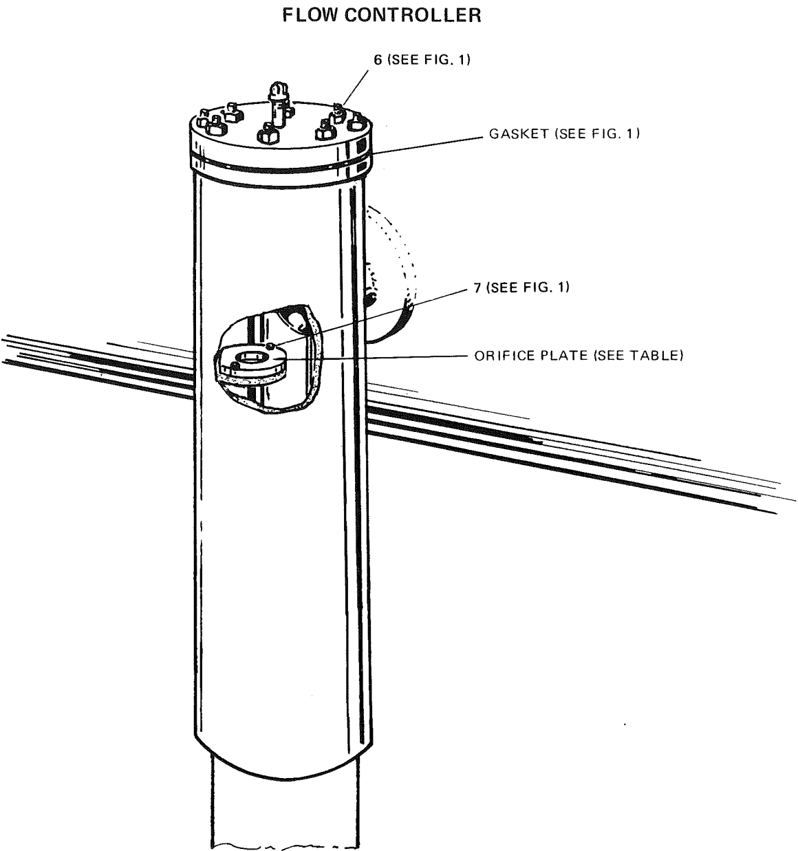
FIG. 2— FLOW CONTROLLER WITH ORIFICE PLATE
