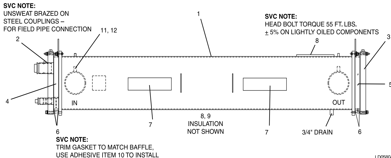
FIG. 1 –EVAPORATOR COMPONENTS
