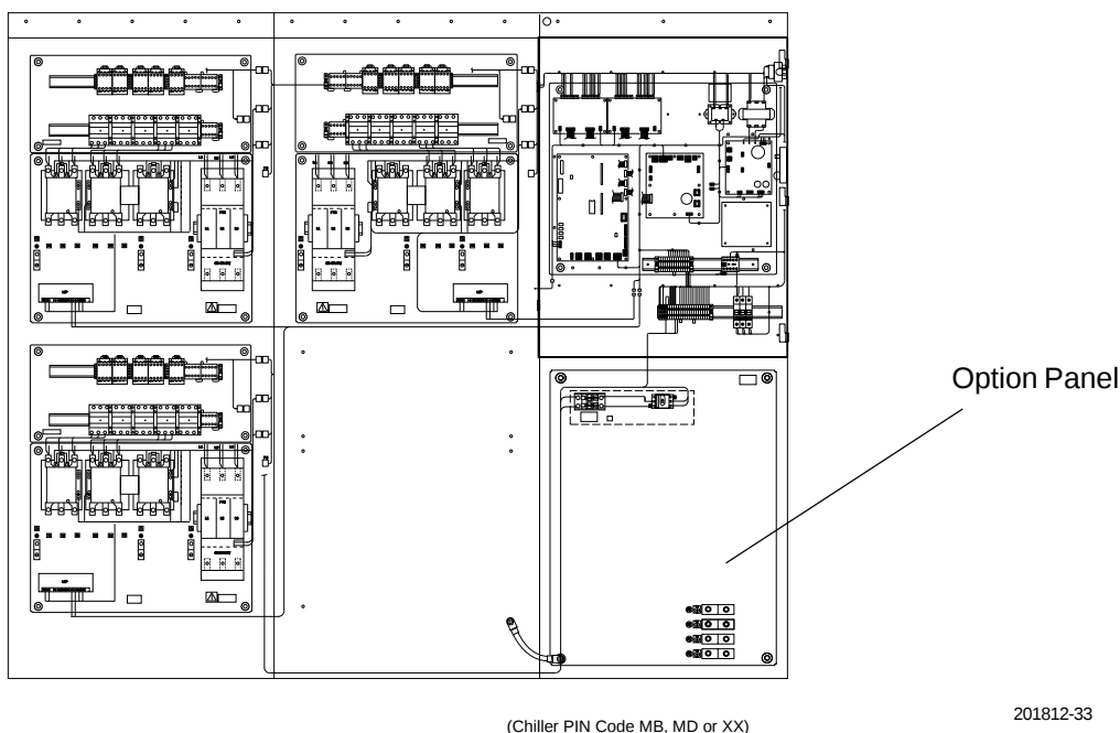
FIG. 26 – OPTION PANEL (3-COMPRESSOR UNITS)
