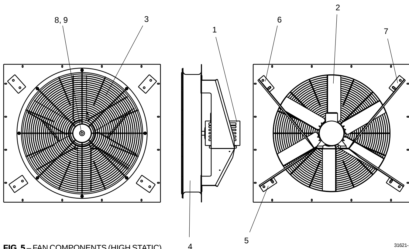
FIG. 5 – FAN COMPONENTS (HIGH STATIC)
