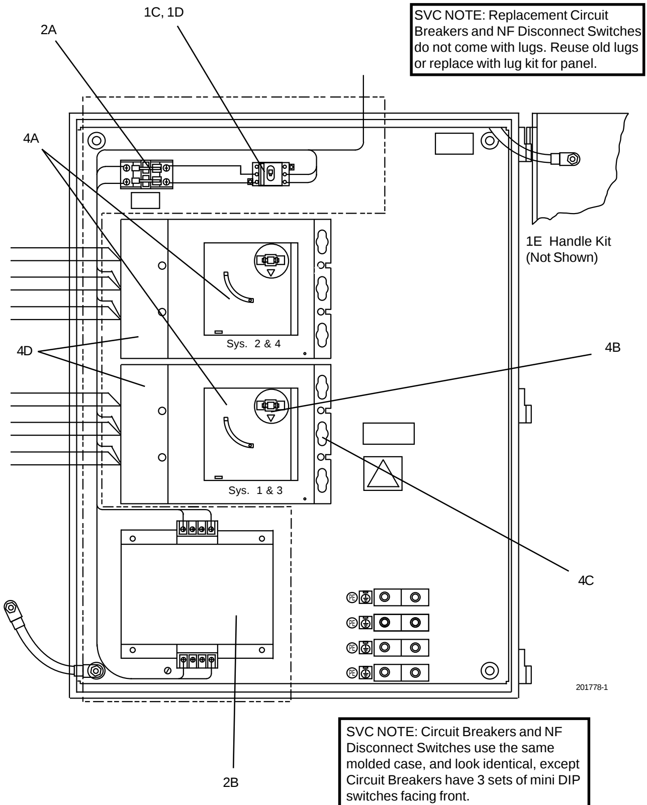
FIG. 27 – OPTION PANEL SHOWN WITH CIRCUIT BREAKER OR NON-FUSED DISCONNECT SWITCH (REF. TABLE 22, PAGES 51 AND 52)
