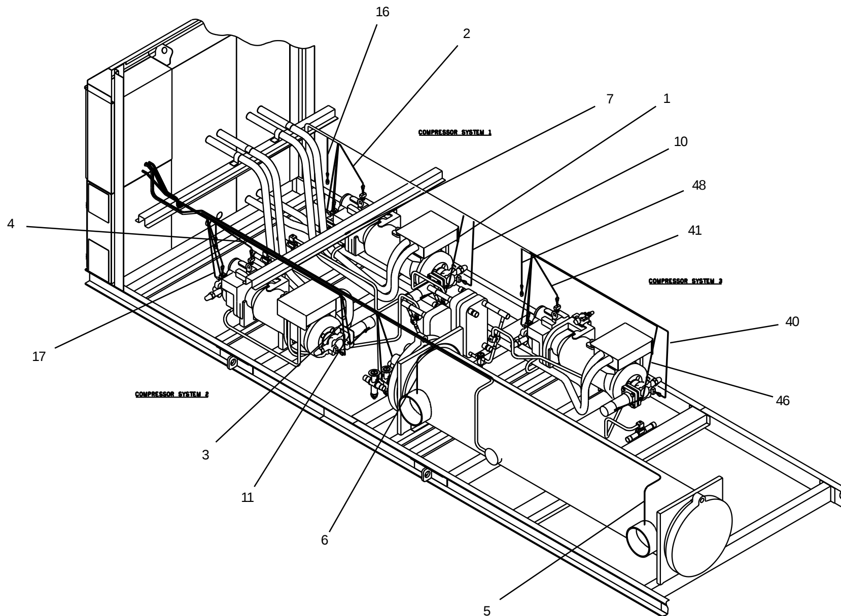
FIG. 19 – HARNESS LAYOUT (REF. TABLE 13, PAGE 29 AND 30)
