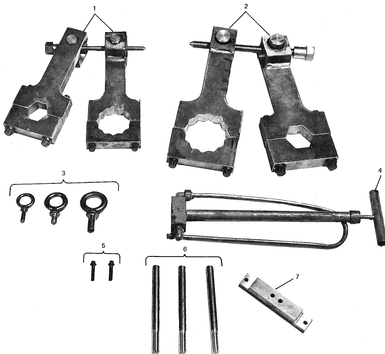
FIG. 14 — COMPRESSOR TOOLS FOR MODELS LKB65 &amp; LKB73
