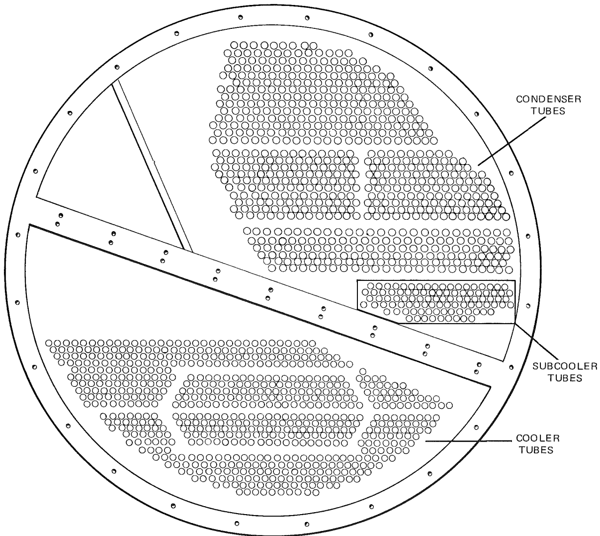
FIG. 3— COOLER AND CONDENSER TUBES—MOTOR END VIEW
