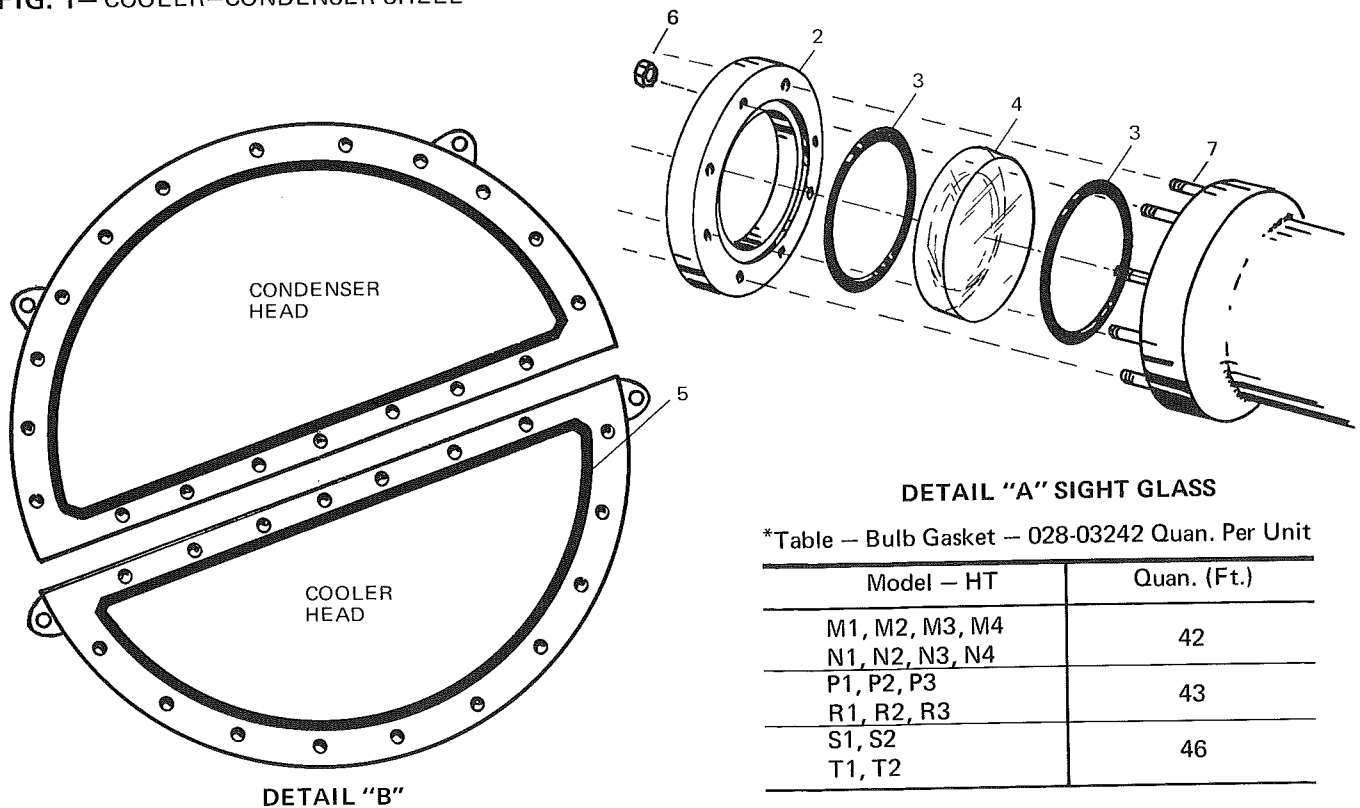
FIG. 1— COOLER—CONDENSER SHELL
