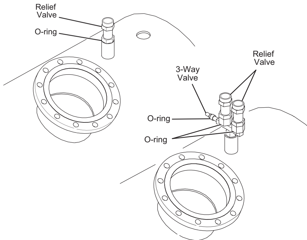
FIGURE 19 - EVAPORATOR RELIEF VALVE
