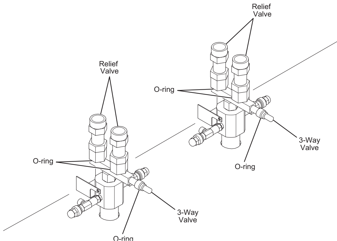
FIGURE 20 - CONDENSER RELIEF VALVE
