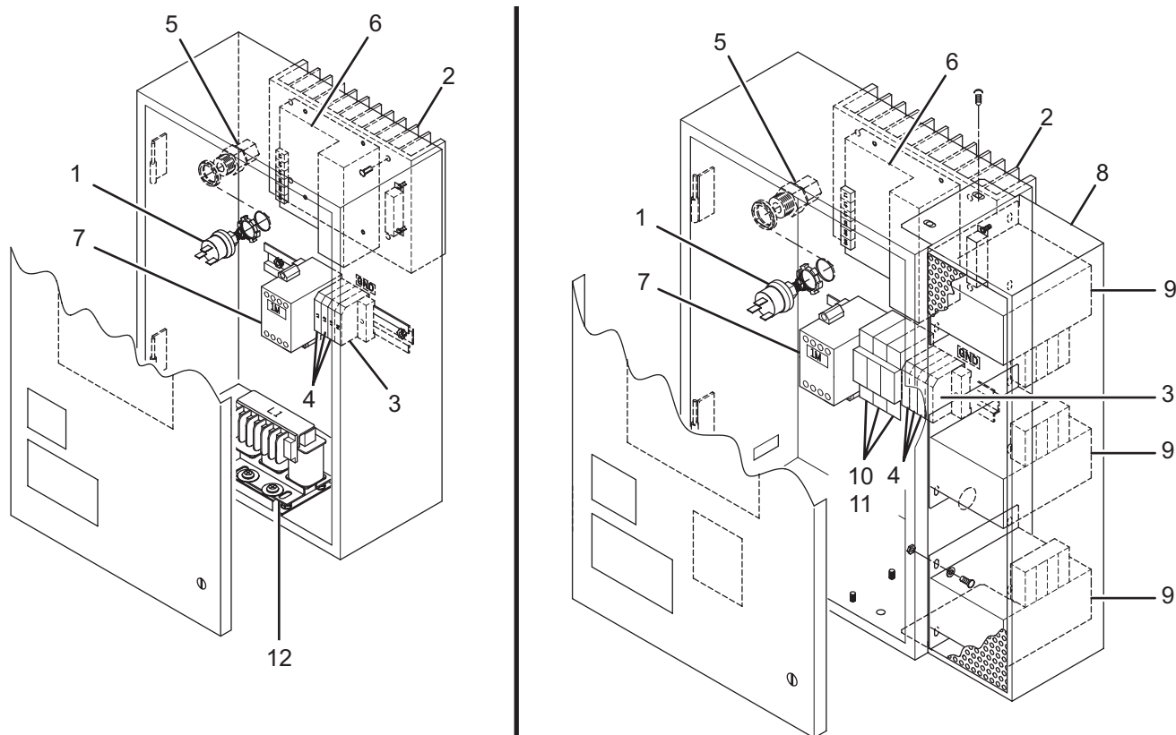
FIGURE 25 - VARIABLE SPEED OIL PUMP PANEL
