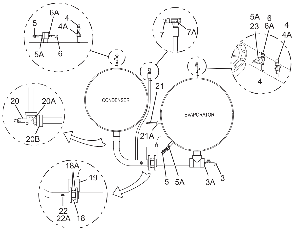
FIGURE 2 - UNIT COMPONENTS (P1-P6)
