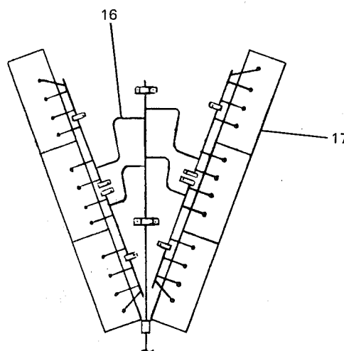
DETAIL "A" SYSTEM #1 & #2 - 4 ROW COILS TYP. 4
